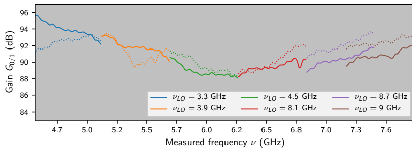
Figure II.10: Channel gains as functions of the measured frequency and the local oscillator frequency, solid lines correspond to one channel, dotted lines to the other. There are some jumps between different local oscillator due to the fact that gain depends on both input signal frequency and local oscillator frequency, see text. Moreover, the gain amplitude is compatible with the upper limit obtained by summed theoretical amplifications and attenuations along all the setup of 101 dB.
