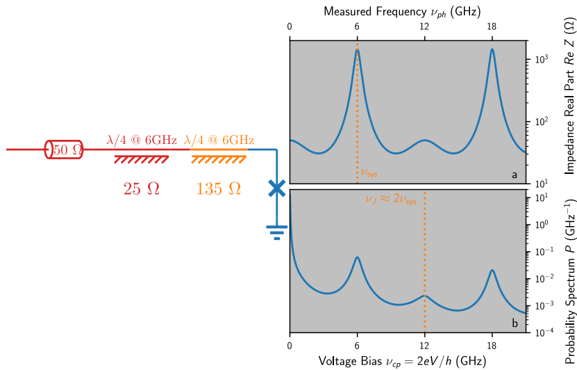
Figure V.2: Degenerate amplifier. Left scheme shows the two cascaded quarter-wave TL, the orange one mainly defines the resonator impedance while the red one together with the 50\Omega port defines the Q factor. The Josephson junction is in blue. Panel a shows the real part of the impedance as a function of the frequency, there are modes at (2n+1)\nu_{\text{sys}} , 6 GHz and 18 GHz peaks are visible. Panel b shows the corresponding P -function as a function of the voltage bias expressed in GHz. The peaks correspond to biases where Cooper pair tunnelling can happen. The zero bias peak is the supercurrent, the second and last correspond to first order processes with photons at respectively 6 GHz and 18 GHz, the third one at 12 GHz is a second order process where a Cooper pair gives two photons at 6 GHz. Orange dotted lines indicate the process used as amplifier.
