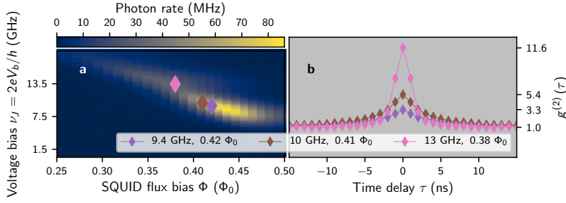
Figure IV.20: Super-bunching. Panel a is the photon rate as a function of the voltage bias and the flux bias. Diamond symbols indicate where g^{(2)} are measured. Panel b shows the g^{(2)} of panel a as functions of the time delay. The different curves show the g^{(2)} evolution when the photon rate is maximum at high voltage biases. Now g^{(2)}(0) \gg 2 , i.e. photons are super-bunched.
