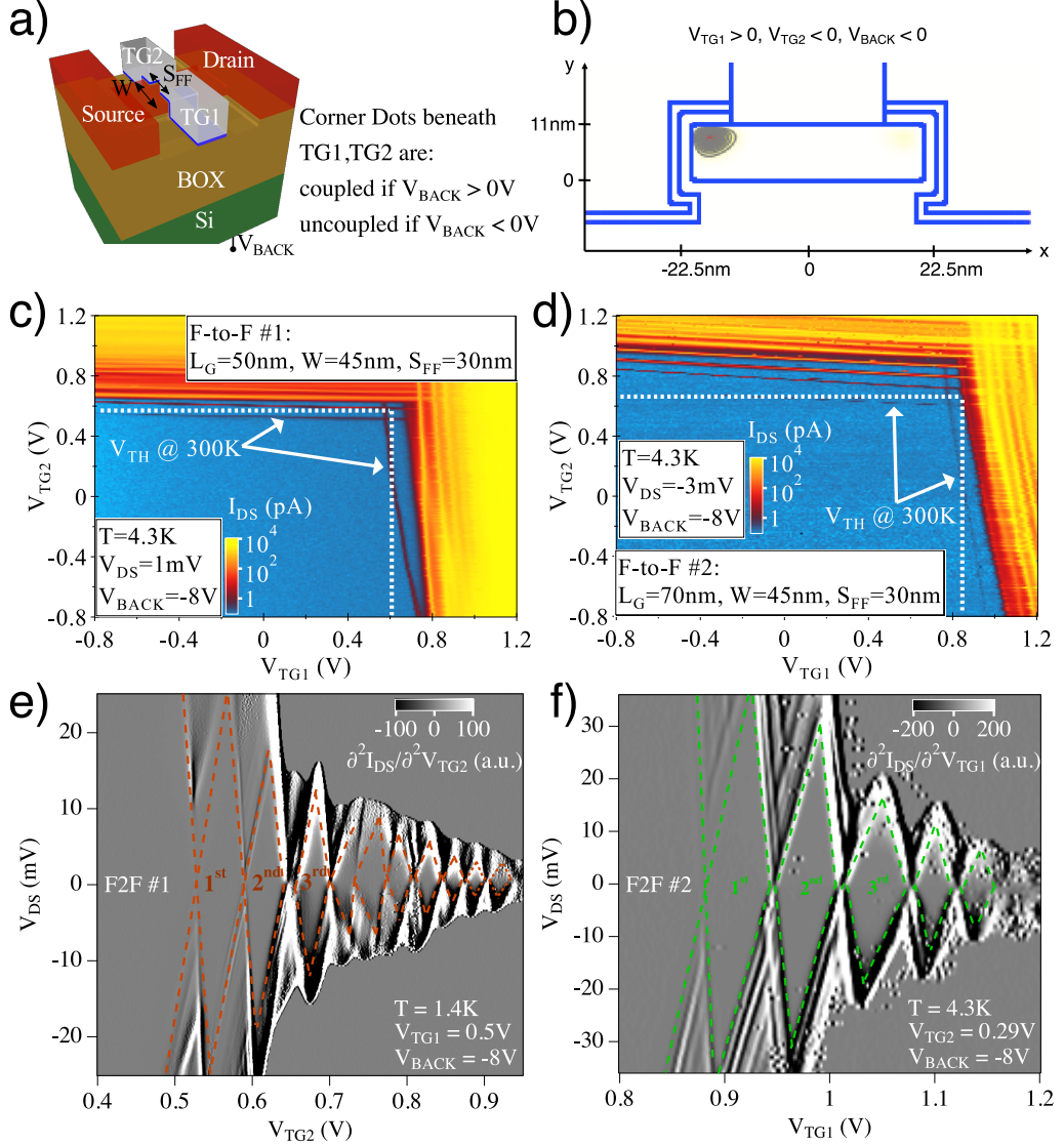
Figure 2.13: (a) A 3D sketch of n-type F-to-F device. (b) The wavefunction for a corner dot defined below G1 at V_{BACK} = -8 V obtained from realistic simulations accounting for the real device geometry. (c)-(d) Stability diagrams for two F-to-F devices with doped and undoped channel recorded at 4.3 K. Geometrical dimensions are given in the inserts. (e)-(f) Coulomb spectroscopy for the first electrons. V_{DS} - V_{TG1,2} are plotted as a function of \partial^2 I_{DS} / \partial^2 V_{TG2,1} .
