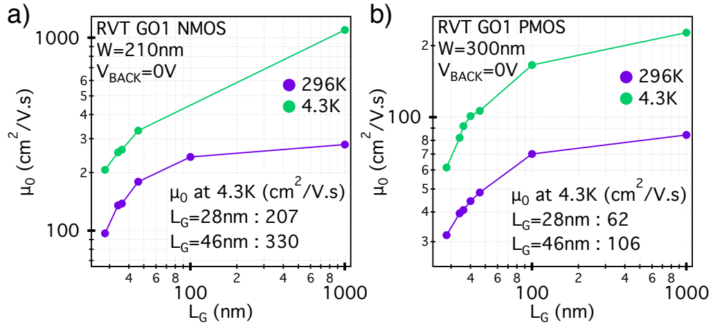
Figure 5.10: Low field \mu_0 mobilities extracted using the Y-function method for gate lengths between 28 nm and 1 \mu\text{m} . (a),(b) room temperature and 4.3 K low field mobilities for RVT transistors ( W_{\text{NMOS}} = 210\text{nm} , W_{\text{PMOS}} = 300\text{nm} ) for different L_G extracted for V_{N\text{-WELL}} = V_{P\text{-WELL}} = 0\text{V} .
