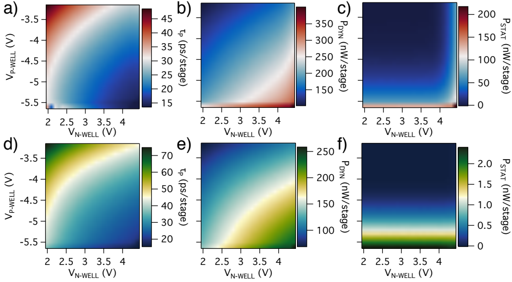
Figure 5.11: Performance of ROs at T = 4.3 \text{ K} and V_{DD} = 0.5 \text{ V} in terms of \tau_P , P_{DYN} , and P_{STAT} for the same forward body biasing ranges. (a - c) L_G = 28 \text{ nm} . (d - f) L_G = 46 \text{ nm} . For both ROs W_{NMOS} = 420 \text{ nm} and W_{PMOS} = 600 \text{ nm} .
