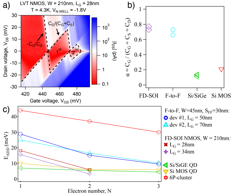
Figure 6.5: (a) Typical Coulomb diamonds observed in short-channel NMOS. (b),(c) Benchmarking of FD-SOI quantum dots with respect to the Corner Dots observed in F-to-F devices (see Chapter 2), Si/SiGe QDs [56], Si MOS QDs structures with two levels of gates [199], and six-phosphorus-based QDs [111].
