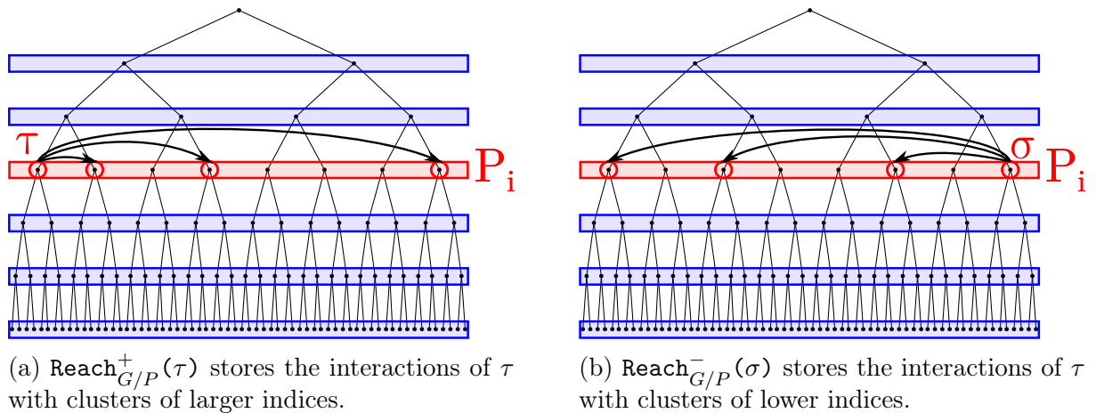
Figure 2.31: Partition P_i in a cluster tree, of which we have highlighted the different levels by blue horizontal lines. The partition is highlighted in red. This representation assumes that clusters are ordered from left to right.
