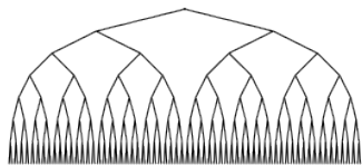
Figure 1.10: Tree based on median bisection.
