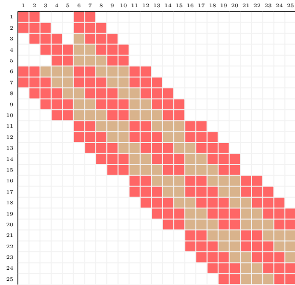
(b) Factorized matrix ( LU ).
