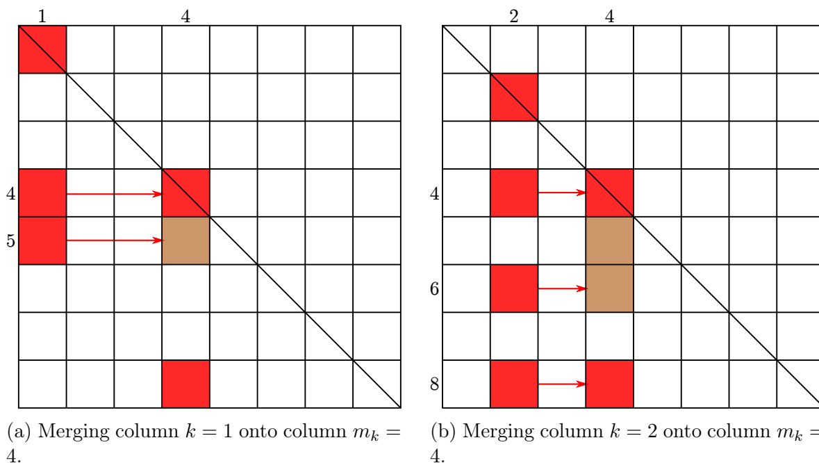
Figure 1.34: Right-looking contributions of column 1 and 2 on column 4 from example Fig. 1.32c.
