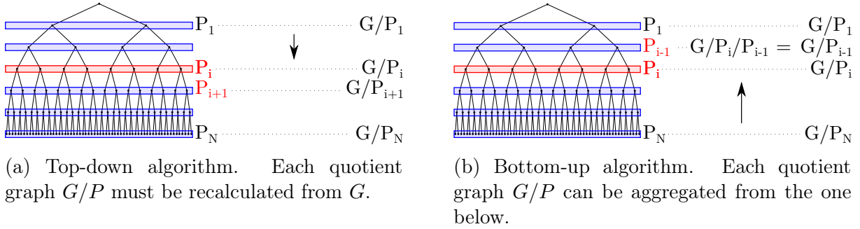
Figure 2.32: The order of the computation of partitions for the Hierarchical Symbolic Factorization is given by the direction of the arrow.
