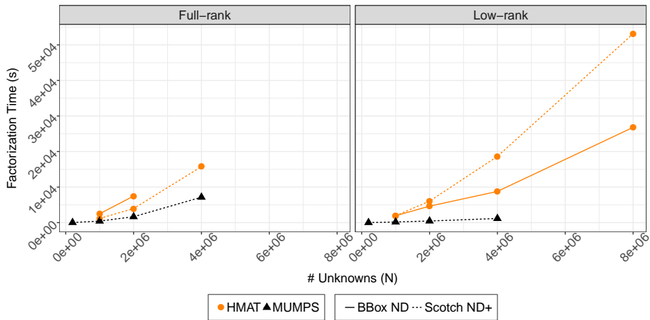
(b) Numerical factorization time.
