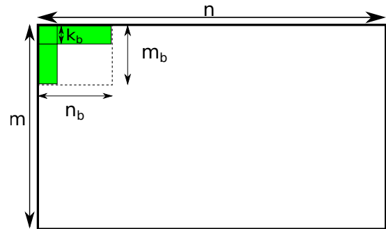
Figure 2.19: Fit \mathcal{R}k format: \mathcal{R}k compression on a Fit Full block.
