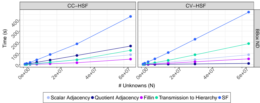
(b) Detail of the symbolic factorization step. The total computation time SF is the sum of all other steps.
