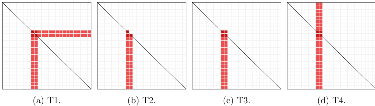
Figure 1.29: Possible types of unsymmetric supernodes.
