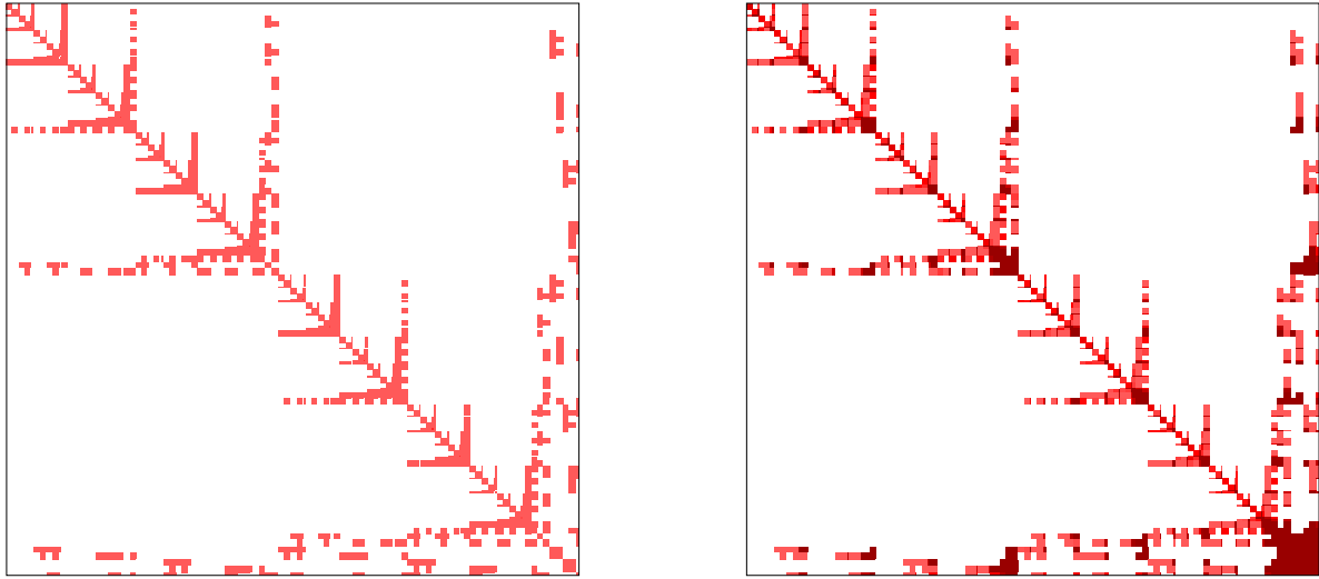
(a) Sparse matrix before factorization, with nested dissection reordering.
