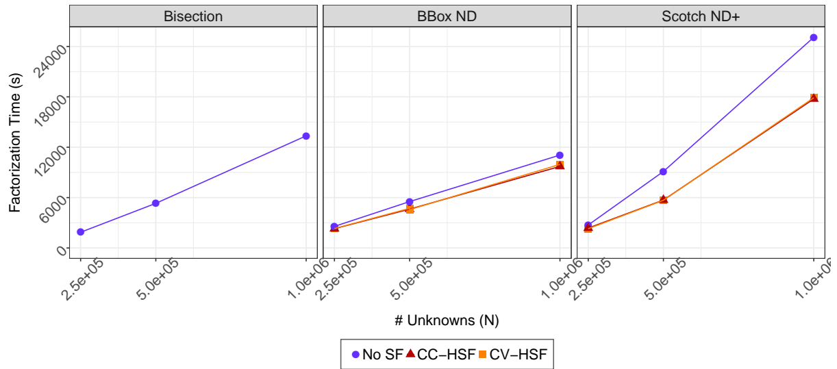
(a) Factorization time.
