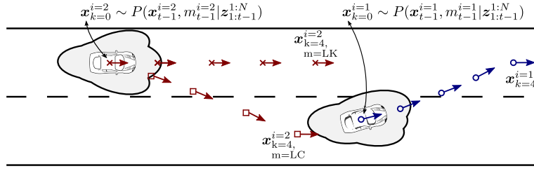
Fig. 6.2.: Schematic showing the anticipatory, model-based maneuver forecasting approach.
