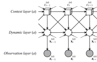
(b) Slice of the DBN proposed by Agamennoni et al. corresponding to a single traffic participant. Dotted lines connect to slices of surrounding vehicles. [Image credit: (Agamennoni et al., 2012)].
