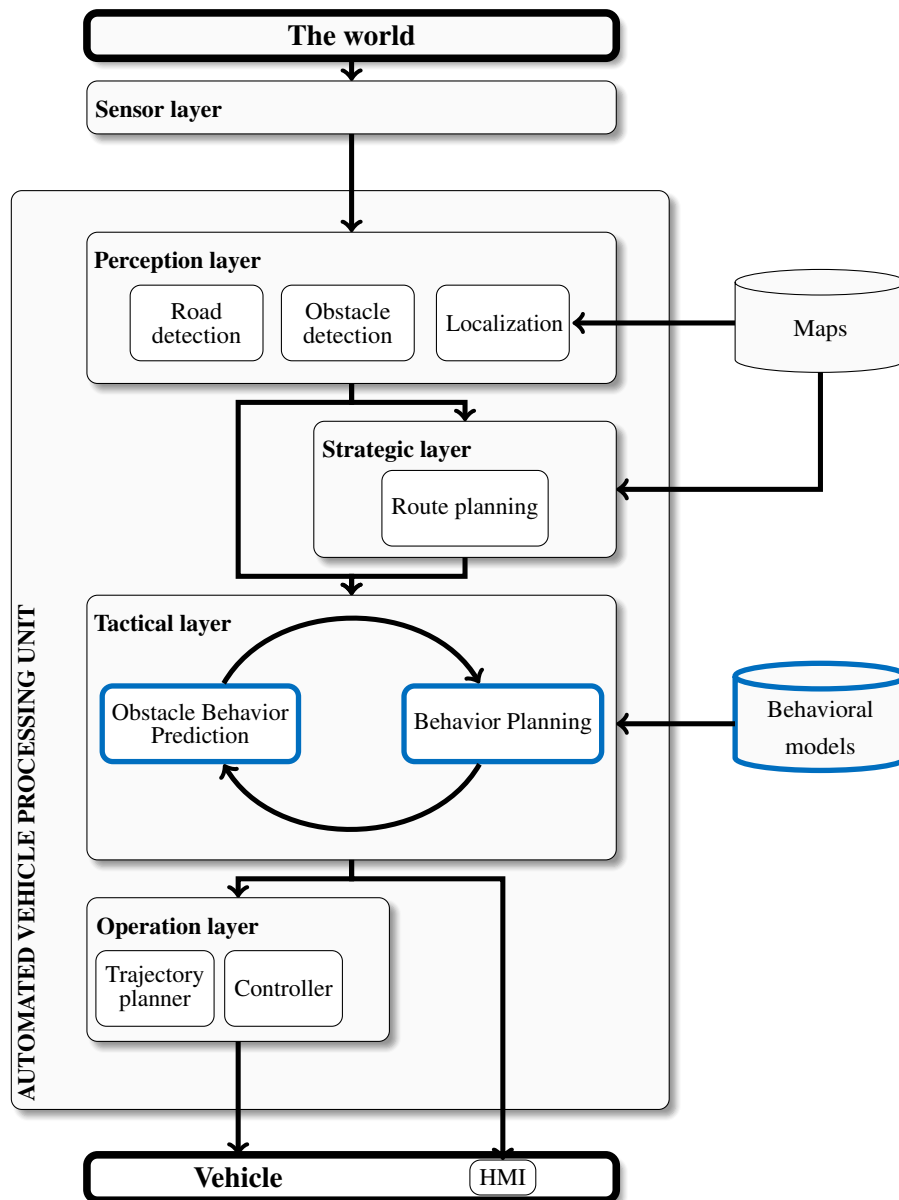
Fig. 1.2.: Simplified block-diagram of the architecture of a fully or highly automated vehicle. The blocks with thicker blue edges are the focus of this thesis.
