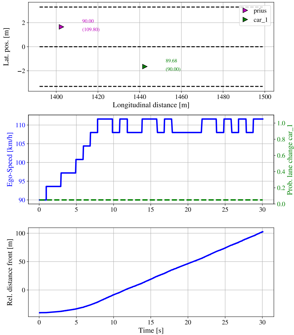
Fig. 7.12.: In this overtake scenario, the POMDP planner selects the acceleration commands for the ego-vehicle. The obstacle in lane 1 is never estimated to be executing a lane change maneuver.
