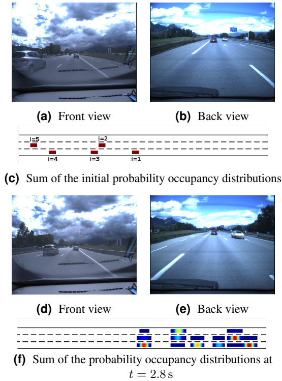
Fig. 5.4.: Typical 3-lane highway scene ( t = 2.8 s). Our approach predicted a lane change for vehicle i = 4 , that was advancing fast in the middle lane.
