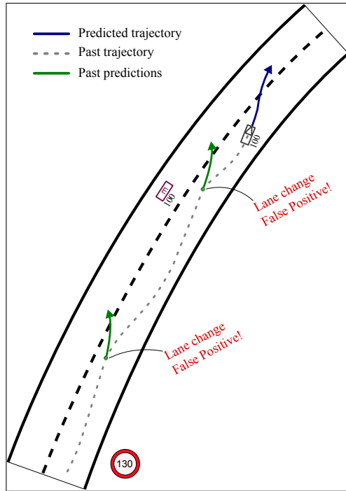
(b) Vehicle trajectories in the real world can produce a high number of false positives in prediction approaches that rely exclusively on dynamic evidence.
