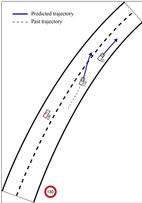
(a) Short-term prediction of behavior leveraging dynamic evidence and situation understanding. Both the dynamics and the relative distance and velocity of the target with respect to the leading vehicle indicate a potential lane change.
