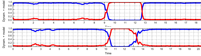
Fig. 6.5.: Filtering results obtained with an incorrect model prediction for the scenes shown in Figure 6.3c (top), and Figure 6.4c (bottom). The model prediction is manually set to P(m_t = \text{LK}) = 0.8 and P(m_t = \text{LC}) = 0.2 throughout the whole scene. Despite this, the lane change maneuvers are still detected.
