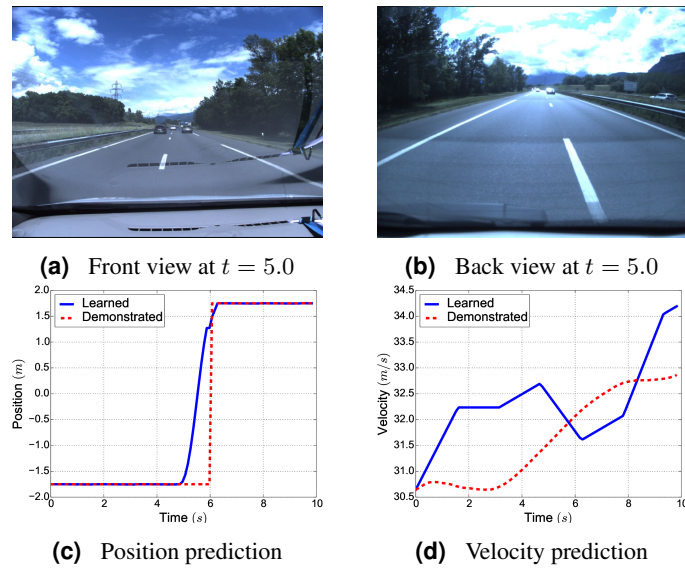
Fig. 4.6.: Prediction of overtaking behavior.
