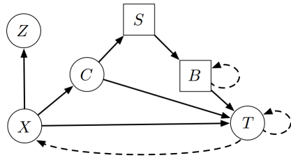
(a) Temporal slice of the DBN proposed by Gindele et al. Dashed lines: temporal dependencies. Solid lines: causal dependencies. Square nodes: discrete. [Image credit: (Gindele et al., 2010)]
