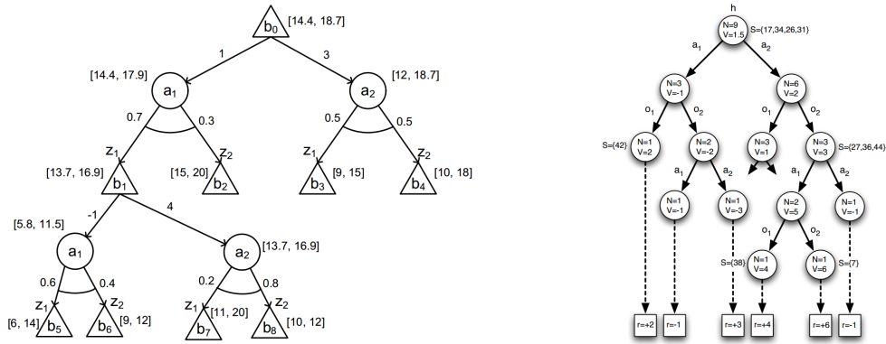
(a) AND-OR search tree for a POMDP with 2 actions and 2 observations. The belief states correspond to OR nodes and the actions to AND nodes. The values between brackets are lower and upper bounds on the value [Image credit: (Ross et al., 2008)]. (b) POMCP search tree for a POMDP with 2 actions, 2 observations, 50 states and no intermediate rewards. The value (V) and number of visits (N) is maintained for each history [Image credit: (Silver and Veness, 2010)].
