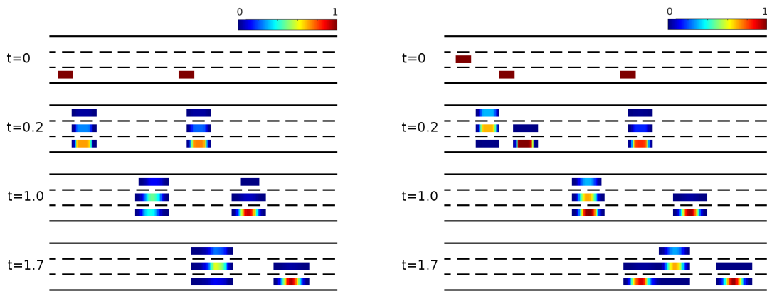
(a) Simulation of the traffic scene presented in Figure 5.1a. The model predicts an overtaking maneuver from the trailing vehicle.
