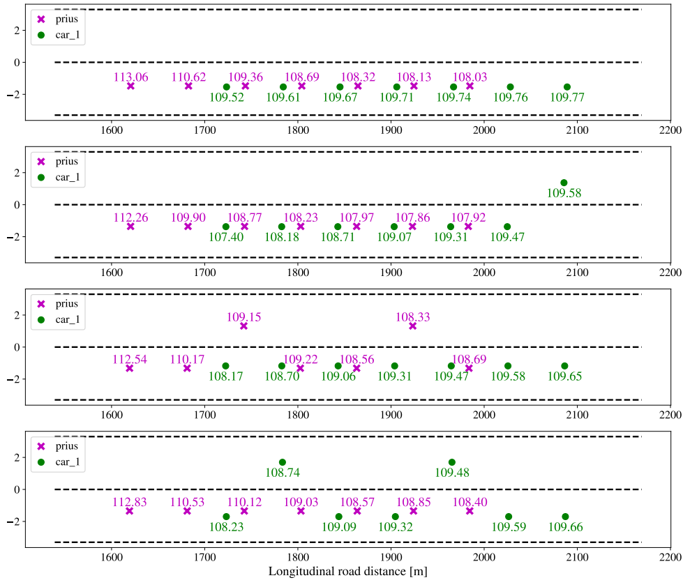
(b) Example of possible rollouts. For each vehicle, the rollout is illustrated as a sequence of markers showing its states at the different rollout steps. A label showing the velocity of the vehicle is also shown next to the markers. In the proposed rollout policy, a maneuver is exponentially more likely when it leads to states with a lower cost. Given that in this traffic scene the difference in cost between driving in the right or left lane is not large, sometimes a lane change maneuver is sampled.
