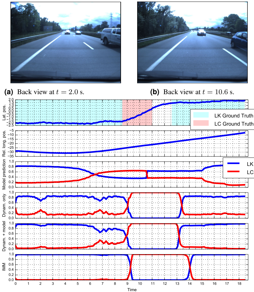
(c) Filtering results obtained for scene 3. The results of the proposed approach that leverages dynamic evidence and model-based prediction are shown in the penultimate row. Compared to an IMM filter (last row), we can observe a slightly quicker detection both of the beginning and of the end of the lane change maneuver of the target.
