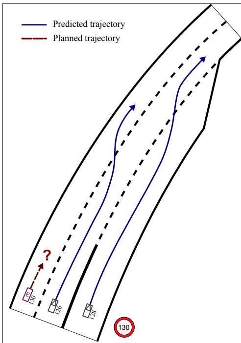
(c) Predicting the long-term development of highway traffic scenes requires a degree of situation understanding and an appropriate model of the interactions between traffic participants.
