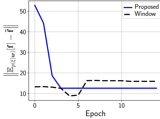
Fig. 4.3.: Convergence of the different learning algorithms considered.
