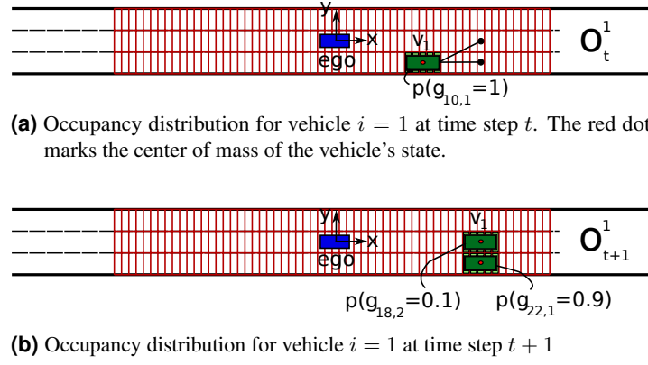
Fig. 5.2.: Evolution of the occupancy distribution of a vehicle over the cells of grid \mathcal{G} in one time step. The occupancy probabilities at time step t + 1 will depend on the available actions in the previous time step.
