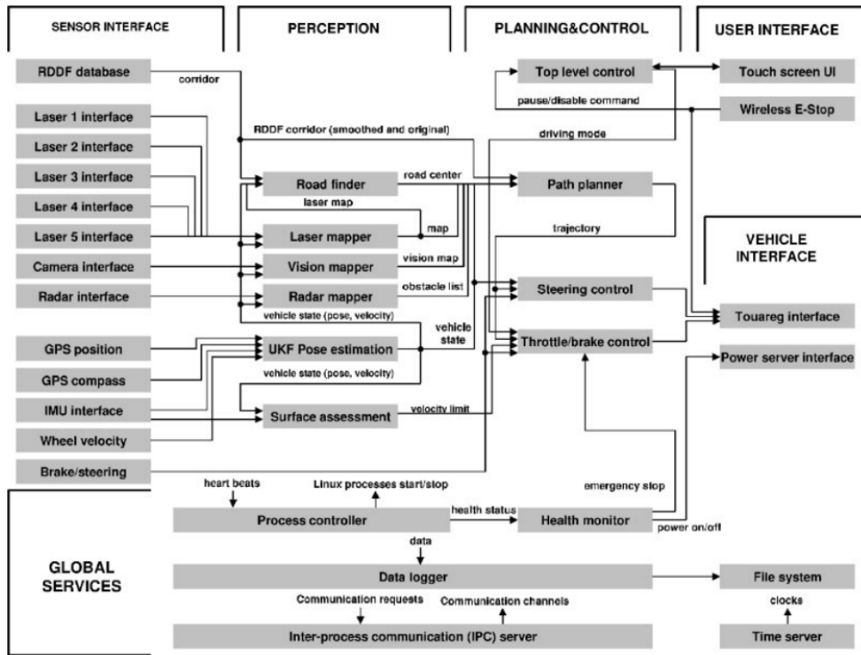
Fig. 3.3.: Software architecture of Stanley , the 2005 DARPA Grand Challenge winner [Image credit: (Thrun et al., 2006)]
