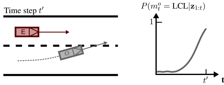
Fig. 7.2.: Example that motivates the proposed sampling procedure. In this scene, the model-based maneuver prediction from Equation 6.7 would predict with high probability a lane keeping maneuver for obstacle o given the presence of the ego-vehicle in the adjacent lane. However, the maneuver of this obstacle had been estimated to be a lane change based on its dynamics (graph on the right) and therefore this situation should be adequately represented in the history tree. Relying exclusively on ideal driver models for sampling during the tree construction can lead to an incorrect estimation of the consequences of an action.
