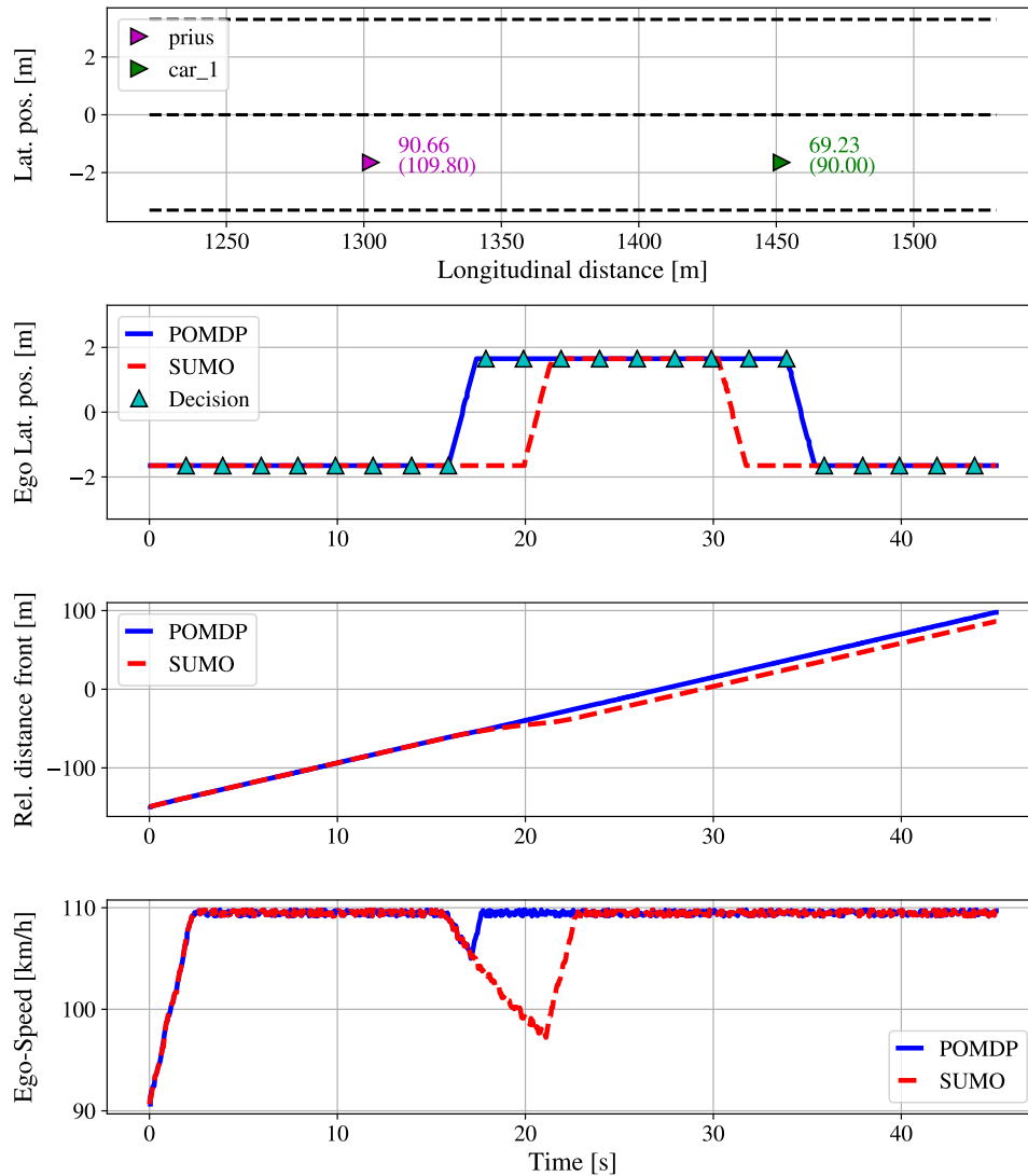
Fig. 7.8.: Planning results obtained for an easy highway overtake scenario. The POMDP planner recognizes the advantage in doing a lane change to avoid deviating too much from the desired speed.
