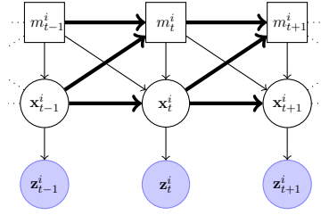
Fig. 6.1.: Graphical model representation of the proposed switching state-space model. A slice of the Bayesian network corresponding to vehicle i is shown. Bold arrows indicate multi-vehicle dependencies.
