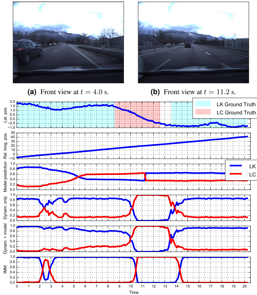
(c) Filtering results obtained for scene 7. The results of the proposed approach that leverages dynamic evidence and model-based prediction are shown in the penultimate row. Compared to an IMM filter (last row), we can observe an increased robustness against false positive lane change detections ( t = 2.5 s) and a lower latency in the detection of actual lane changes ( t = 10 s).
