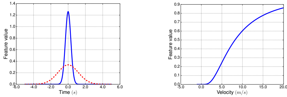
(a) Gaussians used to parameterize the time-to-collision and time-headway features (b) Function used to parameterize the feature associated with the deviation from desired velocity.
