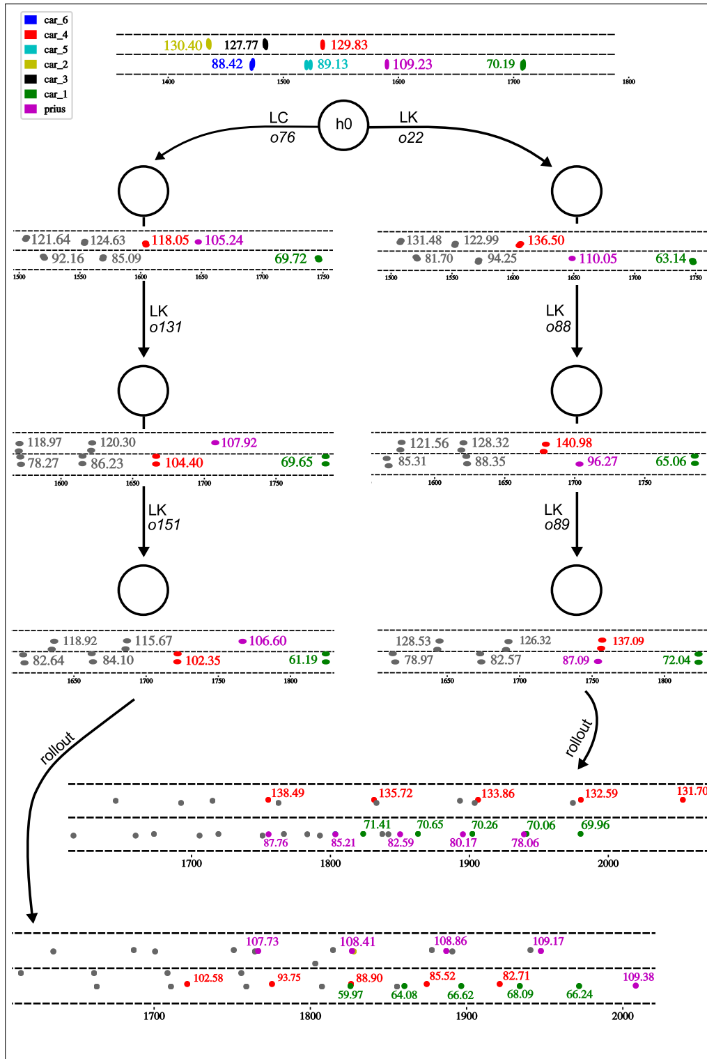
Fig. 7.11.: Exemplary tree simulations for the third traffic scene of task 1. Only the three most relevant vehicles in the scene are depicted in color. The POMDP’s time step is 2 seconds. A simulation in which three lane keeping actions are selected shows the ego-vehicle (prius) stuck on lane 1 behind ‘car_1’ (right-hand side of the figure). In contrast, if a lane change action is selected followed by two lane keeping actions, the ego-vehicle is predicted to overtake ‘car_1’ and merge in front of it.
