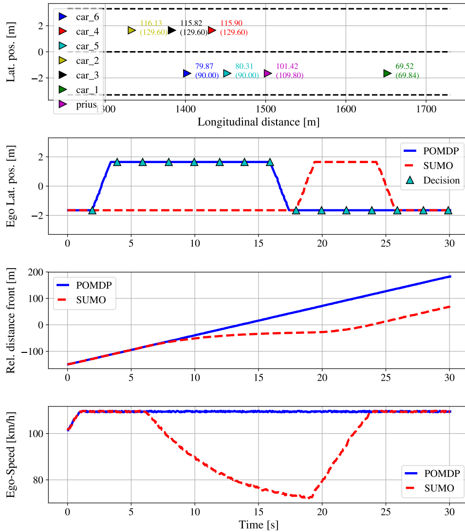
Fig. 7.10.: Planning results obtained for an overtake scenario where the long-term development of the scene needs to be considered. SUMO’s reactive model leads the ego-vehicle to get stuck behind obstacle ‘car_1’ and deviating significantly from its desired velocity. In contrast, the proposed POMDP planner considers the long-term consequences of any decision and decides to switch lanes at around t = 2s , avoiding thus to get stuck.
