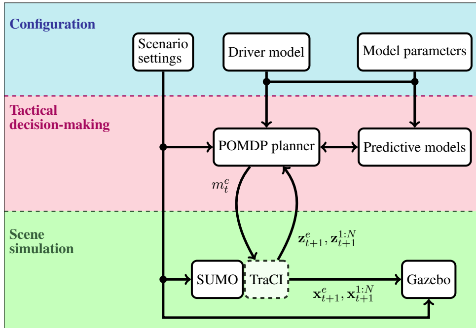
Fig. 7.5.: Architecture of our highway simulation platform. The user can configure the settings of the traffic scene (number of lanes and connectivity, number of obstacles and their preferences, speed limits, etc.) and the parameters of the driver model used in the POMDP and predictive models. In our case, this model is learned from demonstrated driving data as shown in chapter 4. At each time step, our POMDP planner selects a maneuver for the ego-vehicle and then SUMO simulates the state transitions for all vehicles. The resulting physical states of all vehicles are passed to Gazebo for visualization. The POMDP planner receives a noisy observation of the physical states and then proceeds to search for the next maneuver to execute.
