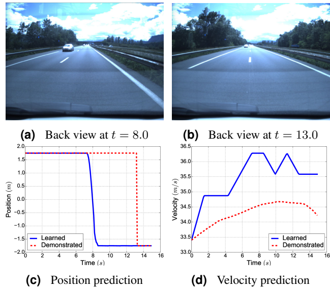
Fig. 4.5.: Prediction of behavior for a right-merge scene.
