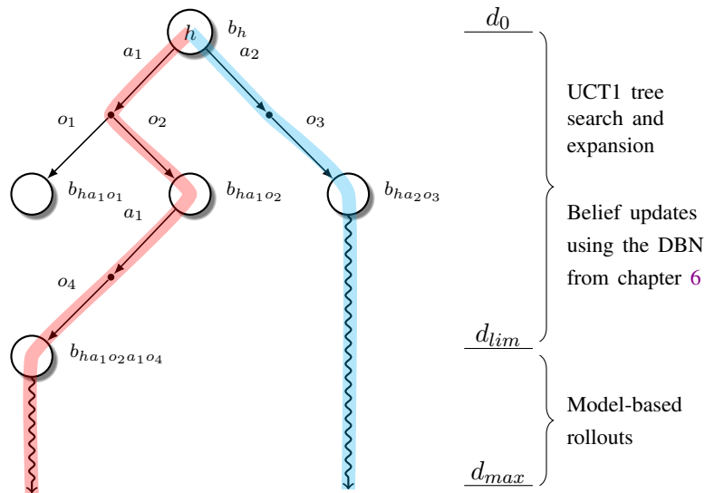
Fig. 7.1.: Search tree of histories. Each history h , has an associated parametric belief b_h . The beliefs are updated using the DBN model from chapter 6. The subscripts in the actions and observations indicate particular instantiations rather than time. The depth of the tree is truncated to d_{lim} . The model-based rollouts are executed until d_{max} . In this chapter, we will refer to the circular tree nodes as belief nodes, and to the black dots as action nodes. The red and cyan transparent lines indicate exemplary simulations executed in the tree.
