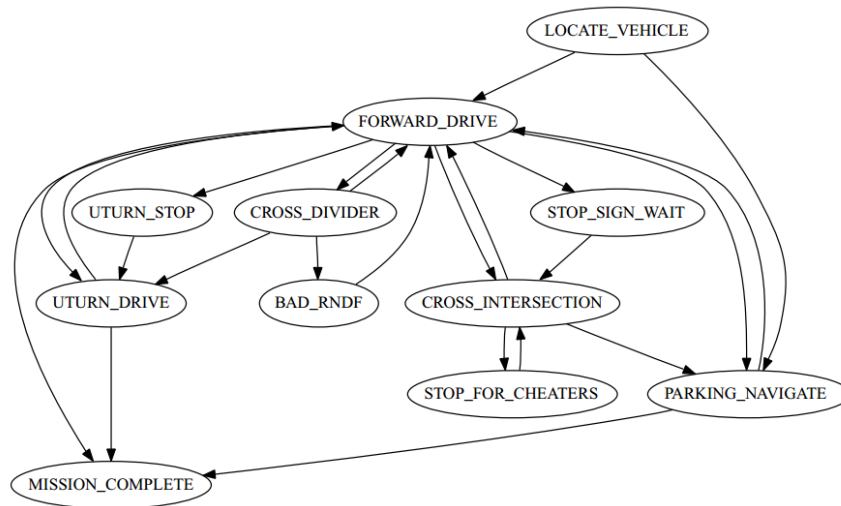
Fig. 3.4.: Finite State Machine for the tactical decision-making of Junior, second-ranked vehicle in the 2007 DARPA Urban Challenge [Image credit: (Montemerlo et al., 2009)].
