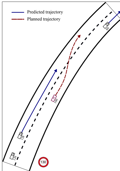
(d) The long-term planning of maneuvers for the EV is enabled by the ability to predict the long-term consequences of each plan.
