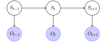
Fig. 2.1.: Graphical model representation of a state-space model. Shaded nodes indicate observed variables.
