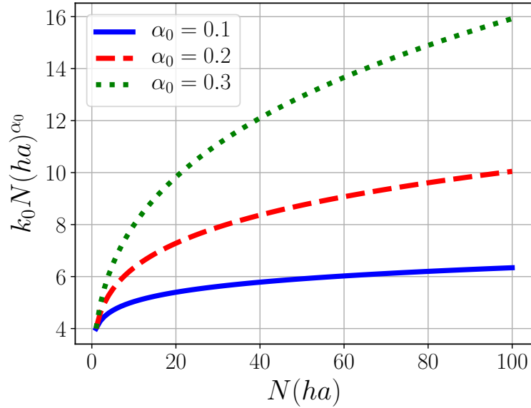
Fig. 7.4.: Progressive widening: Number of observations allowed per action node as a function of the number of visits to the node. The results are shown for k_0 = 4 and different settings of the parameter \alpha_0 . In practice, the observation limit is rounded down to the nearest integer.
