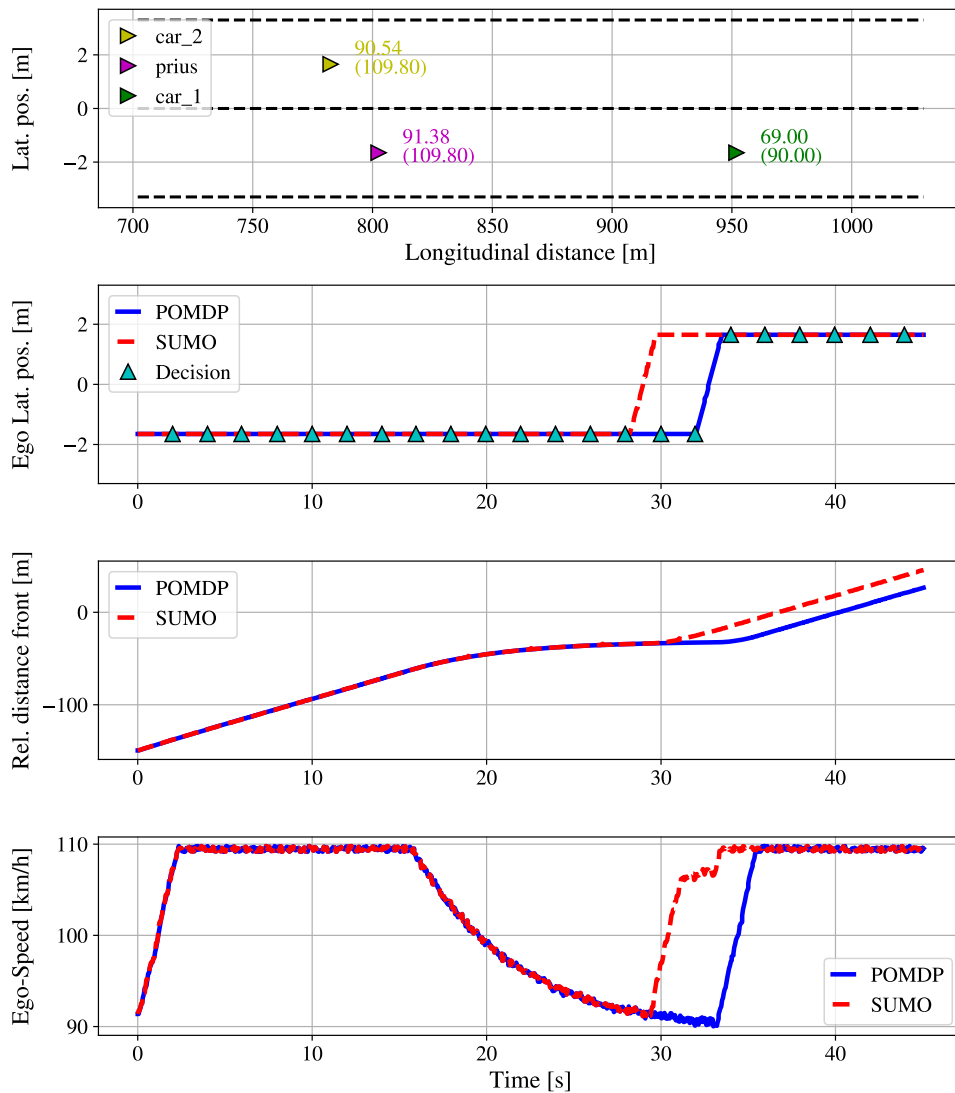
Fig. 7.9.: Planning results obtained for a delayed overtake scenario. As the left lane is occupied, both SUMO and our POMDP planner decelerate the ego-vehicle to match the velocity of the slow leading vehicle.
