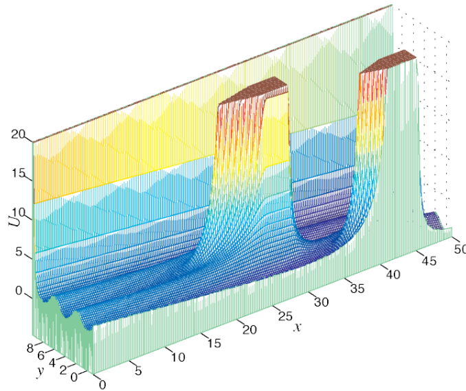
Fig. 3.1.: Example of potential field for a 3-lane highway with 2 dynamic obstacles [Image credit: (Wolf and Burdick, 2008)]
