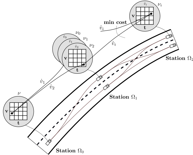
Fig. 4.1.: Structure of the spatiotemporal state lattice. Road-aligned states are sampled at regular longitudinal intervals on each lane and connected with feasible paths using parametric optimal control. The spatiotemporal planner searches for the best trajectories in the lattice and keeps the problem tractable by pruning the search space (McNaughton et al., 2011).
