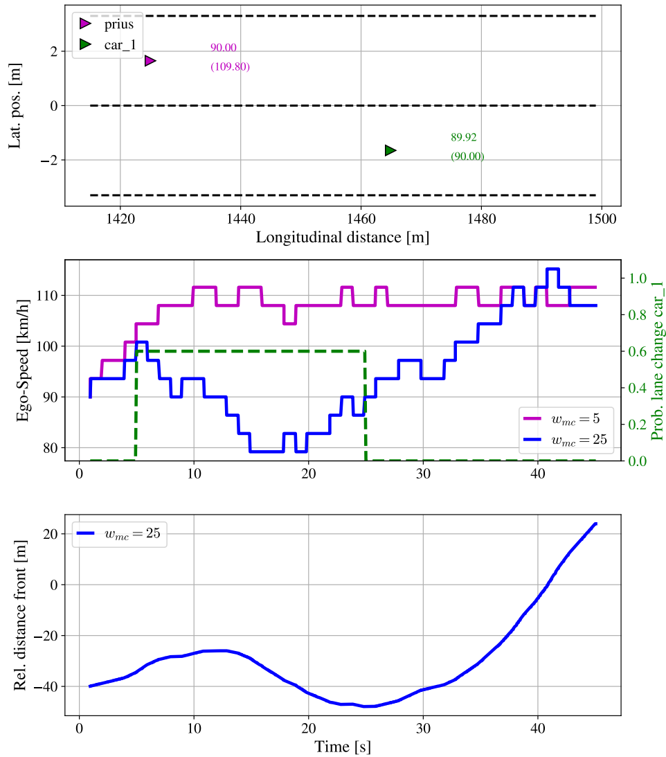
Fig. 7.13.: In this overtake scenario, the POMDP planner selects the acceleration commands for the ego-vehicle. The obstacle in lane 1 is estimated to be executing a lane change maneuver with probability 0.6 between seconds 5 and 25. As a response, the planner (with w_{mc} = 25 ) slows down the ego-vehicle to allow the lane change and avoid falling into high-cost states. Once it is clear that the obstacle will remain on its current lane, the planner (with w_{mc} = 25 ) accelerates to reach the desired speed of the ego-vehicle. However, if w_{mc} = 5 the danger is ignored and the ego-vehicle simply accelerates to overtake the obstacle.
