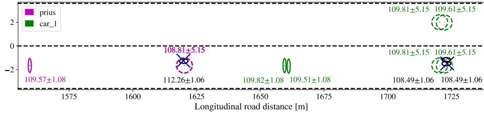
(a) Belief update step after selecting a LK maneuver for the ego-vehicle (prius). The predictive distributions are illustrated by the dashed 2\sigma error ellipses. An observation is sampled from the predictive distributions (blue crosses indicate the sampled physical states) and used to perform the KF measurement step. The expanded posterior distribution for the obstacle is collapsed back to two components. The x-y components of the final belief are illustrated by the black ellipses.
