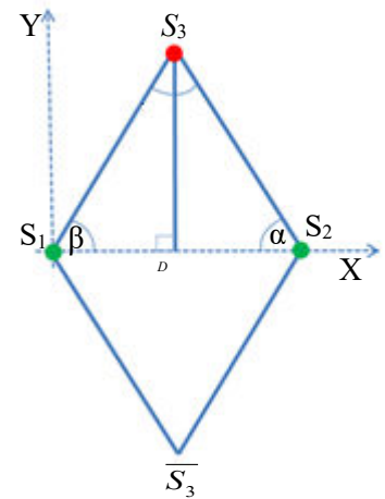
Figure 2.21: Angulation example.
