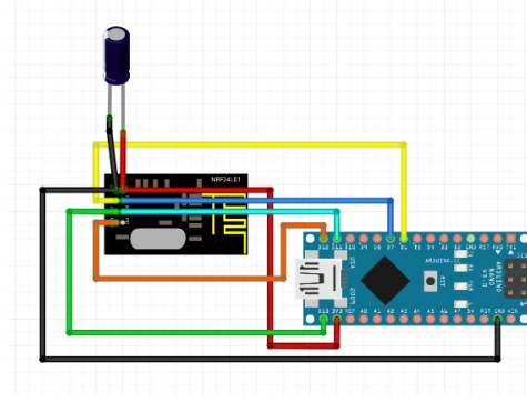
Figure 3.36: Ground sensor nodes wiring diagram.
