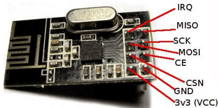
Figure E.2: nRF24L01 Transceiver
