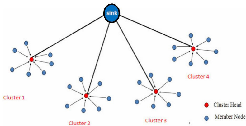
Figure 3.1: LEACH clustering.
