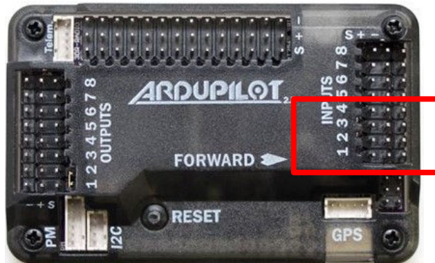
Figure 5.15: APM 2.6 autopilot.
