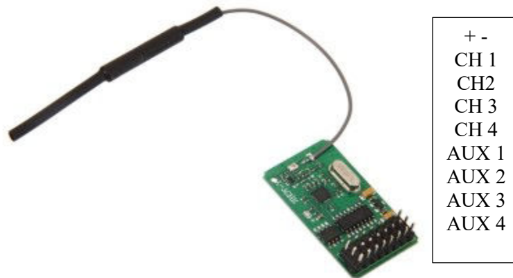
Figure 5.14: Radio receiver for UAV.
