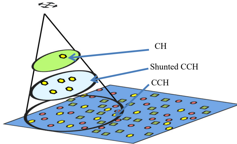
Figure 1.2: Dynamic clustering.
