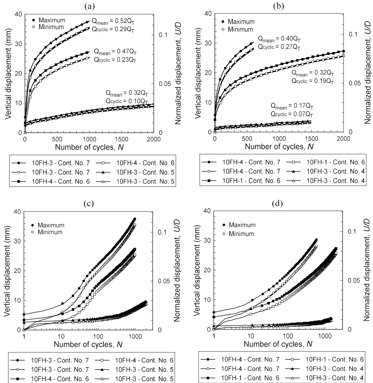
Figure 68. Maximum and minimum values of vertical displacements with number of cycles in (a) and (b) linear scale; and (c) and (d) log scale.
