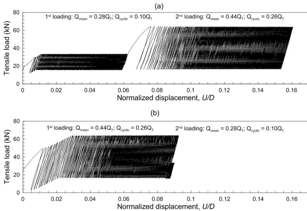
Figure 87. Load-displacement responses of tests with sequence of different cyclic loadings: (a) test 10FH-5 and (b) test 10FH-6, both in Cont. No. 6 (prototype values).
