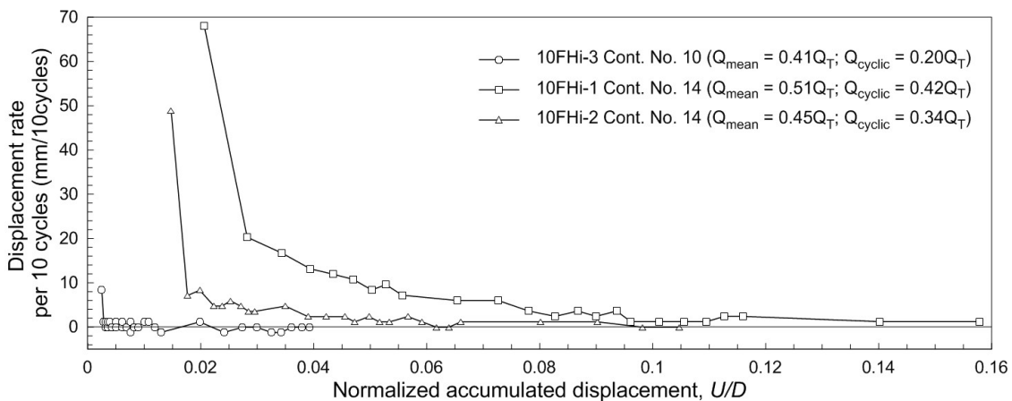
Figure 71. Displacement accumulation rates versus accumulated vertical displacements in cyclic tests performed with 10FHi model, in prototype values.
