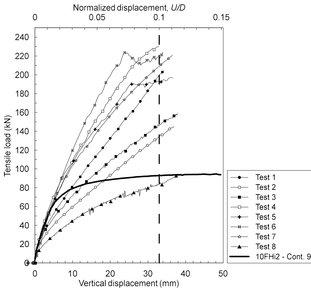
Figure 101. Comparison between numerical and experimental pre-cyclic monotonic responses.
