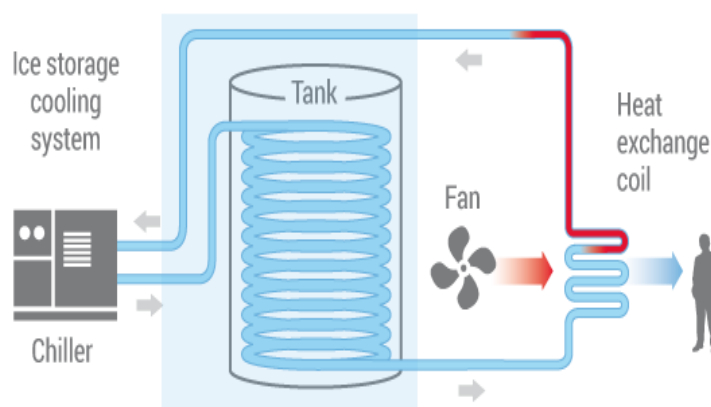
Figure37 Thermal ESS [85]
