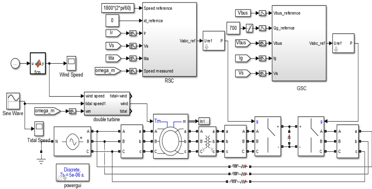
Figure 107 Schematic Diagram of DFIG Based Wind Turbine in MATLAB/Simulink
