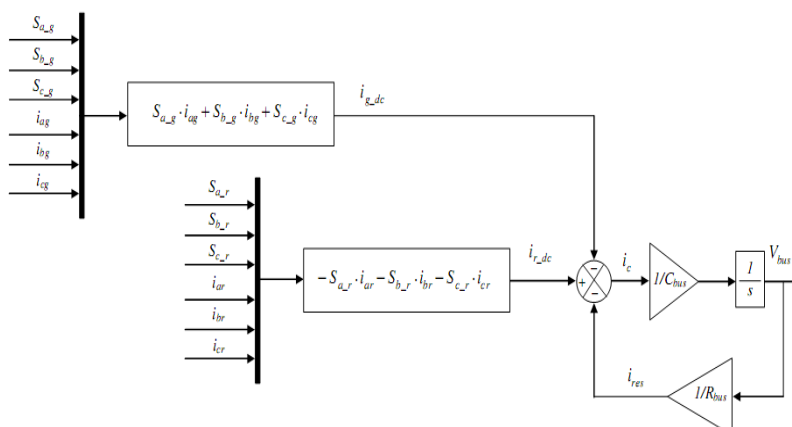
Figure 76 DC-Link Model
