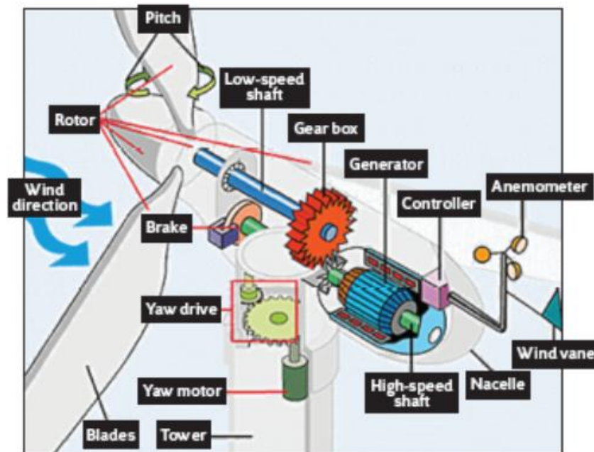
Figure16 Turbine Construction [25]
