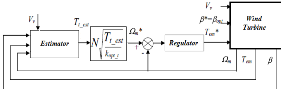
Figure 86 Direct Speed Control Block Diagram
