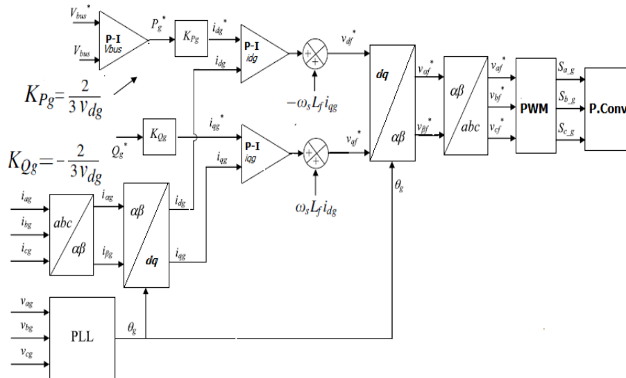
Figure 95 Grid Voltage Oriented Vector Control Block Diagram
