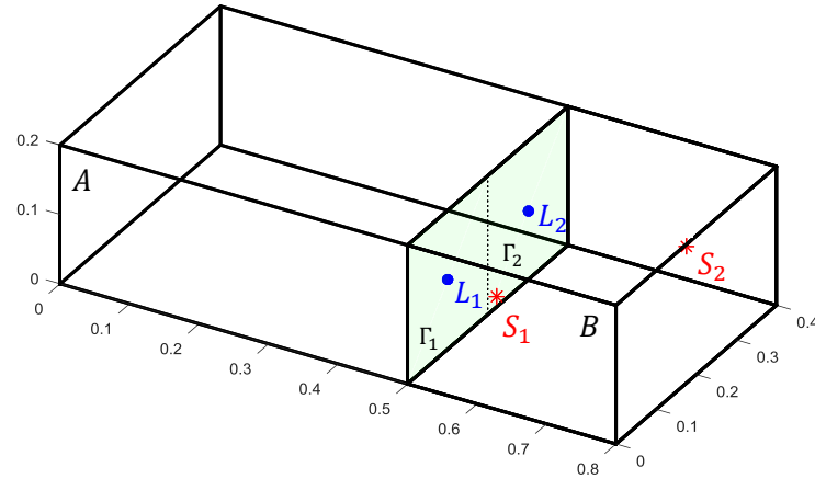
Figure 3.8: Description of the set of experiments necessary to characterize the impedance of the subsystem A. The set of experiments contains two positions of sources S_1 and S_2 in the system C to create two experiments for the characterization of the subsystem A—i.e. identification of the condensed impedance matrix [Z_{i \leftarrow j}^{AId}] . The pressure and velocity is measured at the position L_1 and L_2 considered as being in the center of the two “supposed patches” \Gamma_1 and \Gamma_2 . The patches are depicted only to illustrate where is the virtual limit between the two systems A and B.
