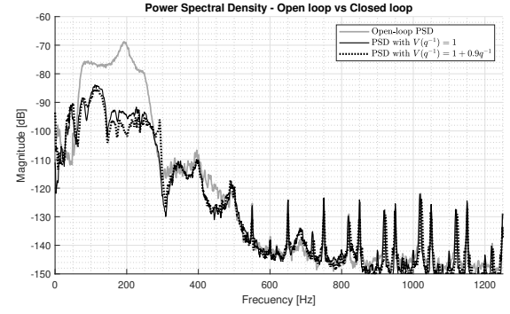
Fig. 21. PSD comparison of the residual noise in open-loop (solid grey line), using the adaptive compensator without filtering of the residual noise (solid black line), and using the adaptive compensator with filtering of the residual noise (dotted black line).
