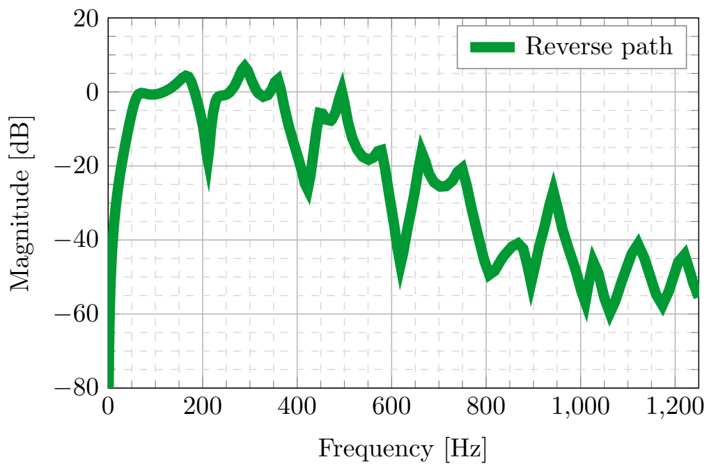
FIGURE 4.7. Identified reverse path for first test bench configuration.
