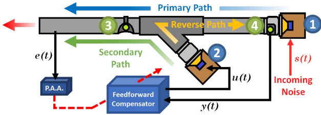
Fig. 5. Duct active noise control test-bench diagram.
