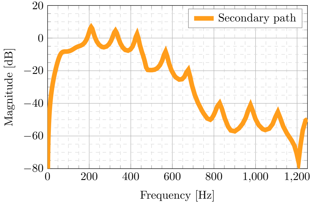
FIGURE 4.9. Identified secondary path for second test bench configuration.
