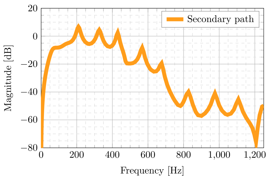
FIGURE 3.10. Second test bench configuration's identified secondary path.
