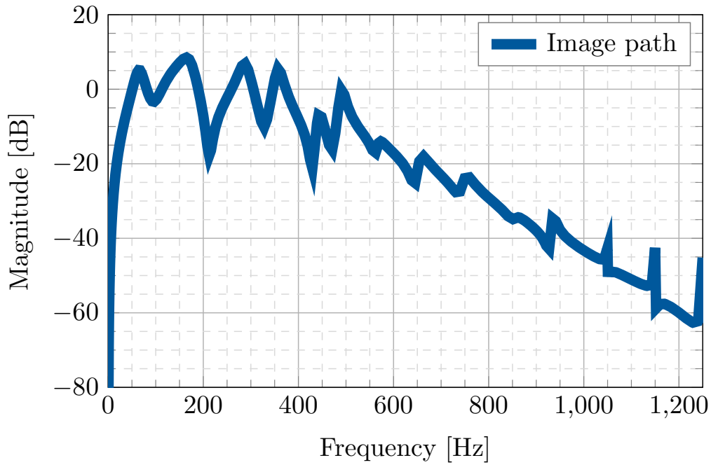
FIGURE 4.8. Identified image path for first test bench configuration.
