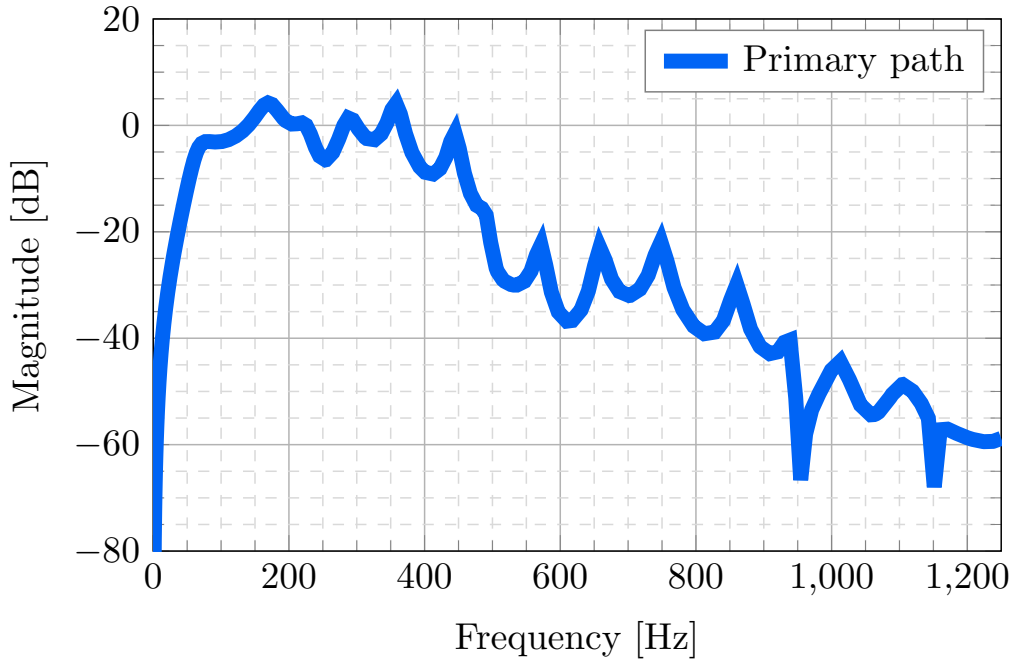
FIGURE 4.5. Identified primary path for first test bench configuration.
