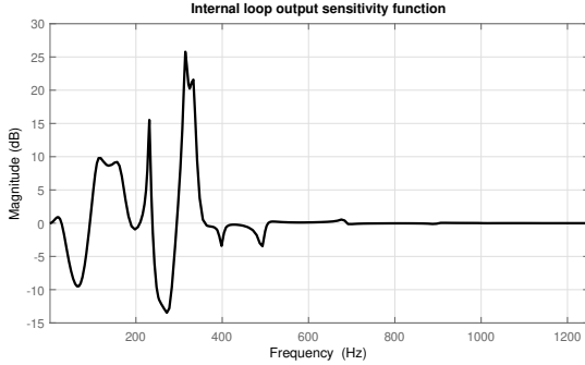
Fig. 9. Internal loop output sensitivity function for the IIR 15/15 adaptive compensator (70-270 Hz disturbance, 600 s experiments).
