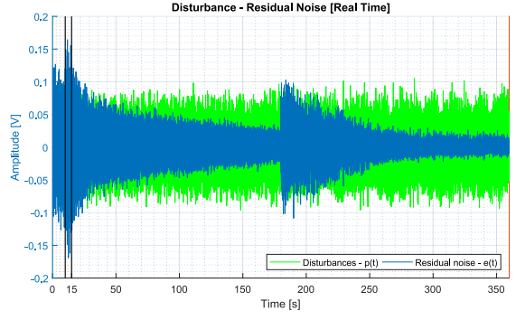
Fig. 11. Residual noise of the IIR 15/15 adaptive feedforward compensator for a change of disturbance from 170 - 270 Hz to 70 - 170 Hz at 180 s.
