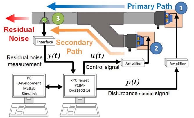
Fig. 2. Duct ANC test bench diagram.
