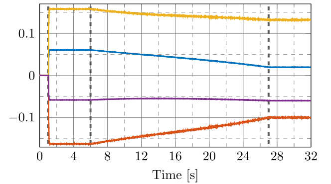
Fig. 13. Evolution of the controller parameters under the effect of tonal disturbances with variable frequency
