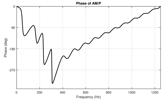
Fig. 13. Phase of \frac{A_M}{P} for the IIRYK 30/30 adaptive compensator (70-270 Hz disturbance, 600 s experiments).
