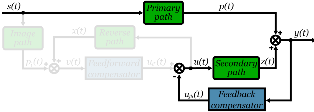
FIGURE 2.5. Reduced block diagram representation for a feedback control problem.
