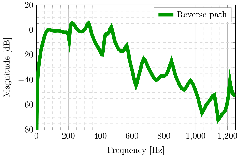
FIGURE 4.10. Identified reverse path for second test bench configuration.
