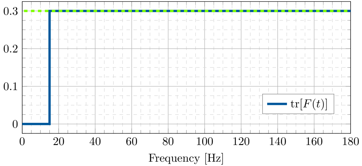
FIGURE 6.15. Evolution of adaptation matrix F 's trace for a constant trace profile of a FuSBA PAA. A value of \text{tr}[F]_{pp} = 0.010 was chosen, so \text{tr}[F(t)] = \text{tr}[F] = 0.3
