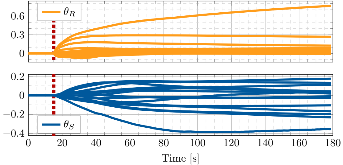
FIGURE 6.14. Filter N(q^{-1}) = \frac{R}{S} parameters evolution for a [15/15] standard IIR filter using FuSBA PAA with a constant trace profile. Compensation starts at 15 s.
