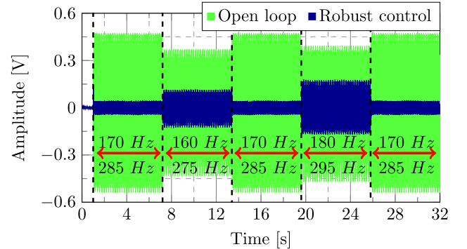
Fig. 14. Step changes in frequencies using the robust controller. Residual noise in open loop (green) and in closed loop (blue).
