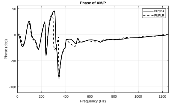
Fig. 10. Phase of \frac{A_M}{P} for the IIR 15/15 adaptive compensator (70-270 Hz disturbance, 600 s experiments).
