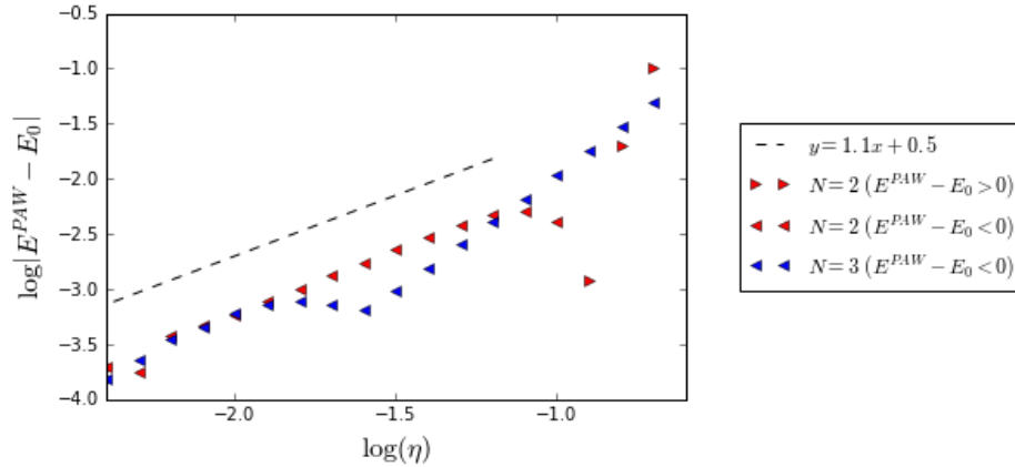
Figure 4.4.2 – Error on the lowest eigenvalue of the PAW equations (4.1.11) with pseudopotentials
