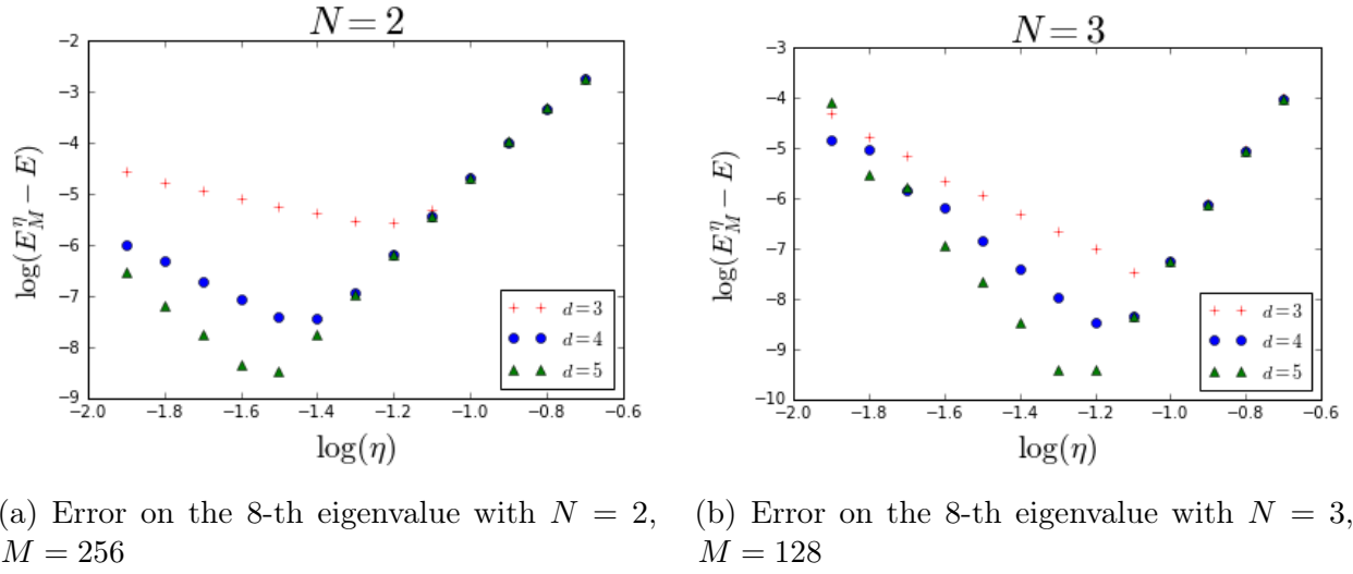
Figure 3.5.5 – Error on the eigenvalue for different values of d
