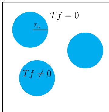
Figure 1.4.1 – Unit cell with PAW balls in blue
