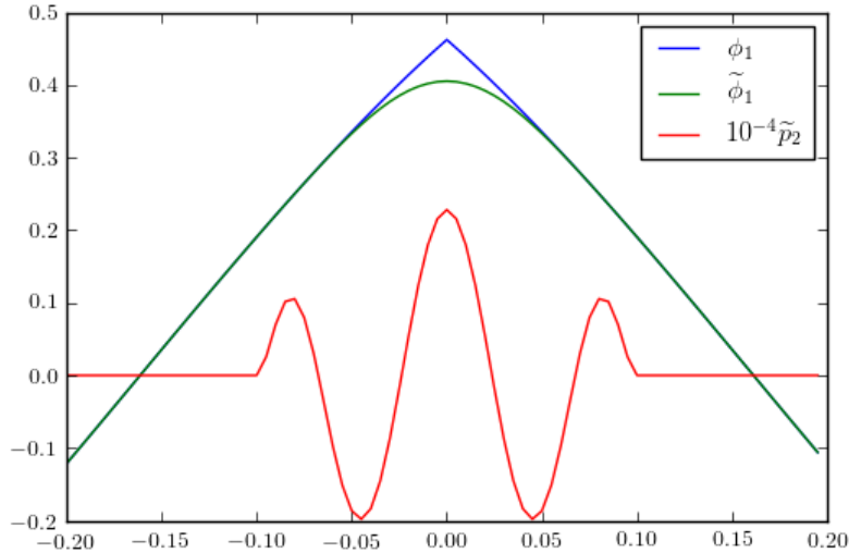
Figure 2.2.2 – Some PAW functions for the one-dimensional toy model ( Z_0 = 10 , a = 0.4 , r_c = 0.1 )
