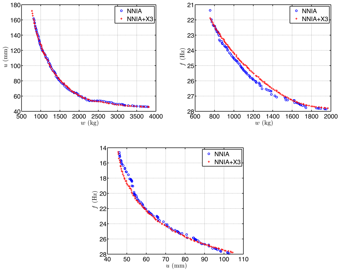
Figure III.7 – Pareto fronts of the ten-bar truss MO problem at iteration number 750 for one typical run when optimizing the three objective functions two-by-two: (w, u) (up-left), (w, f) (up-right), (u, f) (down).
