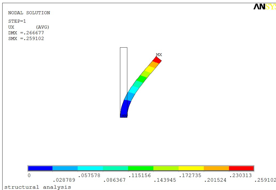
Figure VI.4 – Initial deflection of the plate
