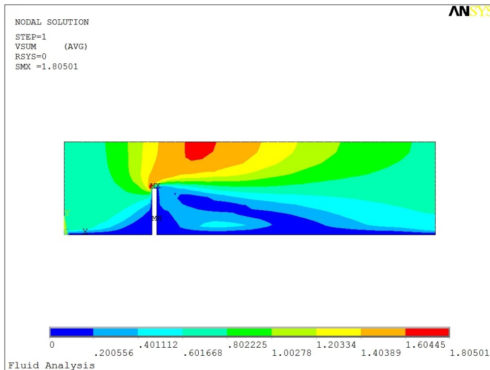
Figure VI.2 – Fluid velocity
