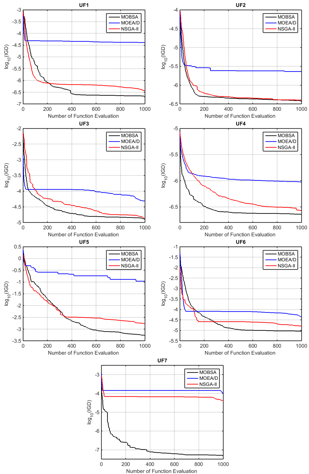
Figure IV.3 – Plot of the IGD evolution versus the number of functions evaluations for UF seri problems by using MOBSA, MOEA/D and NSGA-II algorithms in one typical run.
