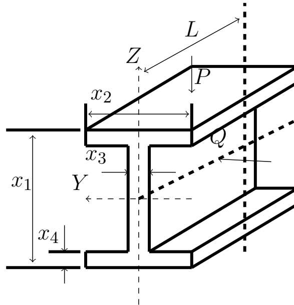
Figure V.2 – I-Beam optimization
