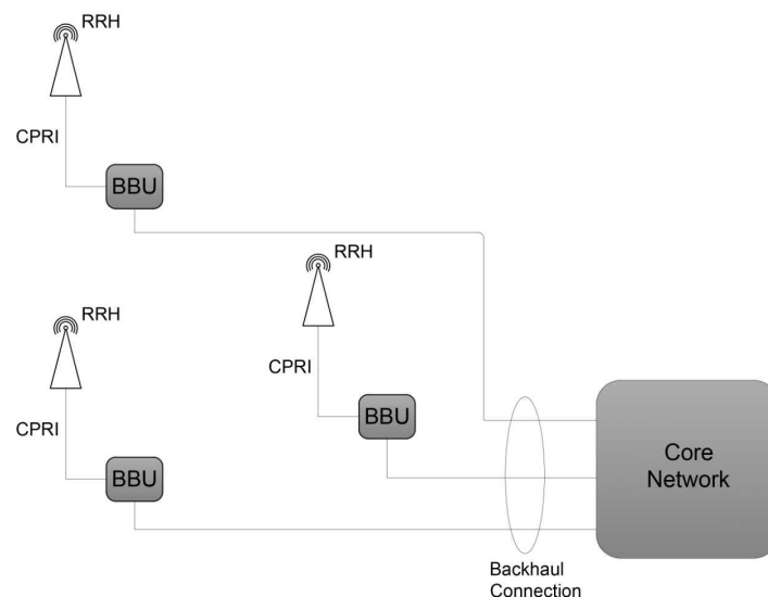
FIGURE 1.1: D-RAN Architecture
