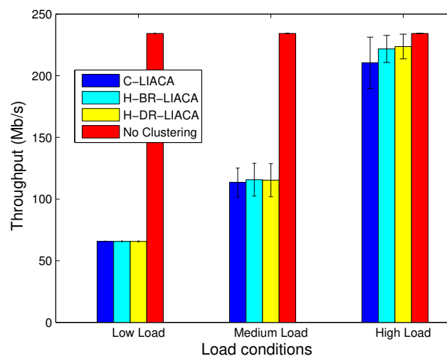
FIGURE 5.30: Total Throughput: C-LIACA vs. H-BR-LIACA vs. H-DR-LIACA vs. No Clustering
