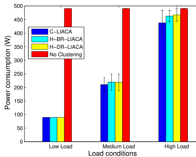
FIGURE 5.24: Power Consumption: C-LIACA vs. H-BR-LIACA vs. H-DR-LIACA vs. No Clustering
