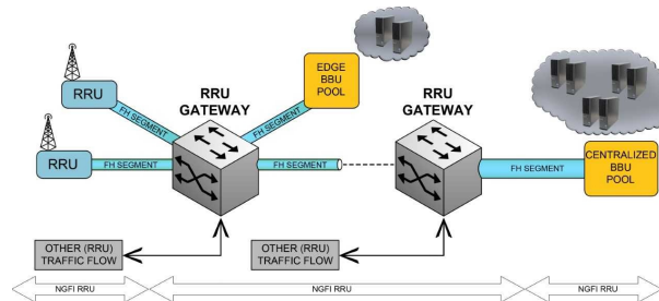
FIGURE 5.1: C-RAN Network Topology according to NGFI
