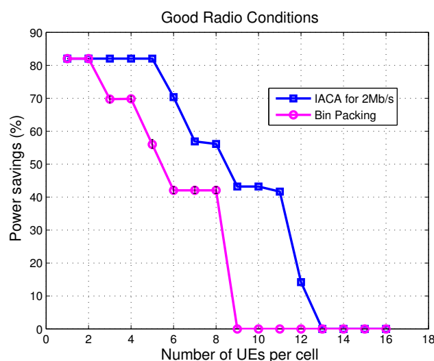
FIGURE 3.12: Power Savings: IACA vs. Bin Packing
