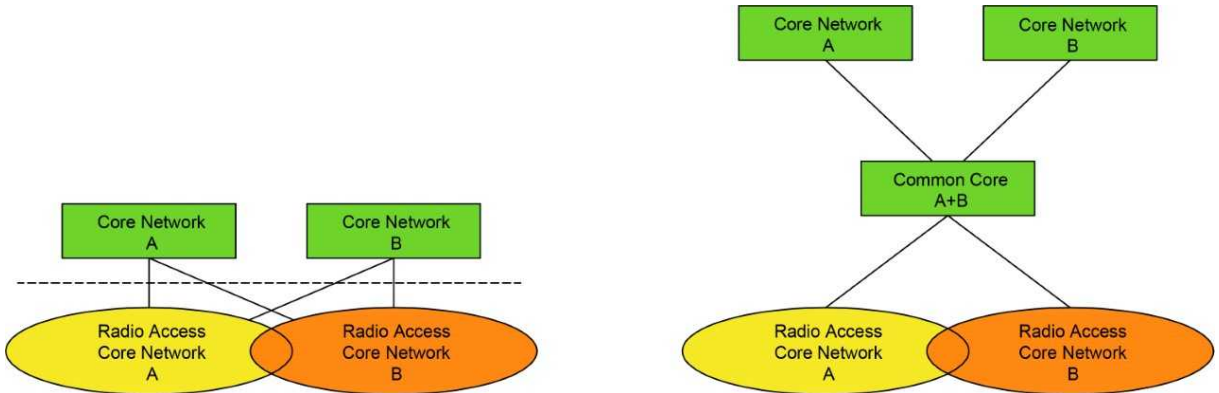
FIGURE 7.2: Geographically split network using dedicated or common core networks
