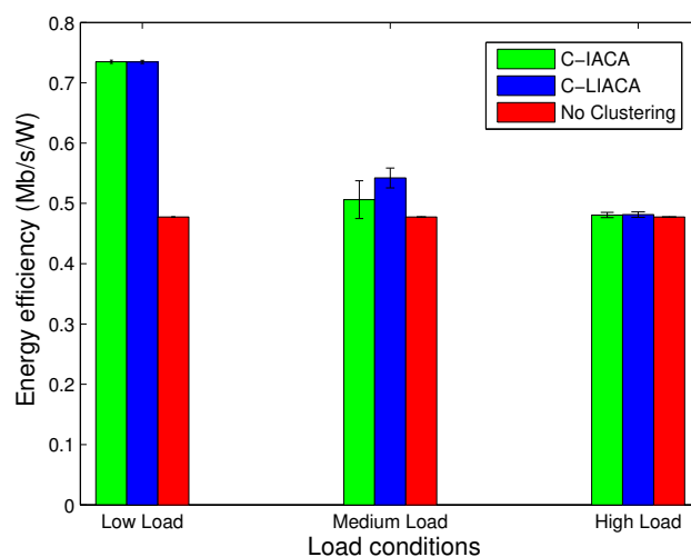
FIGURE 5.18: Energy Efficiency: C-IACA vs. C-LIACA vs. No Clustering
