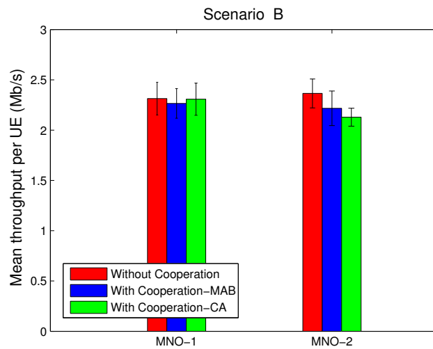
FIGURE 7.23: Scenario B: Mean Throughput per UE
