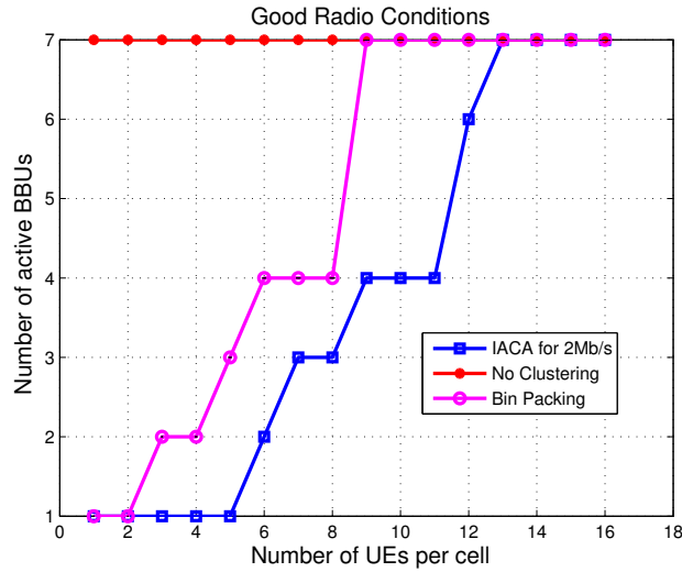
FIGURE 3.10: Number of Active BBUs: IACA vs. Bin Packing vs. No Clustering
