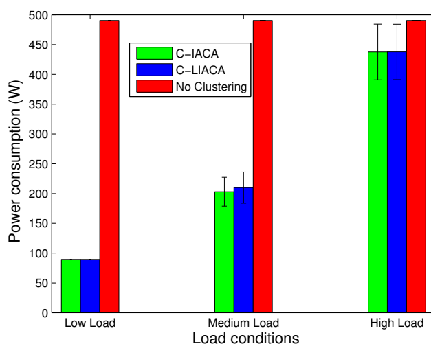
FIGURE 5.16: Power Consumption: C-IACA vs. C-LIACA vs. No Clustering
