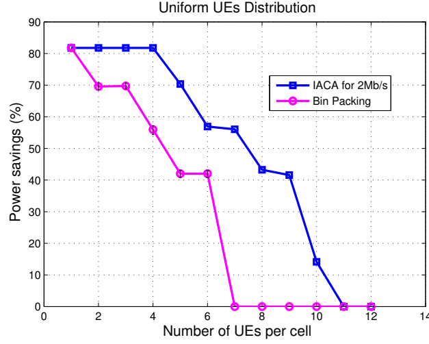
FIGURE 3.4: Power Savings: IACA vs. Bin Packing
