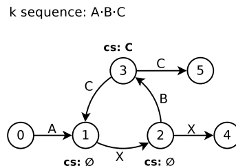
Figure 6.7: Common suffix calculation on an SCC.
