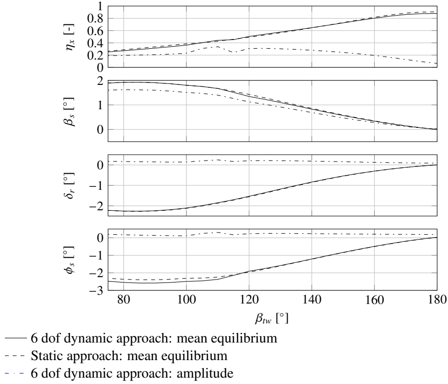
Figure 11.1.: For the calm water case, evolution of the mean kite efficiency \eta_x , mean drift angle \beta_s , mean rudder angle \delta_r and mean heel angle \phi_s with the true wind angle \beta_{tw} . The 6 dof dynamic approach (—) is compared to the static approach (---) in terms of mean equilibrium. The dashed-dotted lines correspond to the amplitudes obtained with the 6 dof dynamic approach (- · -). Kite configuration: L_t = 500 m, A_k = 500 m 2 , A^{(s)} = [110, 0, -10.6]^T m. Sailing condition: U_{tw} = 12.5 m.s -1 .
