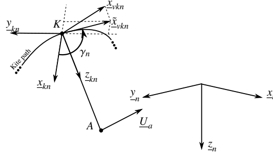
Figure 2.: Schema of the kite reference frame kn
