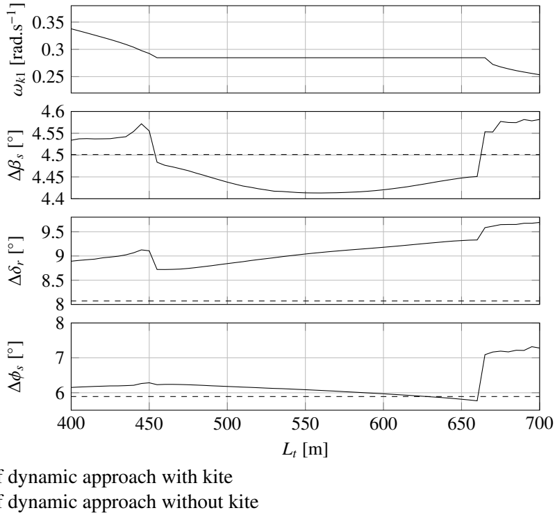
Figure 11.3.: With a regular wave in the wind direction, evolution of the first kite roll excitation harmonic frequency \omega_{k1} , drift angle amplitude \Delta\beta_s , rudder angle amplitude \Delta\delta_r and heel angle amplitude \Delta\phi_s with different tether lengths and a constant angular amplitude of trajectory. A configuration with kite (—) is compared to a configuration without kite (- - -). Kite configuration: A_k = 500 m 2 , A^{(s)} = [110, 0, -10.6]^T m. Sailing condition: \beta_{tw} = 135^\circ , U_{tw} = 12.5 m.s -1 , wave amplitude A_w = 2.5 m and wave angular frequency \omega_w = 0.4 rad.s -1 .
