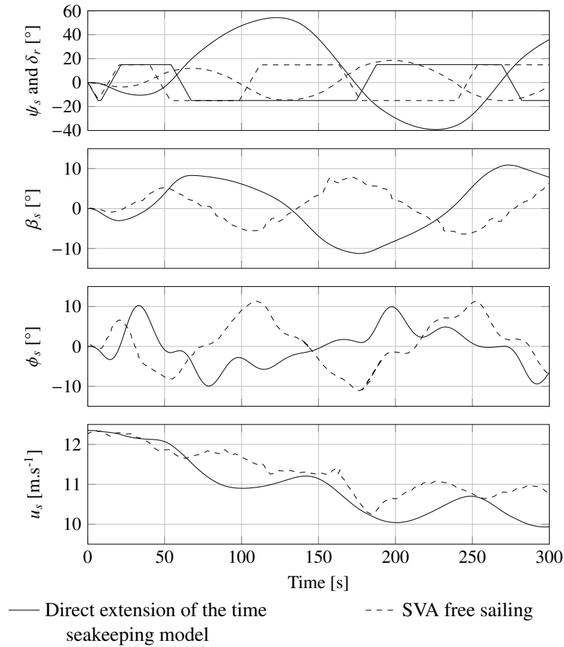
Figure C.17.: Time history during a zigzag 15/1^\circ maneuver of the: rudder angle \delta_r , heading \psi_s , drift angle \beta_s , heel angle \phi_s and surge velocity u_s . The results obtained with the direct extension of the time seakeeping model (—) are compared with the free sailing EFD data of the SVA (- - -).
