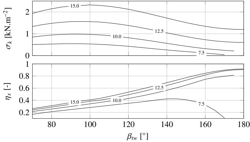
Figure 8.5.: For different true wind speed U_{tw} \in \{7.5, 10, 12.5, 15\} \text{m}\cdot\text{s}^{-1} : evolution with the true wind angle of the mean aerodynamic pressure \sigma_k and of the kite efficiency \eta_x .
