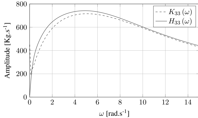
Figure C.3.: Comparison of the amplitude of the transfer function K_{33} in dashed line with the identified transfer function in solid line H_{33} with the time domain method
