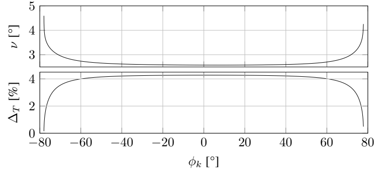
Figure 4.6.: Difference of tether tension between A and K for different kite azimuth angle; in terms of direction on the top; in terms magnitude on the bottom
