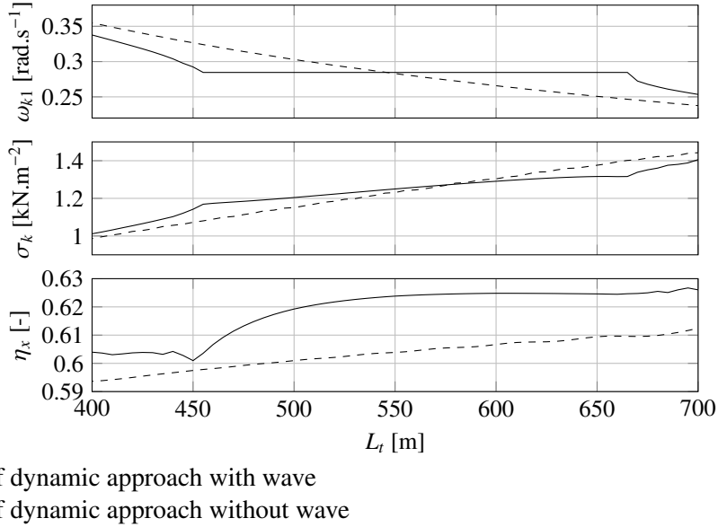
Figure 11.5.: With a regular wave in the wind direction, evolution of the first kite roll excitation harmonic frequency \omega_{k1} , mean kite wind loading \sigma_k , mean kite efficiency \eta_x with different tether lengths and a constant angular amplitude of trajectory. A configuration with wave (—) is compared to a configuration without wave (---). Kite configuration: A_k = 500 \text{ m}^2 , A^{(s)} = [110, 0, -10.6]^T \text{ m} . Sailing condition: \beta_{tw} = 135^\circ , U_{tw} = 12.5 \text{ m.s}^{-1} , wave amplitude A_w = 2.5 \text{ m} and wave angular frequency \omega_w = 0.4 \text{ rad.s}^{-1} .
