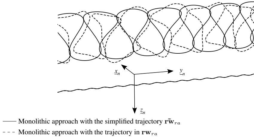
Figure 9.4.: Kite and ship path with respect to \mathbf{n} for L_t = 390 m with a wave of 2.5 m high at the frequency \omega_w = 0.8 rad.s -1 .
