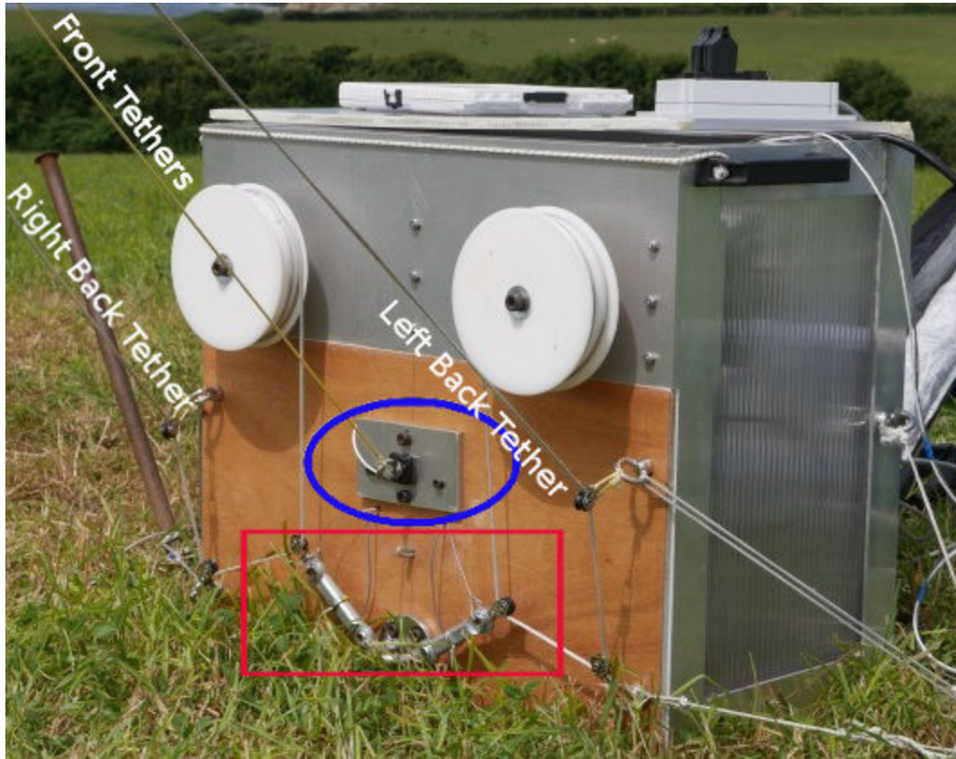
Figure A.2.: Kite control and measurement device deployed on shore. The two winches are visible, as well as the 3D front tether load cell (blue ellipse) and the two 1D back tether load cells (red rectangle). Source: Behrel et al. (2017)
