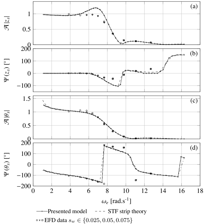
Figure 6.3.: Heave and pitch transfer function at U_h = 1.53 \text{ m.s}^{-1} as function of the wave frequency of encounter w_e . The results are obtained with the frequency domain and time domain approaches, experimental data for different wave steepnesses s_w and with the STF strip theory.
