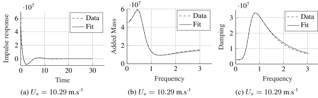
Figure C.18.: (a) plot of the impulse response function K_{22} from the data and the analytical fit H_{22} ; (b) plot of the added mass A_{22} from the data and from the analytical fit; (c) plot of the damping B_{22} from the data and from the analytical fit
