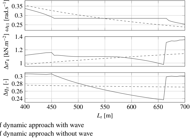
Figure 11.4.: With a regular wave in the wind direction, evolution of the first kite roll excitation harmonic frequency \omega_{k1} , kite wind loading amplitude \Delta\sigma_k , kite efficiency amplitude \Delta\eta_x with different tether lengths and a constant angular amplitude of trajectory. A configuration with wave (—) is compared to a configuration without wave (---). Kite configuration: A_k = 500 m 2 , A^{(s)} = [110, 0, -10.6]^T m. Sailing condition: \beta_{tw} = 135^\circ , U_{tw} = 12.5 m.s -1 , wave amplitude A_w = 2.5 m and wave angular frequency \omega_w = 0.4 rad.s -1 .
