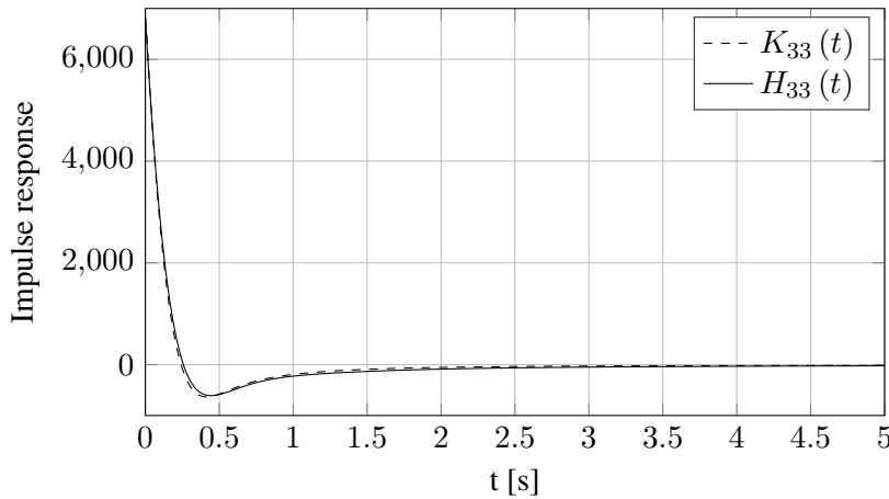
Figure C.2.: Comparison of the impulse response according to the data K_{33} in dashed line compared to the estimated transfer function of order 4 with the time domain method in solid line.
