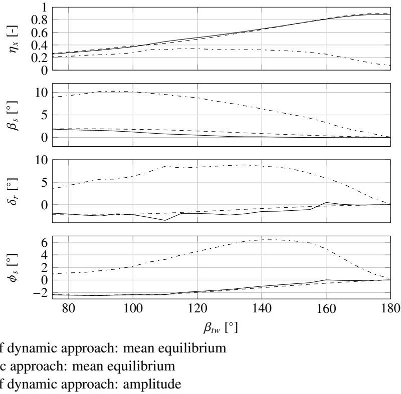
Figure 11.2.: For the regular wave case, evolution of the mean kite efficiency \eta_x , mean drift angle \beta_s , mean rudder angle \delta_r and mean heel angle \phi_s with the true wind angle \beta_{tw} . The 6 dof dynamic approach (—) is compared to the static approach (---) in terms of mean equilibrium. The dashed-dotted lines correspond to the amplitudes obtained with the 6 dof dynamic approach (- · -). Kite configuration: L_t = 500 m, A_k = 500 m 2 , A^{(s)} = [110, 0, -10.6]^T m. Sailing condition: U_{tw} = 12.5 m.s -1 , wave amplitude A_w = 2.5 m and wave angular frequency \omega_w = 0.4 rad.s -1 .
