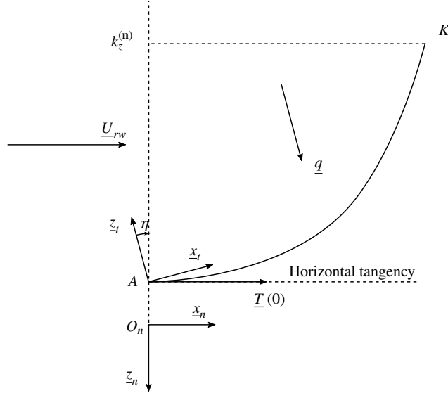
Figure 5.1.: Diagram of the lower limit static flight case
