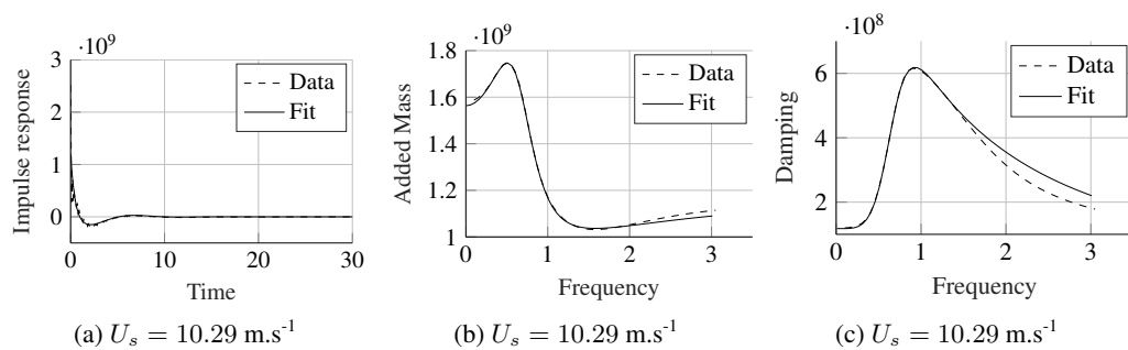
Figure C.24.: (a) plot of the impulse response function K_{44} from the data and the analytical fit H_{44} ; (b) plot of the added mass A_{44} from the data and from the analytical fit; (c) plot of the damping B_{44} from the data and from the analytical fit
