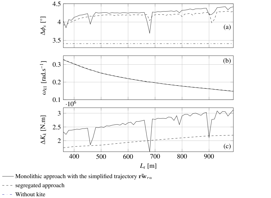
Figure 9.7.: (a) Amplitude of the ship roll motion, (b) first kite harmonic frequency and (c) amplitude of the kite moment of excitation for different tether lengths from 360 m to 990 m by step length of 10 m with a beam regular wave of 2.5 m high at a frequency of \omega_w = 0.8 \text{ rad.s}^{-1} .
