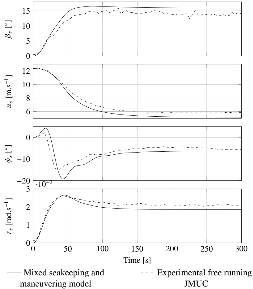
Figure 7.3.: Time history during a 35^\circ turning circle maneuver of the: drift angle \beta_s , surge velocity u_s , heel angle \phi_s , surge velocity u_s and yaw turning rate r_s . The results obtained with the mixed seakeeping and maneuvering model (—) are compared with the free sailing EFD data of the SVA (- - -).
