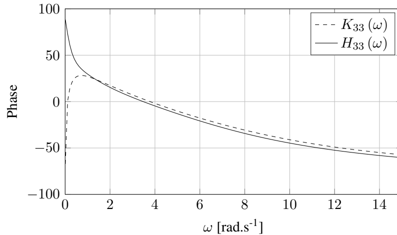
Figure C.4.: Comparison of the phase of the transfer function K_{33} in dashed line with the identified transfer function in solid line H_{33} with the time domain method
