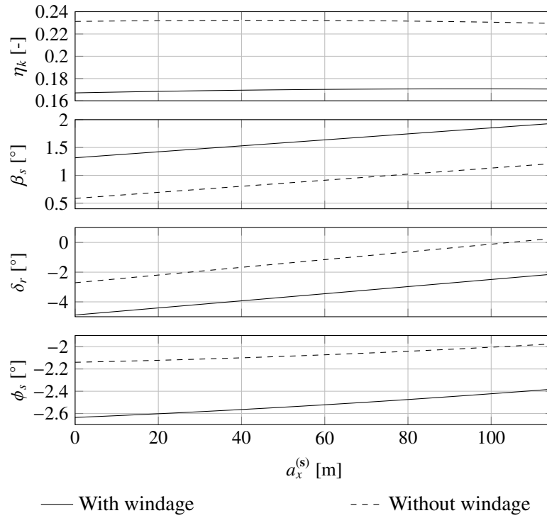
Figure 8.3.: For U_{tw} = 12.5 \text{ m}\cdot\text{s}^{-1} , \beta_{tw} = 90^\circ , L_t = 500 \text{ m} and A_k = 500 \text{ m} : mean evolution of the kite power saving ratio \eta_k , drift angle \beta_s , rudder angle \delta_r and heel angle \phi_s with the longitudinal position of the tether attachment point a_x^{(s)} . The solid line is the mean equilibrium with the windage taken into account. The dashed line is the mean equilibrium without the windage effect.
