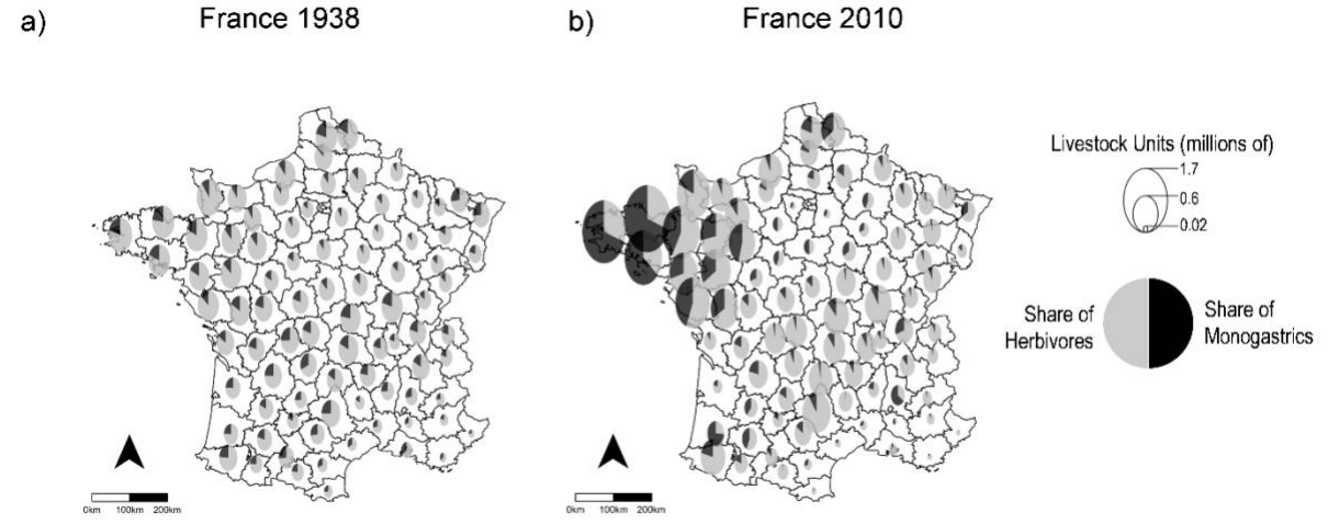
Figure V-2. The changes in the livestock population of herbivores (cattle, sheep, goat, horse) and monogastrics (pig, poultry) and in the species composition over time in France at the department level from 1938 (a) to 2010 (b).
