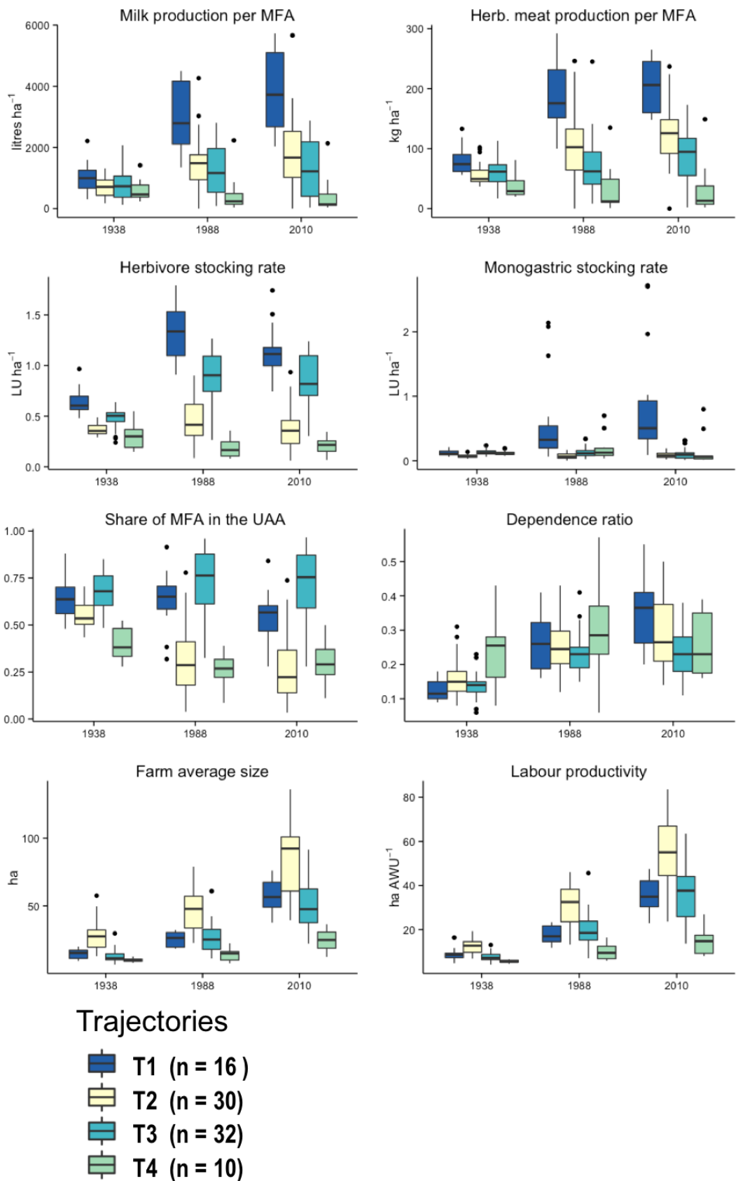
Figure III-5. Trends of change observed in the French departments per type of trajectory. T1, 2, 3, and 4 correspond to 'High intensification of livestock production', 'Crop orientation and intermediate intensification of livestock', 'Grazing orientation of livestock production', and 'Non-livestock dominated' departments, respectively.
