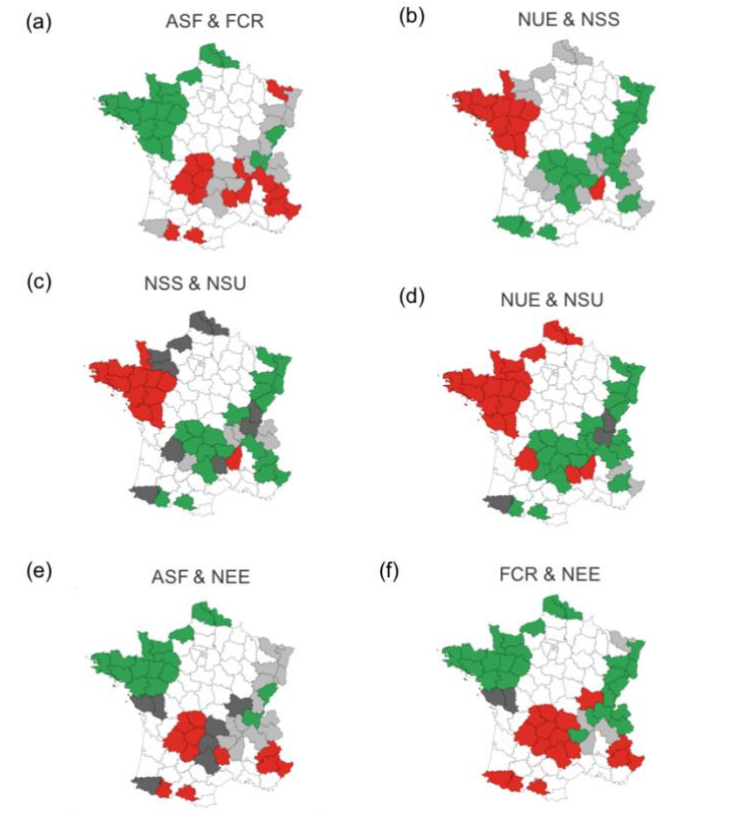
Figure III-8. Spatial decomposition of synergies among performance (a-b) and among performance and impacts (c-f) in 48 livestock dominated NUTS3 units. Green: Superior; Red: Inferior; Grey: Intermediate. ASF: Animal Source Food; FCR: Nitrogen Feed Conversion Ratio; NUE: Fodder Nitrogen Use Efficiency; NSS: Nitrogen Self-Sufficiency; NEE: N Excretion Emissions; NSU: Nitrogen Surplus.
