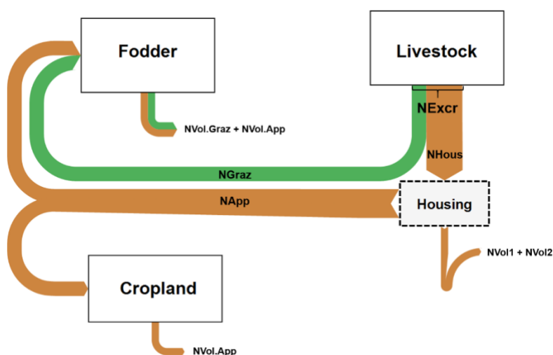
Figure II-3. Nitrogen excretion flows decomposition. NExcr : N excretion; NHous : N excretion on housing; NGraz : N excretion on grazing; NApp : N manure application; NVol : N volatilization on housing ( NVol1 ), manure storage ( NVol2 ), during grazing ( NVol.Graz ) and of application ( NVol.App ) (adapted from SOeS, 2013)
