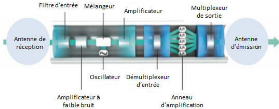
Figure I.6 : Architecture d'une charge utile [5].
