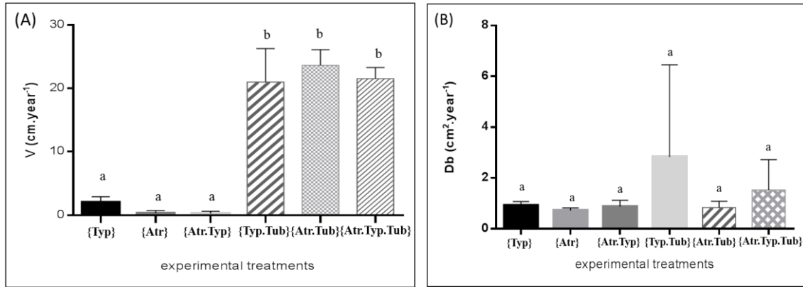
Fig. 3. (A): bioadvective rates -( V , ) and (B): biodiffusive rates - ( Db ,) estimated after 26 days for the different experimental treatments. For each parameters, the variable same letters at the top of the bars indicate treatments that were not significantly different ( P < 0.05 ) as analyzed by TUKEY HDS multiple comparison test. Values are means \pm SD, n = 4 , excepted for {Typ.Tub}, {Atr.Tub}, {Atr.Typ.Tub} with ( n = 3 ) . (see Table 1 for the definitions of acronym corresponding to the different treatments).
