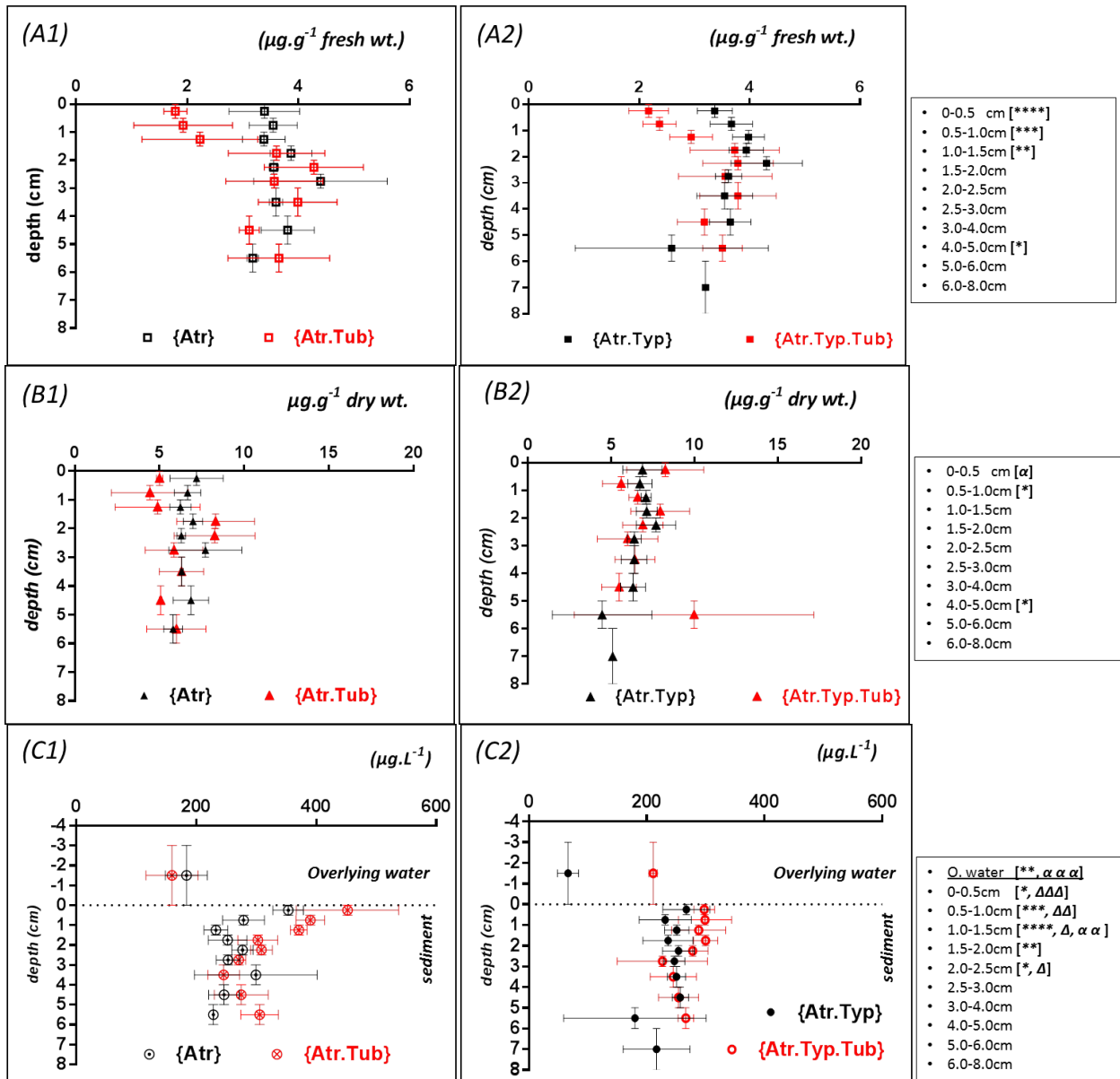
Figure. III.5. [ 14 C]-atrazine + metabolites) concentrations according to depth and experimental treatments for different sediment fractions (A1 and A2: fresh sediment (or bulk sediment: being the sum of sediment particles and interstitial water); B1 and B2: sediment particles; C1 and C2: overlying water and pore water) at the end of the experiment (t=26). Values are means \pm S.D., replicate (n) = 4 per treatment group. (*), (**), (***), and (****) indicate significance effects of worms addition at P \leq 0.05, 0.01, 0.001, and 0.0001 respectively according to the two-way ANOVA (The test were performed on the concentrations of the four treatments: {Atr}, {Atr.Typ}, {Atr.Tub}, and {Atr.Typ.Tub}). Similarity, the number of \Delta and \alpha indicate the level of significance of T. latifolia effect the level of the two factors interactions, respectively at different levels of P values according to the two-way ANOVA (see Table II.2 for the definitions of acronym corresponding to the different treatments).
