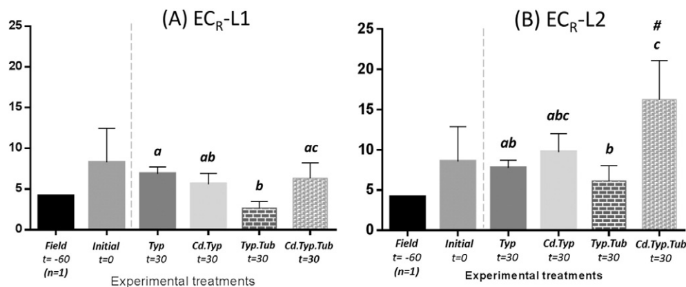
Fig. 7. Enrichment coefficients for the roots ( EC_R ) of Typha latifolia at two different sediment layers ((A): L1; (B): L2). Values are means ± S.D., n = 3 per treatment group, except for the field sample ( n = 1 ). (#) indicates significant differences between a given treatment at t = 30 and the initial EC_R value (Dunnett test); Different superscript letters indicate significant differences for EC_R between treatments at t = 30 , assessed separately at the two sediment layers (Tukey HSD test). See Table 1 for the meaning of acronyms corresponding to the different treatments.
