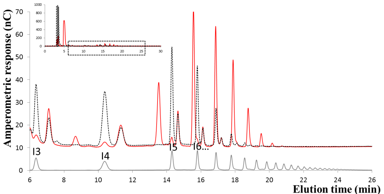
Figure S11: HPAEC-PAD profiles of reaction medium at 15min reaction using DSR-MAV-W624A on 292mM sucrose. Red: Before invertase digestion, Black dots: after invertase digestion. Grey: commercial dextran 1500. Reaction products are mainly elongated sucrose but pure isomaltoligosaccharides are present in major amount than the wt enzyme.
