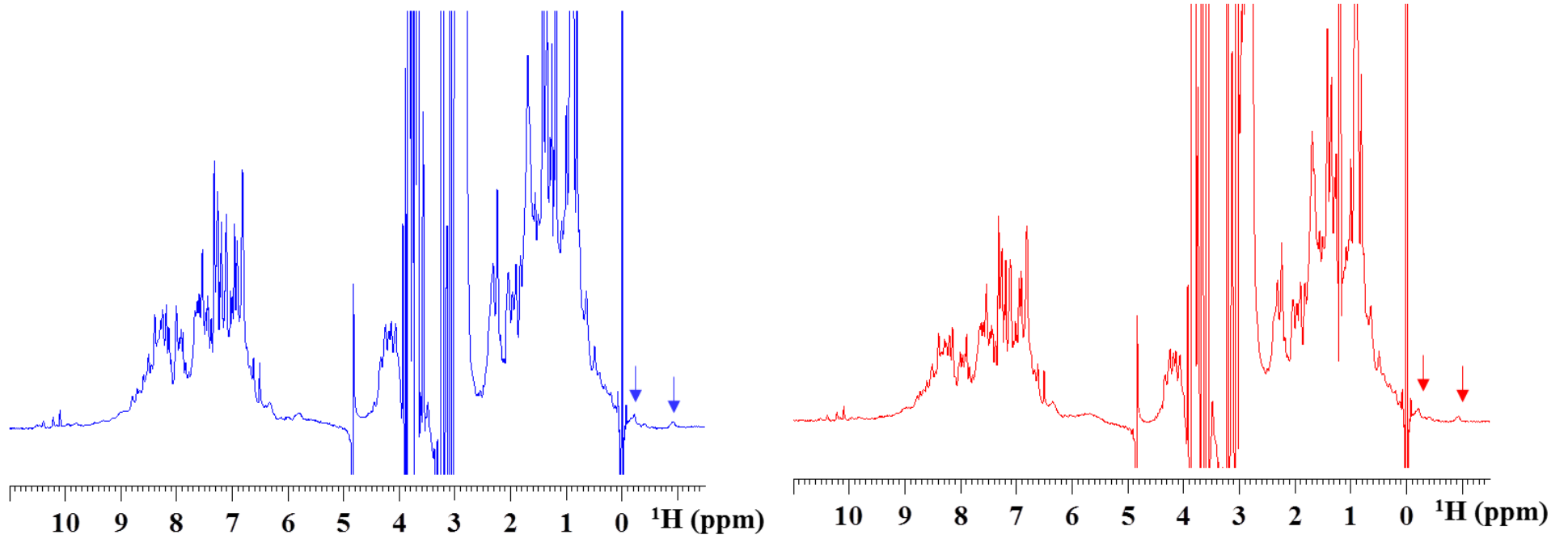
Figure NMR3: 1D proton NMR spectra of DSR-MDV wt U- ^{15}N labeled (left) and DSR-MDV W624A U- ^{15}N labeled (right)
