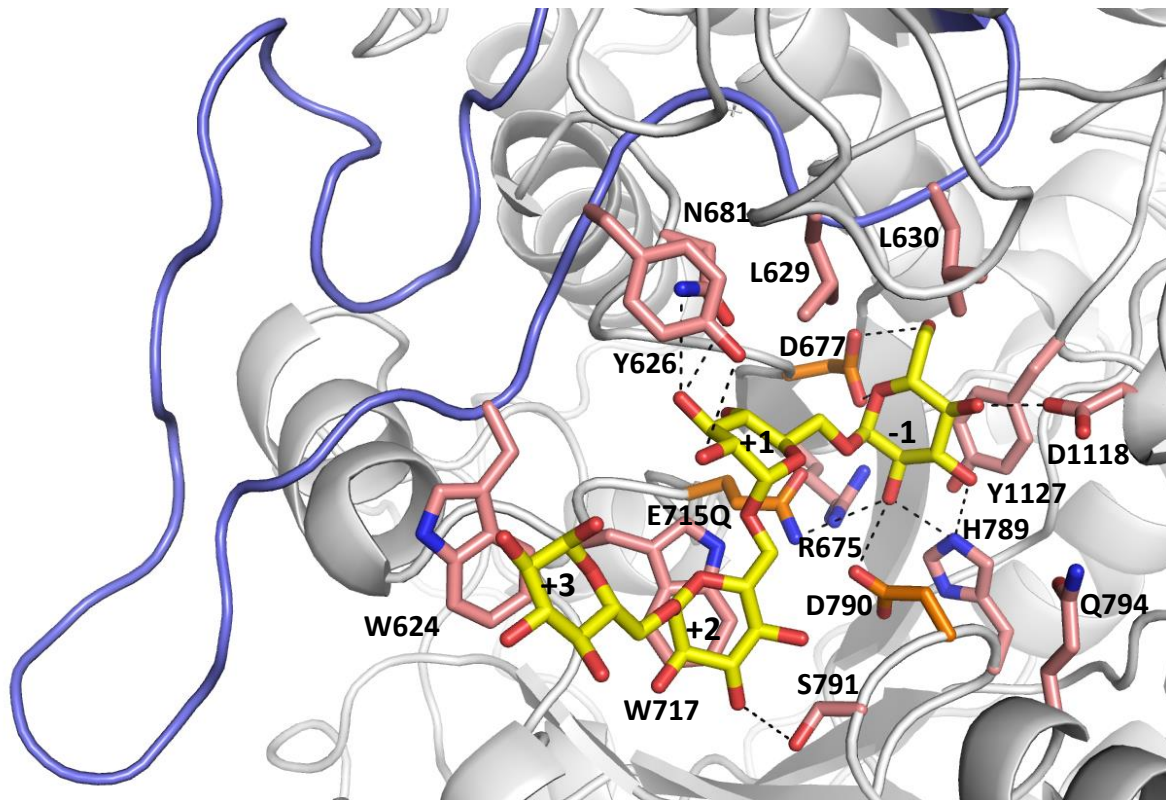
Figure 37: Crystal structure of DSR-M \Delta 2-E715Q with an isomaltotetraose. Indole rings form a platform for the nascent dextran chain with the two glucosyl units Glc+3 and Glc+2 stacking against the aromatic rings of Trp624 and Trp717, respectively. Catalytic residues are shown in orange sticks; residues participating in the catalytic site are shown in salmon sticks; Loop B2 (600-632) is presented in purple, helix H1' (807-817) has been removed for clarity.
