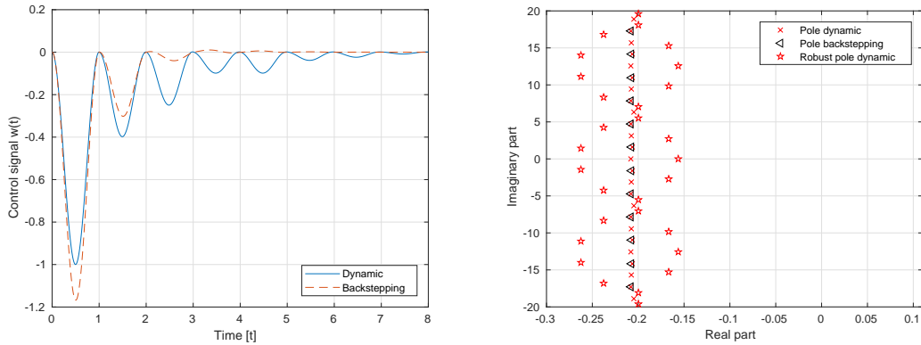
(c) Control signals w based on the dynamic controller (F.2) (blue) and backstepping controller (F.13) (dashed red).
