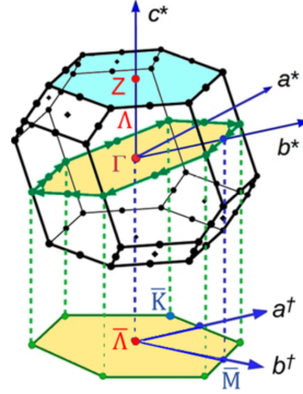
Figure 1.18: The Brillouin zone of \text{ReS}_2 . a^*, b^*, c^* are the reciprocal lattice vectors and the high-symmetry Z-plane, \Gamma -plane and its projection on the k_z=\text{constant} plane are shaded [Webb 2017].
