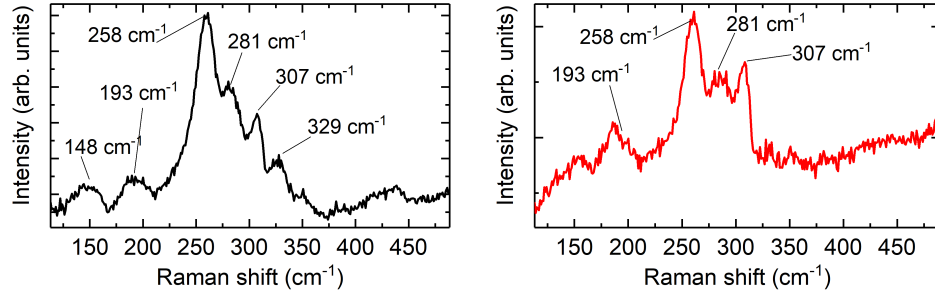
Figure 5.10: Raman spectrum of the thicker franckeite flake with marked characteristic modes for (a) co-polarized and (b) cross-polarized detection configurations and averaged over the full range of excitation directions.
