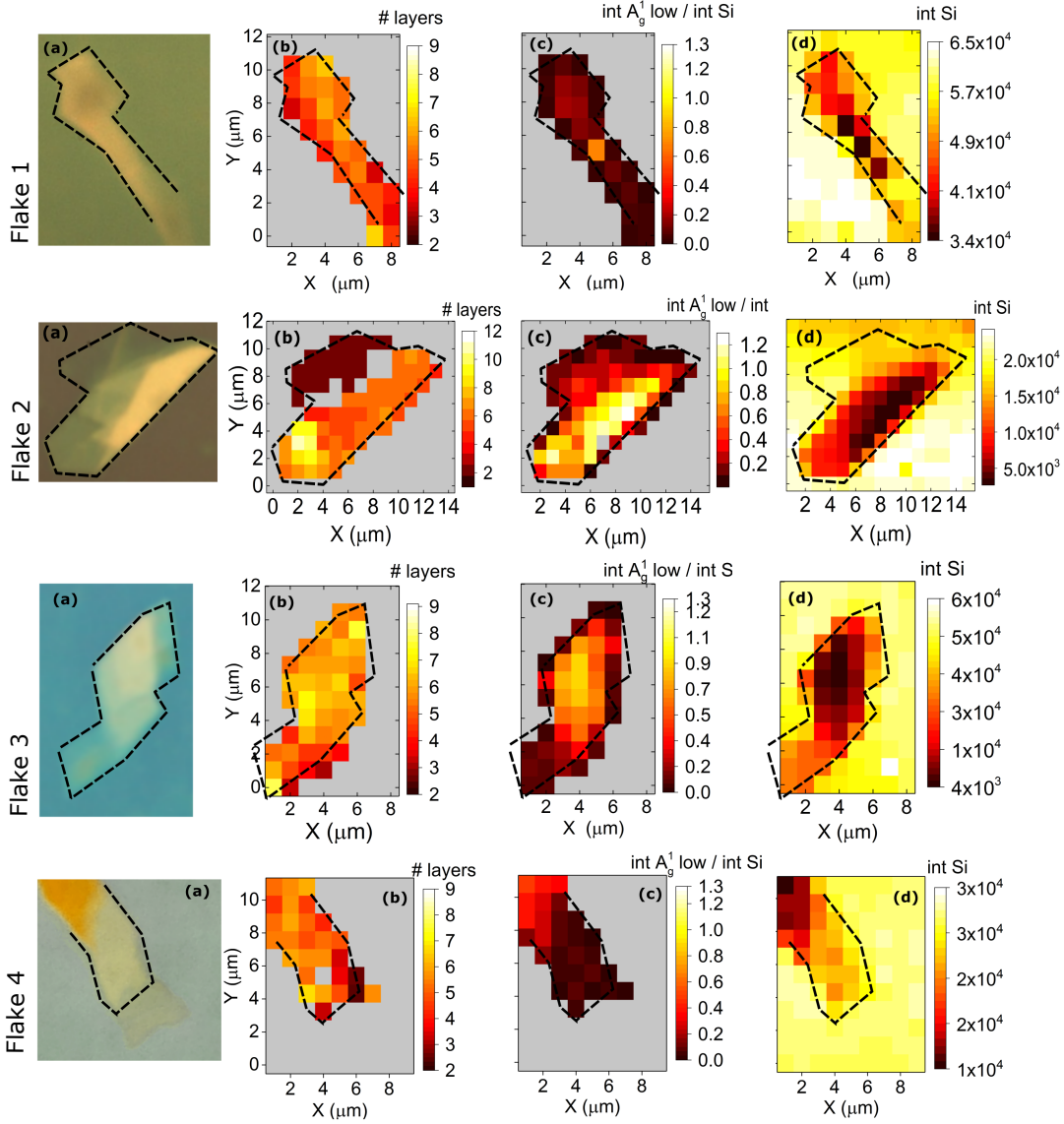
Figure 3.11: (a) Optical micrograph of the flakes, (b) calculated number of layers, (c) A_g^1 //Si peak intensity ratio and (d) Si 520 \text{ cm}^{-1} peak intensity for four different investigated flakes.
