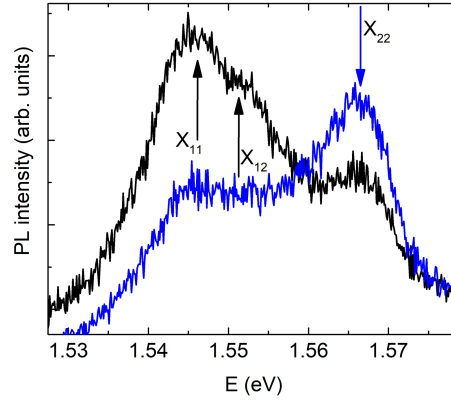
Figure 4.20: Photoluminescence spectra for two different polarization detection angles 0° (black) and 140° (blue). The arrows mark the approximate energies of the transitions.
