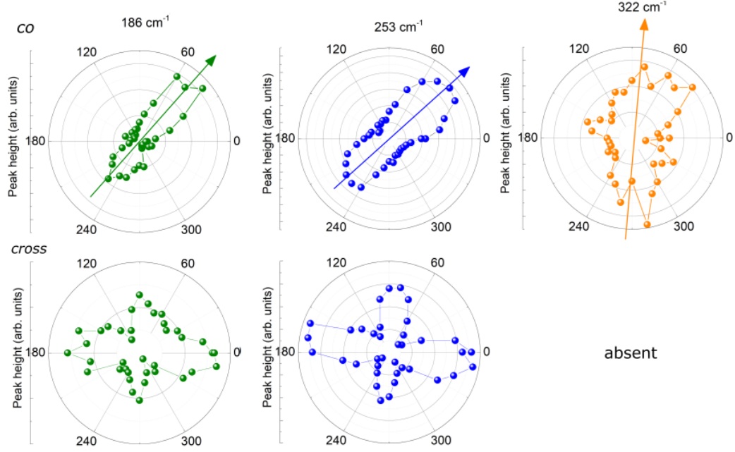
Figure 5.14: Polar plots showing the intensity of the 186\text{ cm}^{-1} (green), 253\text{ cm}^{-1} (dark blue) and 322\text{ cm}^{-1} mode as a function of excitation angle in the copolarized (top) and cross-polarized (bottom) configuration. The 322\text{ cm}^{-1} mode was not observed in the cross-polarization. The arrows mark the approximate directions of the maximum intensity.
