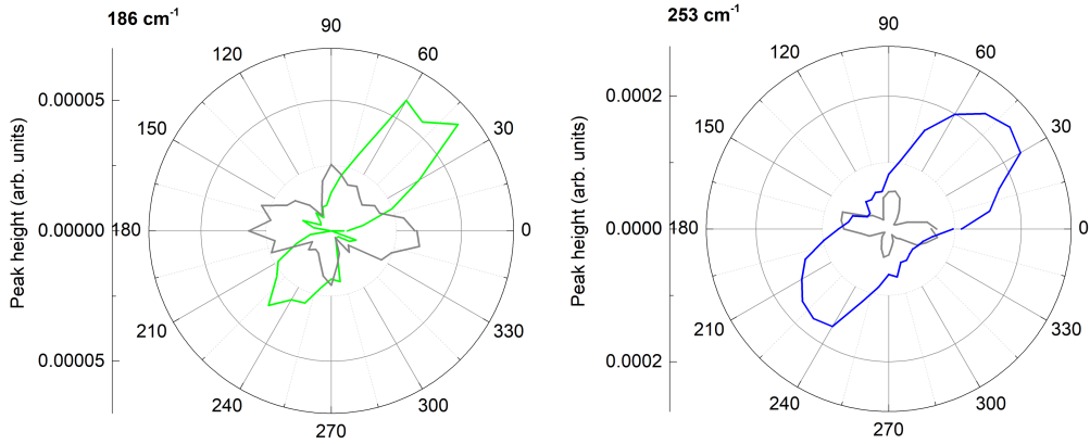
Figure 5.15: Raman mode height as a function of the excitation angle in the co- (color) and cross-polarization (grey) for the 186\text{ cm}^{-1} and 253\text{ cm}^{-1} modes.
