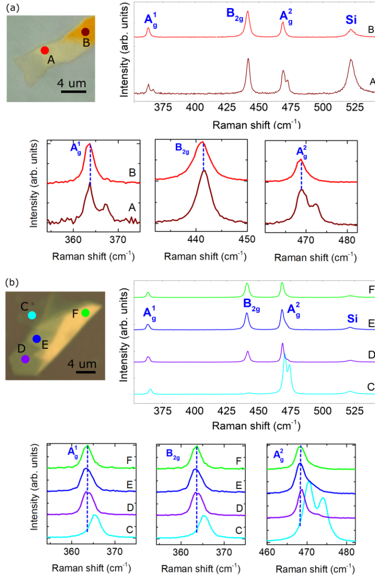
Figure 3.7: Raman spectra showing the three Raman active modes of BP and the Raman mode around 520\text{ cm}^{-1} from the Si substrate normalized to the A_g^1 mode intensity, optical micrographs of flakes with marked spots at which representative spectra were taken and the A_g^1 , B_{2g} and A_g^2 Raman peaks in larger scale for two different flakes (a) and (b).
