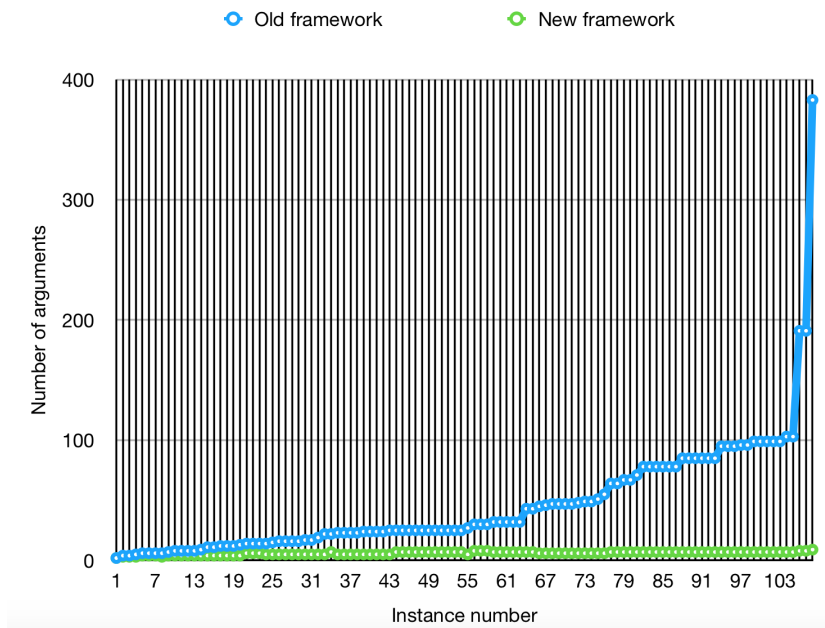
Figure 4.3: Number of arguments for both the old framework \mathfrak{F}_{\mathcal{KB}} and the new framework \mathfrak{F}^*_{\mathcal{KB}} with the set of knowledge bases A . Instances are sorted with respect to the number of arguments of \mathfrak{F}_{\mathcal{KB}}
