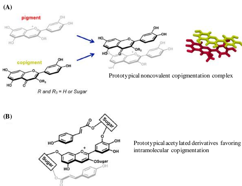
Figure 1.12 Prototypical copigmentation complexes. (A) Noncovalent association of anthocyanin pigment and flavanoid copigment (intermolecular copigmentation). (B) Acylated derivatives allowing copigmentation between anthocyanin moiety and two phenolic acids covalently linked (intramolecular copigmentation). Adapted from Trouillas et al. (2016).
