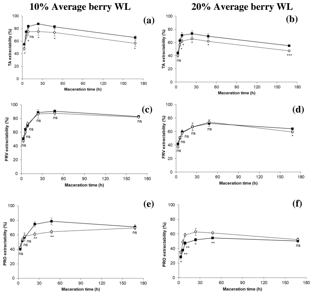
Figure 4.3 Effect of gaseous ozone exposure on the extractability of total anthocyanins (a, b), monomeric and oligomeric flavanols (c, d) and polymeric flavanols (e, f) during maceration for Nebbiolo winegrapes partially dehydrated at 10% WL (a, c, e) and 20% WL (b, d, f).
