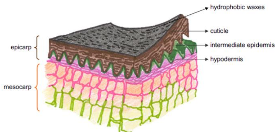
Figure 1.10 Different layers of the grape skin (From Pinelo et al. , 2006).
