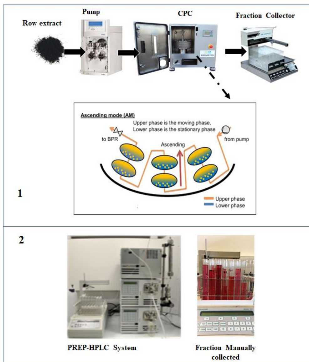
Figure 5.2 CPC separation scheme (1) and Prep-HPLC (2).
