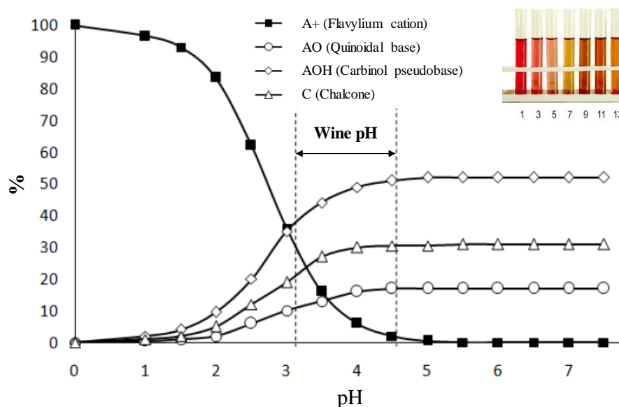
Figure 1.7 Proportion of the different anthocyanins forms depending on the solution pH. Adapted from Zeng, 2015.
