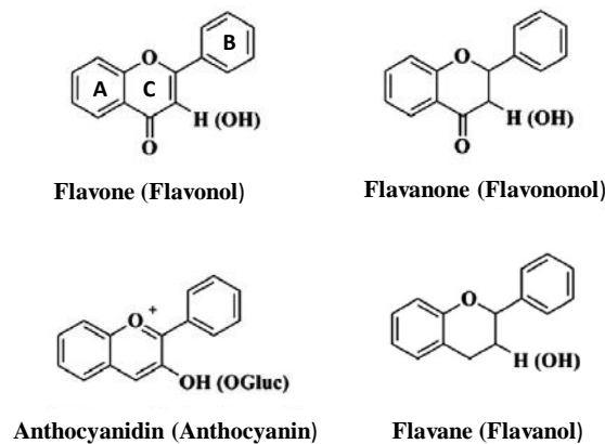
Figure 1.4 Skeleton of the main flavonoids in grape.
