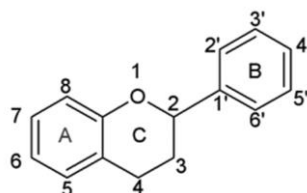
Figure 1.3 Flavonoids general structure: the C 6 -C 3 -C 6 skeleton.
