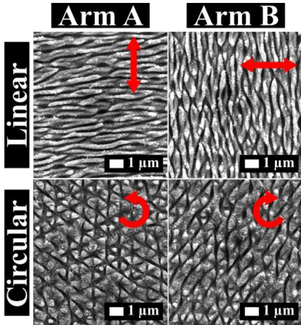
Figure 66 SEM images of stainless-steel surface after single arm irradiation for linear and circular pulse configuration as indicated. The polarization direction is indicated by a red arrow. The irradiation parameters were the same for both arms: H=1 \mu\text{m} , \text{pps} = 10 and \Phi = 0.1 \text{J}/\text{cm}^2 .
