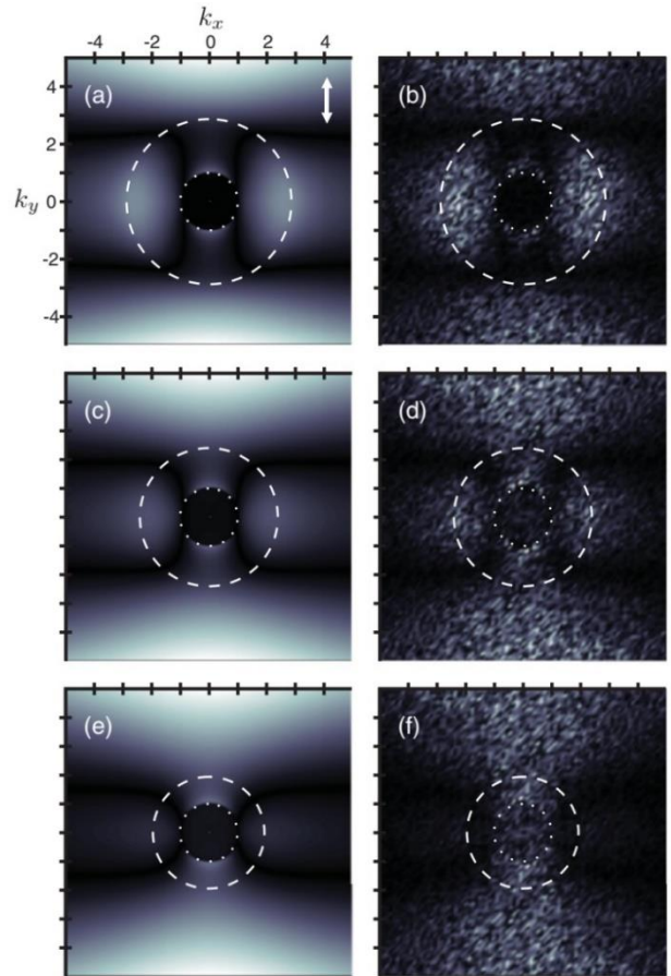
Figure 24 (Taken from ref. 95 ) \eta and FDTD- \eta maps For panels (a) and (b), N_e = 2 \times 10^{27} \text{ m}^{-3} , N_i = 26794 , \tilde{n}^* = 2.868 + 0.382i . For panels (c) and (d), N_e = 3 \times 10^{27} \text{ m}^{-3} , N_i = 13436 , and \tilde{n}^* = 2.401 + 0.679i . For panels (e) and (f), N_e = 4 \times 10^{27} \text{ m}^{-3} , N_i = 13421 , and \tilde{n}^* = 1.943 + 1.116i . The polarization direction is indicated by the white arrow in (a). The dotted and dashed circles represent \|k\| = 1 and \|k\| = \text{Re}(\tilde{n}^*) , respectively. A linear grayscale colourmap is used, the brightest areas have the largest values.
