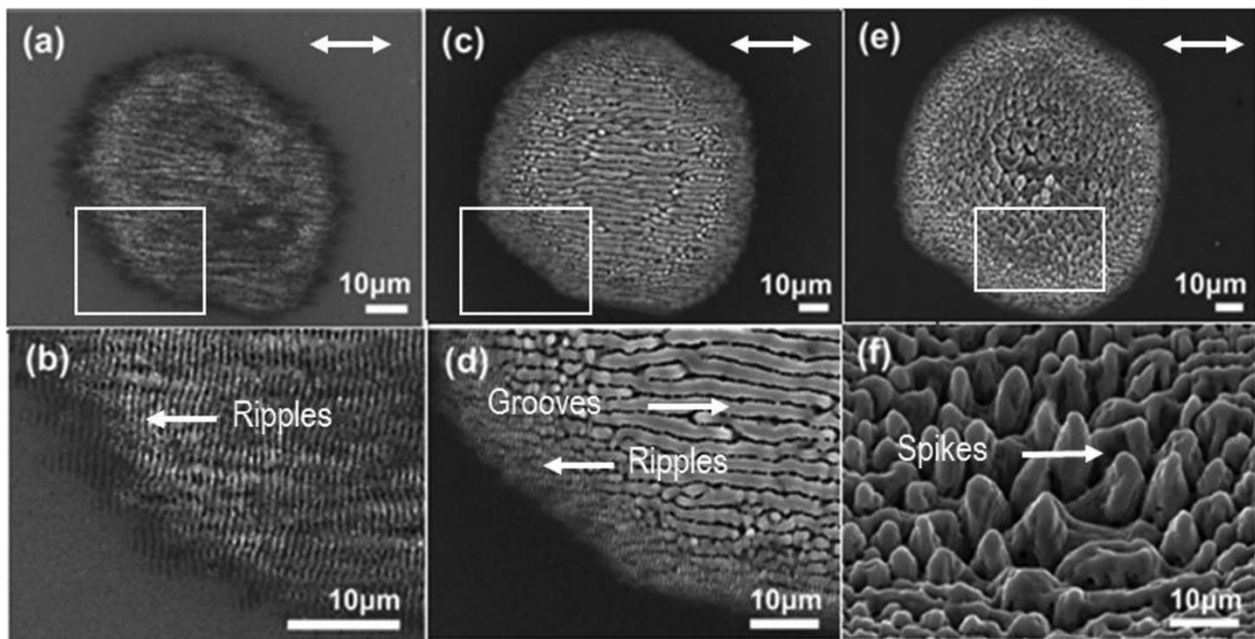
Figure 34 (Taken from ref. 46 ) SEM of silicon surface after irradiation with \lambda = 800 nm, \tau_p=430 fs, \Phi = 0.7 J/cm 2 . Ripples are formed for N = 10 (a & b), grooves for N = 40 (c & d), and spikes for N = 100 (e & f). Double-ended arrows indicate the laser beam polarization.
