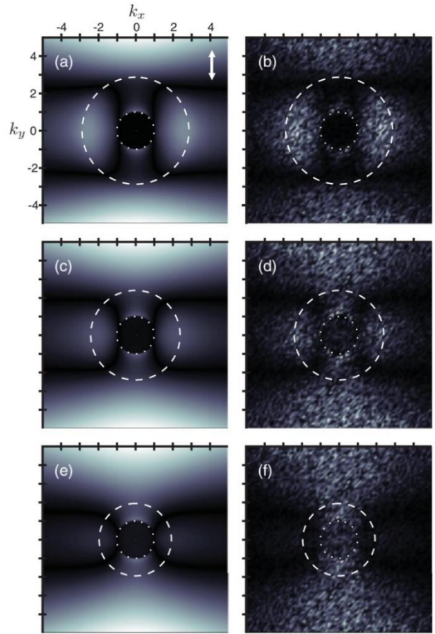
Figure 24 (Taken from ref. 95 ) \eta and FDTD- \eta maps For panels (a) and (b), N_e = 2 \times 10^{27} \text{ m}^{-3} , N_i = 26794 , \tilde{n}^* = 2.868 + 0.382i . For panels (c) and (d), N_e = 3 \times 10^{27} \text{ m}^{-3} , N_i = 13436 , and \tilde{n}^* = 2.401 + 0.679i . For panels (e) and (f), N_e = 4 \times 10^{27} \text{ m}^{-3} , N_i = 13421 , and \tilde{n}^* = 1.943 + 1.116i . The polarization direction is indicated by the white arrow in (a). The dotted and dashed circles represent \|k\| = 1 and \|k\| = \text{Re}(\tilde{n}^*) , respectively. A linear grayscale colourmap is used, the brightest areas have the largest values.
