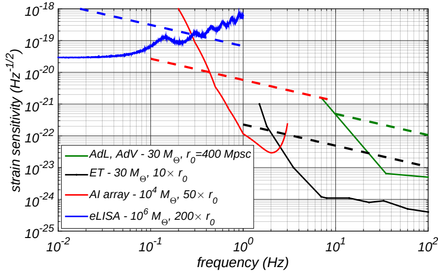
Figure 5.4: From [119]. Strain sensitivity curves of current and possible future GW detectors (plain lines). Dashed lines indicate the required sensitivity to detect the GW from a compact binary following Eq. (5.26); M_{\odot} is the mass of the sun and r_0 = 400 \text{ Mpc} . We assumed a detection with a signal to noise ratio of 1. AdV: Advanced VIRGO [121], AdL: Advanced LIGO [120]; ET (Einstein Telescope) [131]. eLISA [132] is a space-based laser interferometer proposal. The AI array is the proposal [70].
