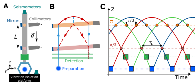
Fig. 1. Principle of the experiment. (A) Sketch of the experiment, where the atoms are laser cooled (blue cloud) and launched vertically, interrogated by two Raman beams (brought from the gray collimators and retroreflected on the blue mirrors), and detected on their way down (green box). The distance between the Raman beams is L = \frac{3}{8} gT^2 \approx 59 cm. (B) Diagram of the atom interferometer in the (xz) plane (not to scale), with the blue and red lines labeling the |\vec{0}\rangle and \hbar\vec{k}_{\text{eff}} momentum states, respectively. The dashed and plain lines show the two paths of the matter waves in the interferometer, which enclose an area of 11 \text{ cm}^2 . (C) Trajectories of the successively launched atom clouds in interleaved operation. Each interferometer has an interrogation time 2T = 801 ms, and the cycle time is T_c = 2T/3 = 267 ms. The \pi/2 pulses are shared between the atom clouds entering and exiting the interferometer.
