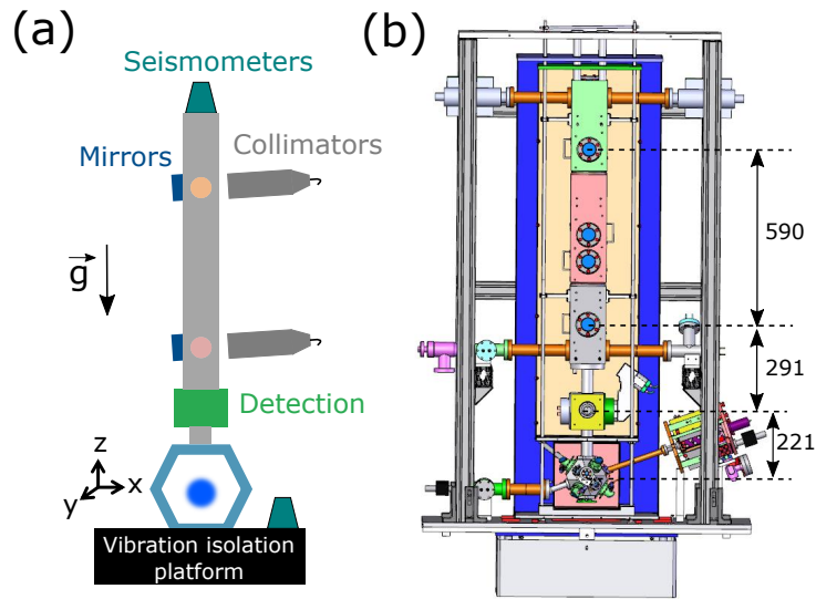
Figure 3.1: (a) Skematic view of the gyroscope-accelerometer experimental setup. The atoms are laser cooled (blue cloud) and launched vertically, interrogated by two Raman beams (brought from the gray collimators and retro-reflected on the blue mirrors), and detected on their way down (green box). The distance between the Raman beams is \frac{3}{8}gT^2 \simeq 59 cm for the maximally achievable interrogation time 2T = 0.8 s. Seismometers are used to record the vibrations of the setup. (b) Mechanical drawing (dimensions in mm).
