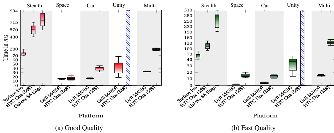
Figure 4.5: CPU-time required to generate one frame on the standalone and wearable devices
