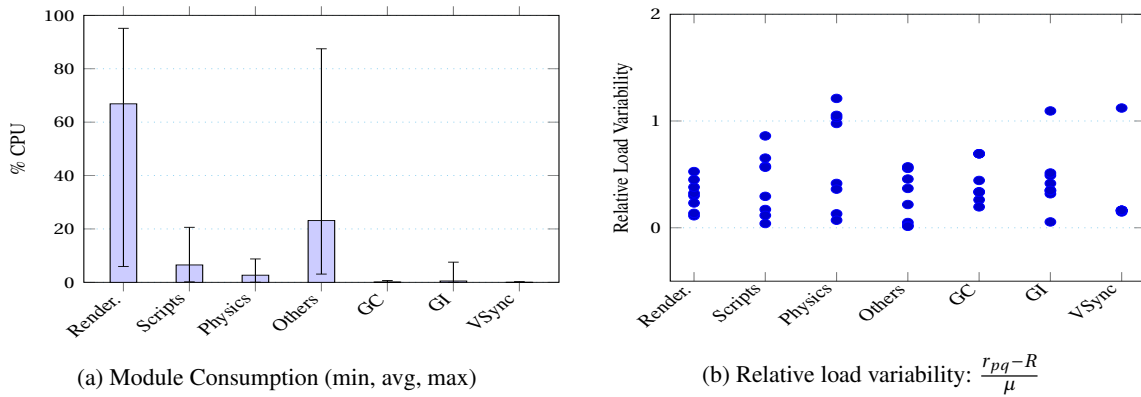
Figure 4.7: Module resource requirement and relative load variability
