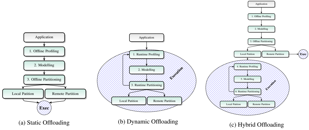
Figure 2.2: Time-based approaches for allocation decision
