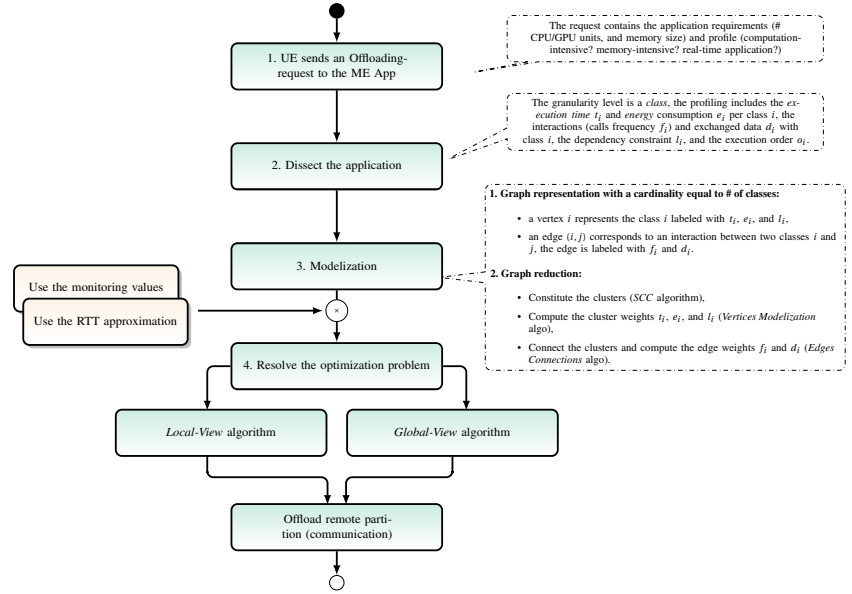
Figure 6.10: UE flowchart
