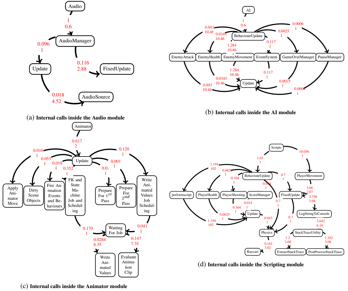
Figure 4.11: Internal flow concerning the main modules: Audio, AI, Animations, and Scripting
