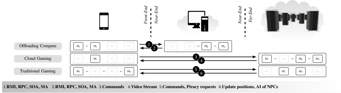
Figure 4.1: Comparison of gaming architectures
