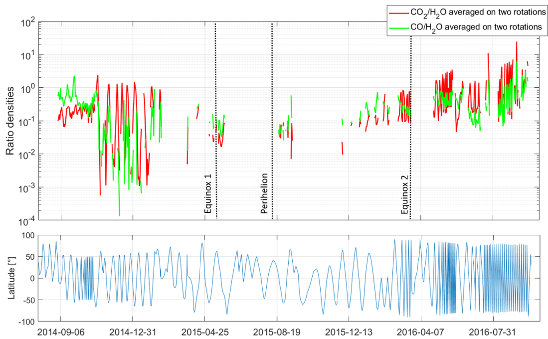
Figure 7.14: Upper panel: time evolution of CO/H 2 O and CO 2 /H 2 O average density ratios for the entire mission, starting in September 2014 and ending in September 2016. Lower panel: variation of the sub-spacecraft point's latitude in degrees.
