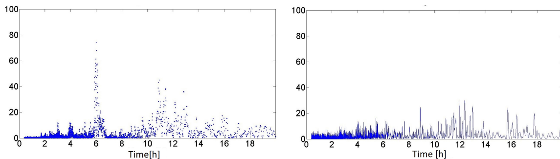
Figure 7.3: Lomb-scargle periodogram of \text{H}_2\text{O} (left), with strong periodicities at 6 and 12 hours, and of \text{CO}_2 (right), with a more homogeneous behaviour and a main periodicity of 12 hours.
