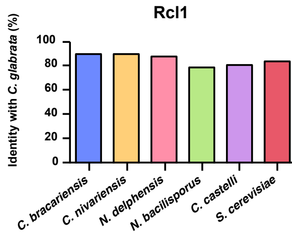
Figure 4.12. Rcl1 protein sequence identity between C. glabrata , Nakaseomyces species and S. cerevisiae . Pairwise alignments of Rcl1 protein sequence between S. cerevisiae , Nakaseomyces species and C. glabrata were performed with T-COFFEE software (Notredame et al. 2000). Identity rates were extracted from the 6 pairwise alignments and represented as bar charts.
