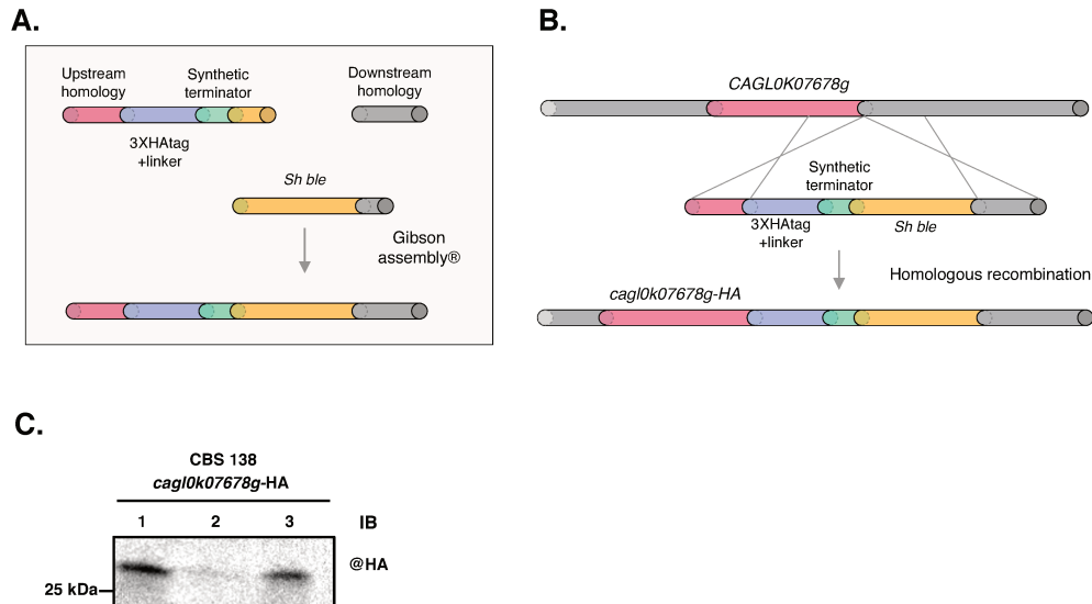
Figure 5.5. Tagging of the CAGL0K07678g protein by a 3X-HA epitope in a CBS138 strain. (A) The integrative cassette Cagl0k07678g -HA is composed of left and right homology arms of respectively 255 bp and 274 bp; the 3X-HA tag downstream a neutral linker; the synthetic terminator from (Guo and Sherman 1996) and the Sh ble selectable marker conferring the resistance to Zeocin™. (B) The integrative cassette enabling the tagging of the Cagl0k07678g protein was transformed in the CBS138 reference strain, and inserted into the C-terminal domain by homologous recombination. (C) Expression of the cagl0K7678g -HA fusion protein. The three independent cagl0K7678g -HA mutants were grown in rich liquid medium at 30°C to exponential phase, cells were then pelleted and transferred in liquid nitrogen-starvation medium for 6h. After total protein extraction, the expression of the cagl0K7678g -HA protein was assayed by Western Blot using monoclonal @HA antibody. IB: Immune blotting.
