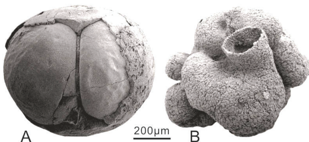
Fig. 6. Phosphatized micro fossils from the late Neoproterozoic Doushantuo Formation, Weng'an, Guizhou Province, south China. A. Assumed fossil animal embryo at two-cell stage. B. Earliest known sponge colony. Modified from Xiao et al., 1998; Yin et al., 2015.
