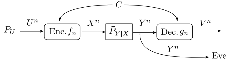
Figure 4.7: Wiretap channel: strong coordination implies secrecy.
