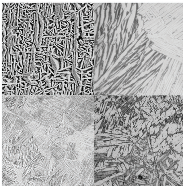
Widmanstätten Pattern at 40µm, 80µm, 400µm & 400µm [clockwise from top left]
