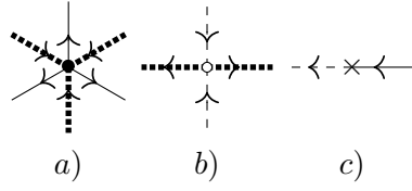
Figure 2.6: Colored vertices of a real trigonal graph.
