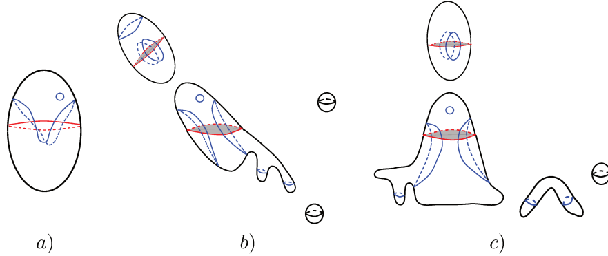
Figure 5.24: \mathbb{R}E in red.
