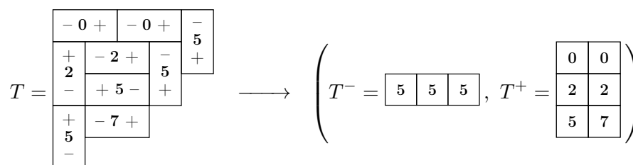
FIGURE 5.1: A semistandard domino tableau and its 2-quotient.
