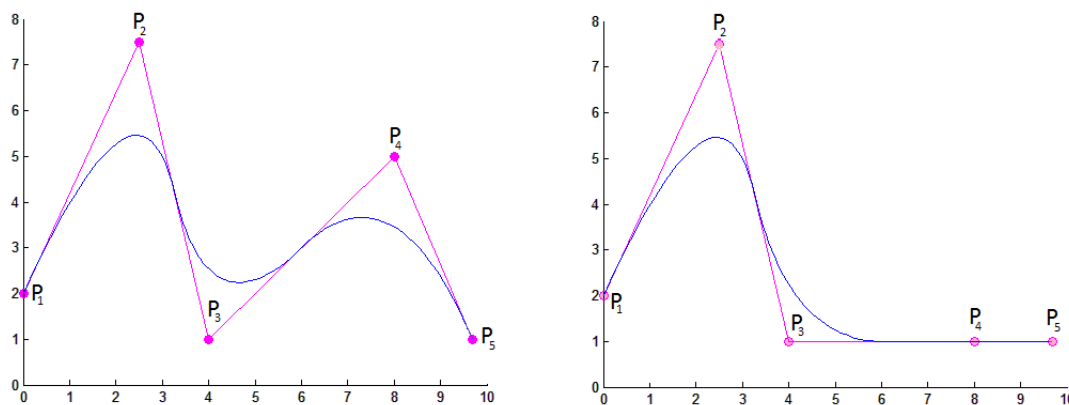
Figure 3.6: A quadratic B-spline curve and its control points. In the right, the curve after moving the control point P_4 .
