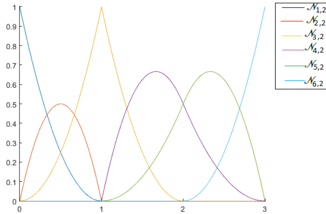
Figure 3.4: Quadratic basis functions with reduced continuity at \xi = 1 , \Xi = \{0, 0, 0, 1, 1, 2, 3, 3, 3\} .
