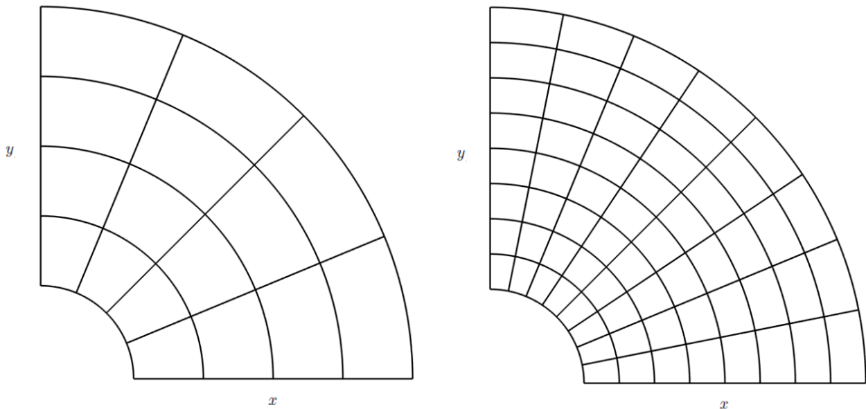
Figure 9.13: Curvilinear patches.
