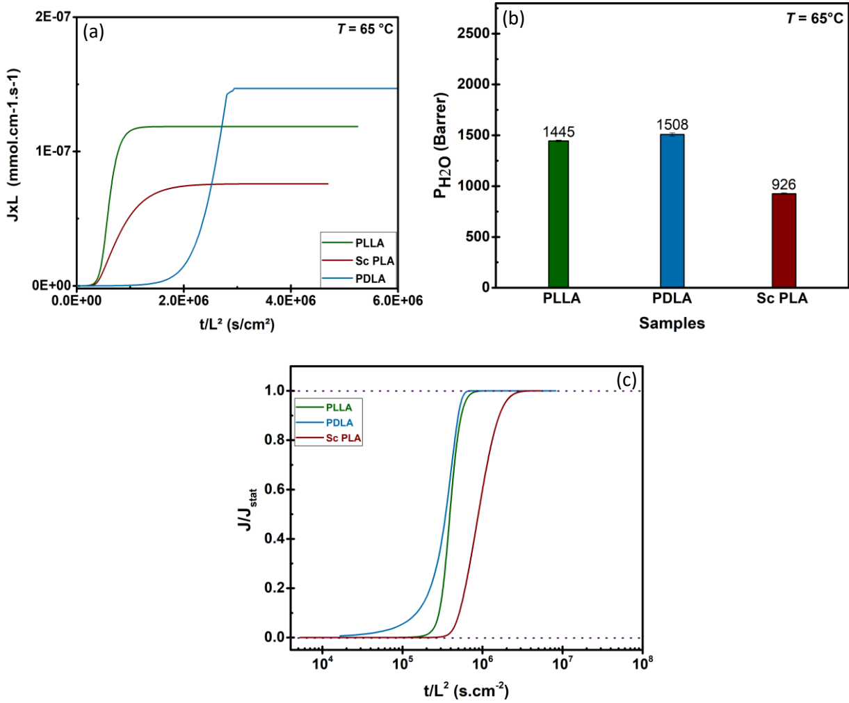
Figure 5. 8. (a) Evolution of the reduced flux of water permeation ( J^*L ) as a function of reduced time ( t^*L^2 ), (b) water permeability coefficient P , and (c) normalized water permeation curves as a function of the reduced time for semicrystalline PLLA, PDLA and sc PLA at T_{\text{permeation}} = 65^{\circ}\text{C} .
