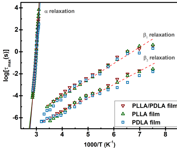
Figure 4. 13. Temperature dependence of structural \alpha and \beta relaxation times as a function of the inverse of temperature for amorphous PLLA, PDLA and sc PLA films.
