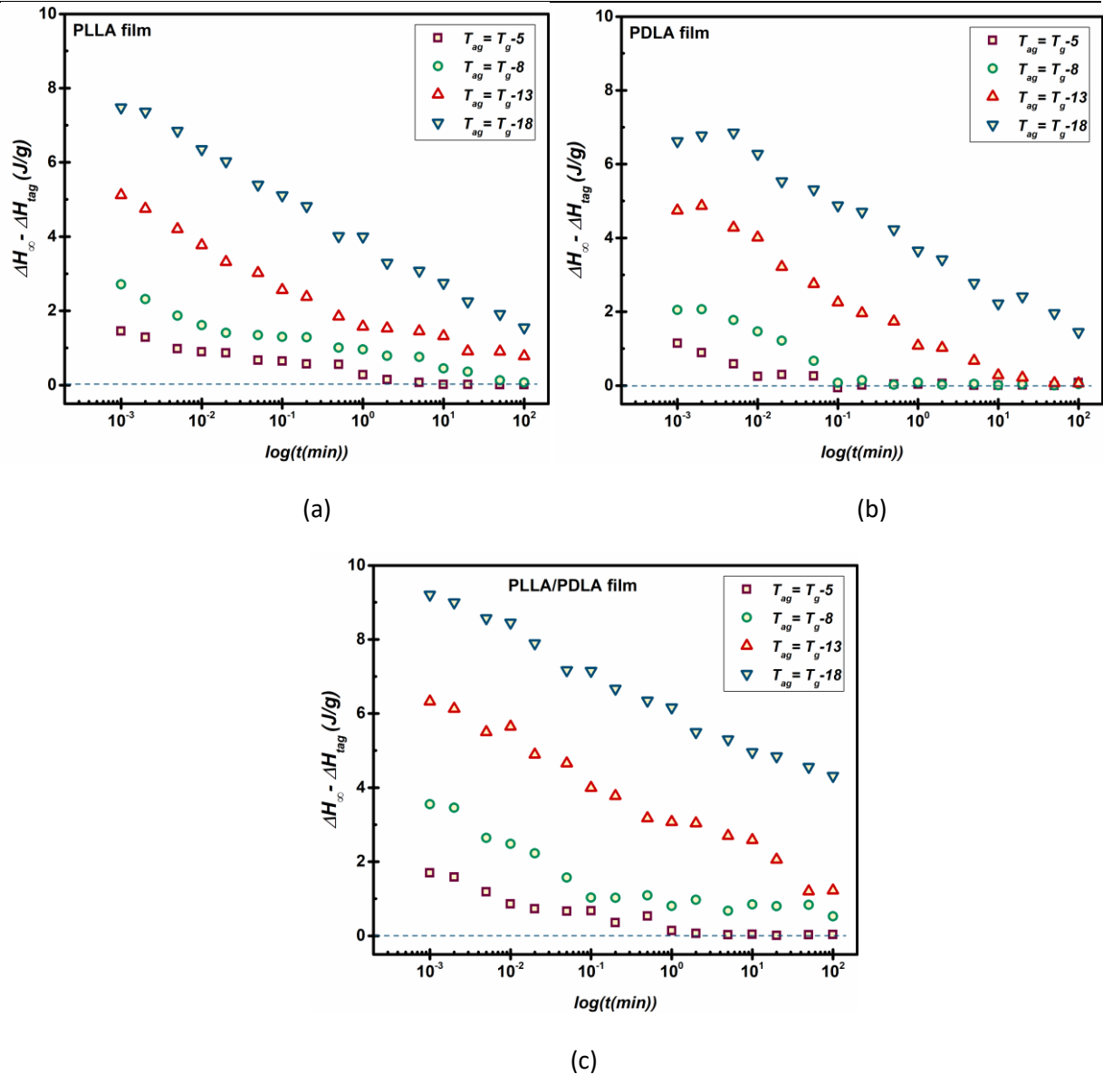
Figure 4. 6. Time evolution of the difference between the \Delta H_\infty and the \Delta H_{tag} for the aged amorphous (a) PLLA, (b) PDLA and (c) sc PLA as a function of T_{ag} with the aging time ranging from 0.001 min to 100 min at |\beta_c| = \beta_h = 1500 \text{ K}\cdot\text{s}^{-1} .
