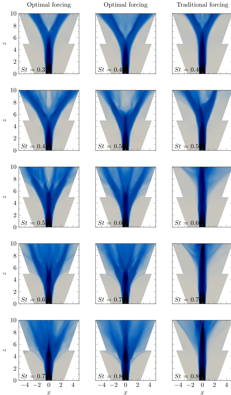
Figure 4.18: Mean axial velocity cuts in the bifurcating plane for various values of the Strouhal number in the range [0.35; 0.80] and for both optimal (left and middle columns) and ad-hoc (right column) forcings. The forcing amplitude is fixed for B and B' at 1% and the colour bar can be found in figure 4.17. The sponge layers are not displayed.
