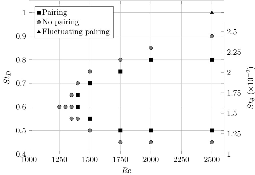
Figure 3.6: Occurrence of vortex pairing as a function of Reynolds number and Strouhal number for configurations with forcing amplitude A = 5\% and initial shear layer thickness \theta_0 = 0.025 . Only points near the pairing boundary are represented.
