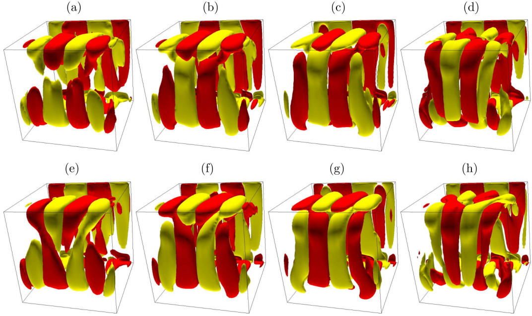
Figure 1.7: Successive helicity perturbation \mathcal{H} - \overline{\mathcal{H}} snapshots in one period of the time-periodic orbit observed in the cubical lid-driven cavity at Reynolds number 1930. The helicity is defined as \mathcal{H} = \mathbf{u} \cdot (\nabla \times \mathbf{u}) and is averaged over one period as \overline{\mathcal{H}} . From Lopez et al. (2017).
