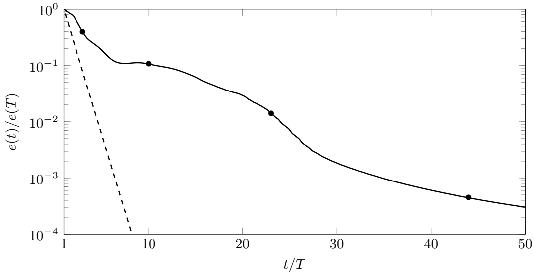
Figure 2.5: Evolution of the residual norm e(t) (equation (2.17)), in a jet simulation with Re = 2000 , St = 0.6 and \lambda = 0.04432 . Dashed line: decay rate found in the model problem. Markers indicate the instances of snapshots shown in figure 2.6.
