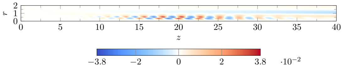
Figure 3.19: Vorticity field of the perturbation without any forcing applied at t = 40T .
