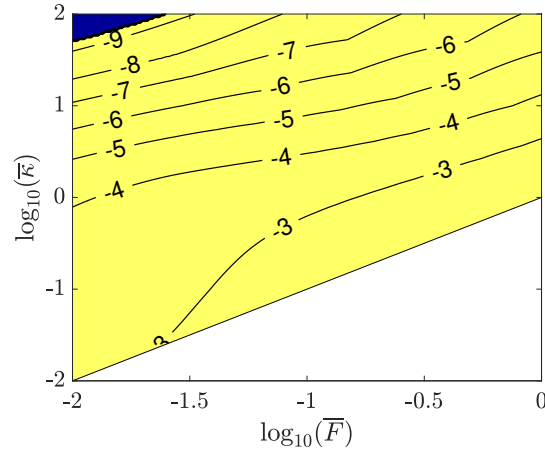
Figure A.5: Stability diagram for the deposition of GaAs(001), with \bar{v} = 0 , \Theta = 0.2 , S = 2 , \bar{\alpha} = 5 \times 10^{-6} . Blue and yellow correspond to the stable and unstable domains, and isolines display \max_{k \in (-\pi, \pi)} \log_{10} \mathcal{R}(\lambda) . The white area corresponds to a unphysical domain where the adatom density reaches values well above the equilibrium adatom coverage.
