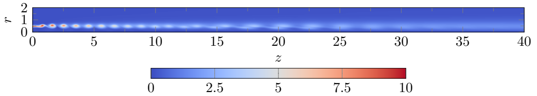
Figure 3.14: Vorticity snapshot of the base periodic unpaired flow at Re = 2000 and St_D = 0.6 slightly perturbed by the most unstable Floquet mode: \mathbf{u}' = \mathbf{U}^u + \epsilon \tilde{\mathbf{v}}_1 , with \epsilon = 0.2 .
