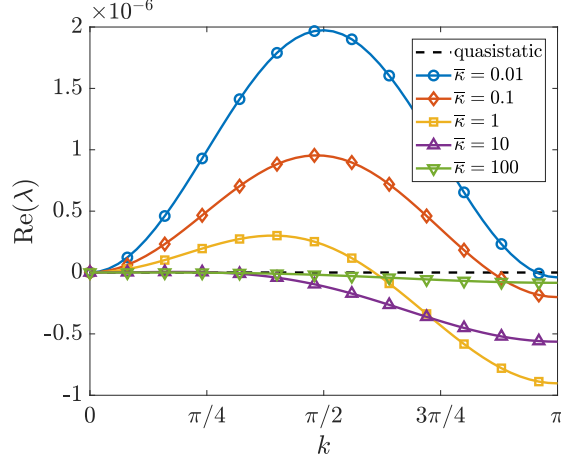
Figure A.2: Dispersion curves giving the critical growth rate \mathcal{R}(\lambda) as a function of the wavenumber k under pure deposition ( \bar{v} = 0 ), for \bar{F} = 10^{-2} and \Theta = 0.01 . The dotted line indicates neutral stability under the quasistatic approximation and the continuous lines show the stability results when the dynamics terms are included.
