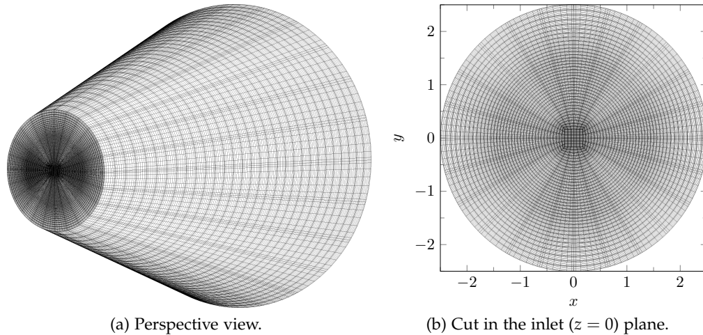
Figure 4.15: Mesh used for 3D nonlinear computation.
