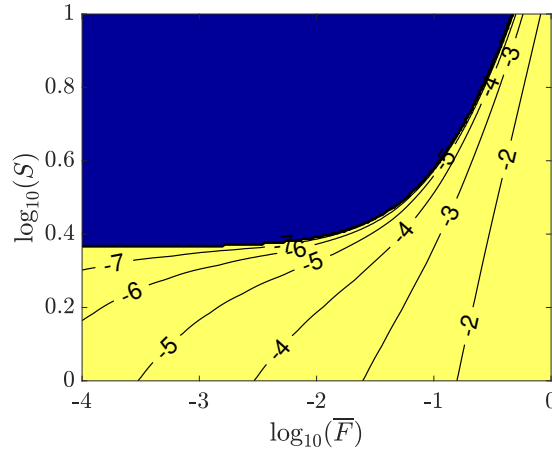
Figure A.3: Stability diagram under deposition ( \bar{v} = 0 ) in the presence of the ES effect and dynamics, with \bar{\kappa} = 10.1 and \Theta = 0.2 . The stable domain ( \max_{k \in (-\pi, \pi)} \mathcal{R}(\lambda) < 0 ) is shown in blue and the unstable region ( \max_{k \in (-\pi, \pi)} \mathcal{R}(\lambda) > 0 ) appears in yellow. In the latter, isolines display \max_{k \in (-\pi, \pi)} \log_{10} \mathcal{R}(\lambda) , indicating the magnitude of the most critical growth rate. For comparison, the diagram corresponding to the quasistatic approximation (i.e., with only the ES effect) is stable everywhere.
