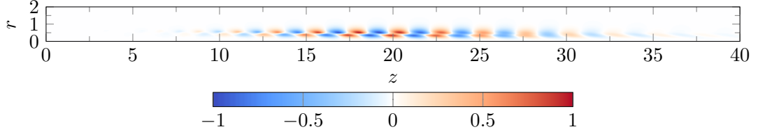
Figure 3.13: Vorticity component of the most unstable Floquet mode at Re = 2000 and St_D = 0.60 . It peaks far downstream.
