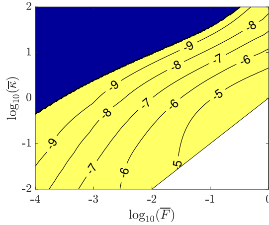
Figure A.4: Stability diagram for the deposition of Si(111)-7 \times 7, with \bar{v} = 0 , \Theta = 0.01 , S = 1 , \bar{\alpha} = 5 \times 10^{-5} . Blue and yellow correspond to the stable and unstable domains, respectively, and isolines display \max_{k \in (-\pi, \pi)} \log_{10} \mathcal{R}(\lambda) . The white area corresponds to a unphysical domain where the adatom density reaches values well above the equilibrium adatom coverage.
