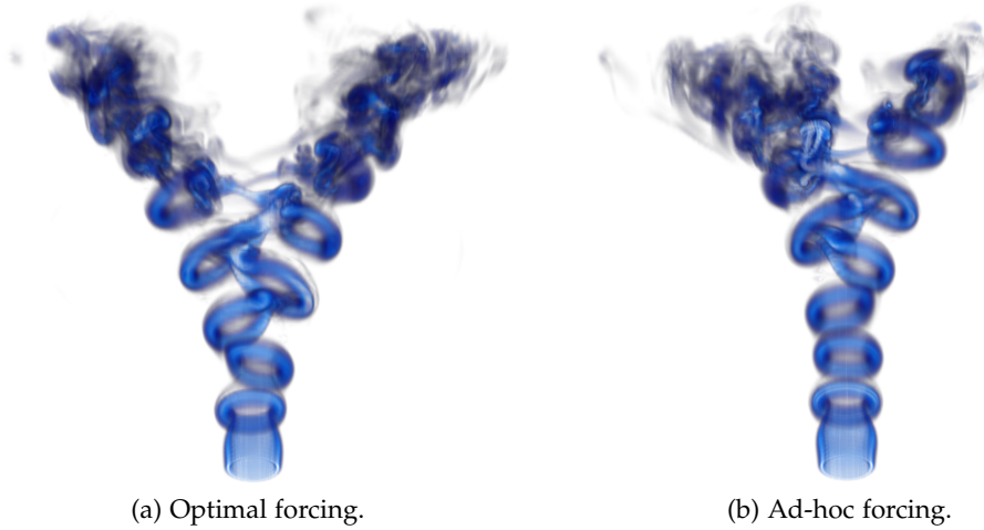
Figure 4.16: 3D vorticity magnitude snapshots of the nonlinearly forced bifurcating jet for Re = 2000 and St = 0.50 . On the left, the jet is forced optimally, whereas on the right, simple ad-hoc forcing is applied.
