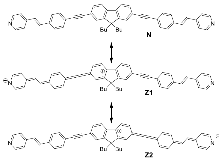
Figure 2.24 Resonance structures of 1 ; neutral one (N, top) and two zwitterionic ones (Z1 and Z2, below).
