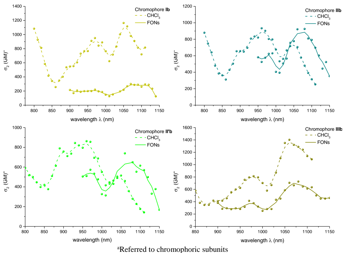
Figure 3.10 2PA spectra of chromophores in \text{CHCl}_3 (dotted line) solution and in aggregated state (solid line)
