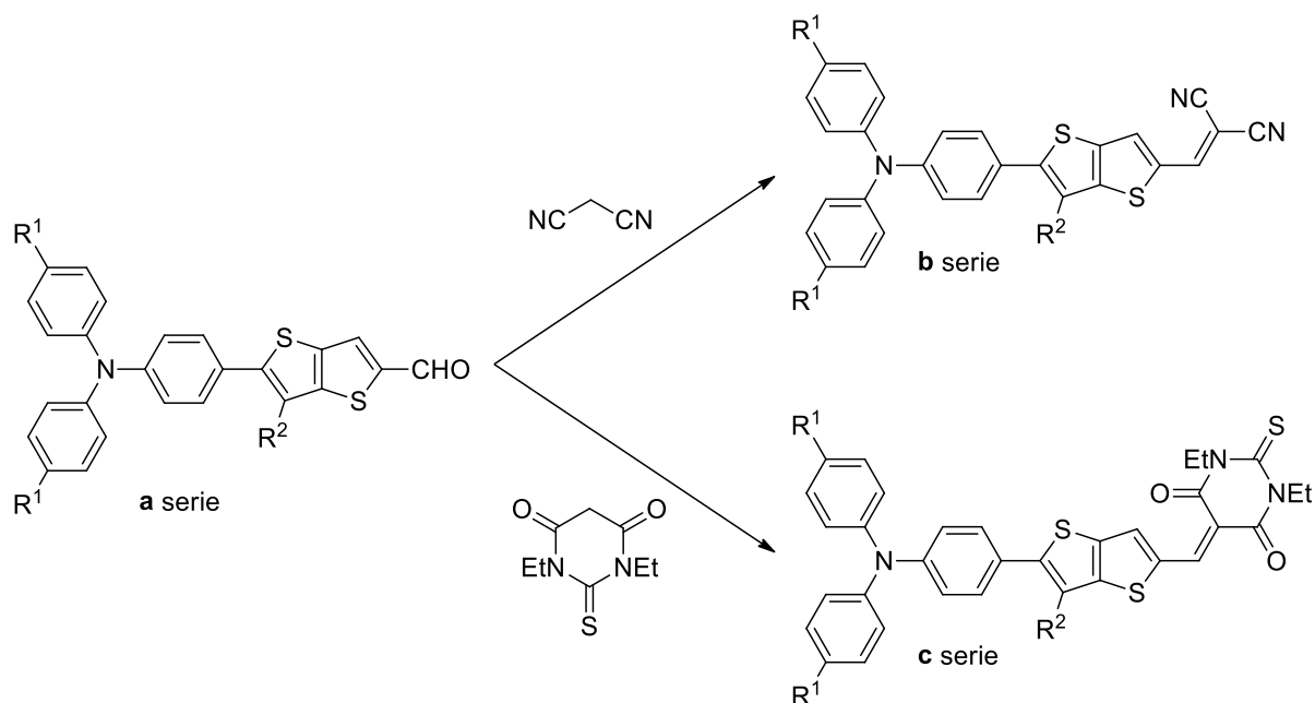
Scheme 3.7
