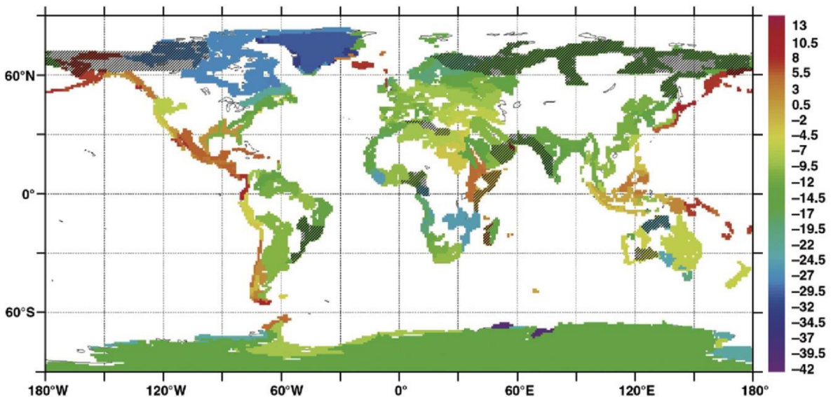
Figure 1.9 – Compilation of rock \epsilon_{Nd} with focus to the coastal areas. Figure from Jeandel et al. (2007)
