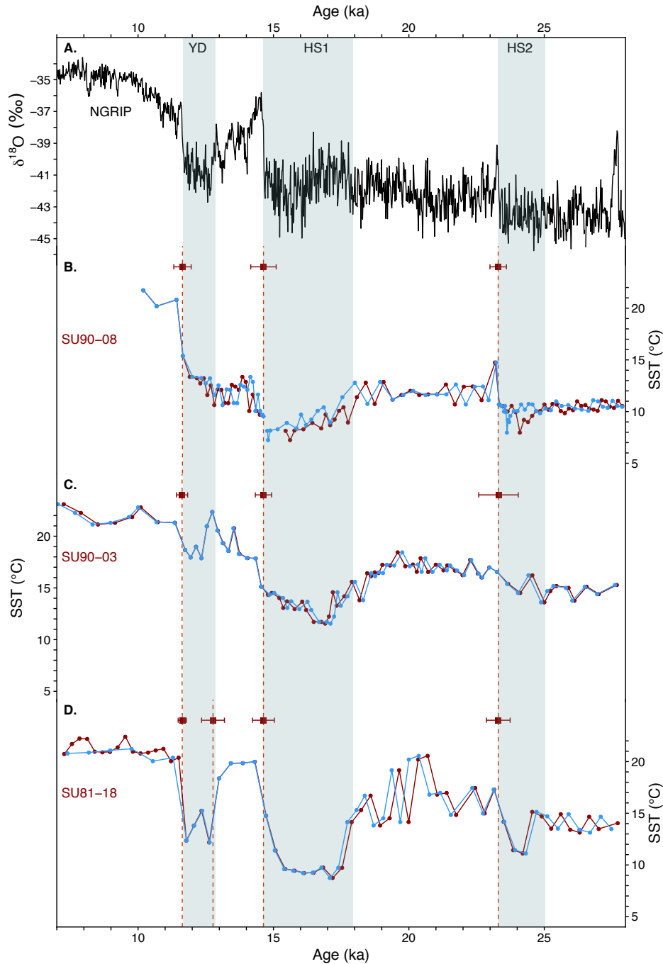
591 Figure 2: Impact of Th-normalization on the chronologies for SST reconstructions 592 A. \delta^{18}\text{O} of the ice at NGRIP [Andersen et al. , 2006; Rasmussen et al. , 2006; Svensson et al. , 593 2006; Vinther et al. , 2006], SST records (see Table 1) of core SU90-08 ( B ), SU90-03 ( C ), 594 SU81-18 ( D ). For each subplot, the red squares represent the alignment tie-points and 595 corresponding 1\sigma uncertainty (Tables S6 to S6), the red curve age scale is based on the 596 alignment tie-points, the blue curve age scale is based on Th-normalization between dated 597 levels. Grey bands represent the Younger Dryas, and Heinrich Stadial 1 and 2 chronozones.
