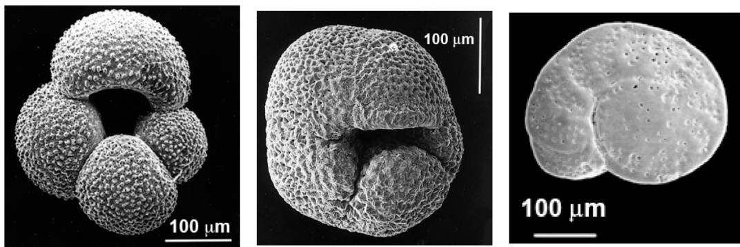
Figure 1.4 – Commonly used foraminifera species for paleoceanographic reconstructions.
