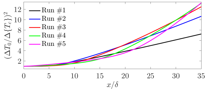
Figure 9.20: Downstream evolution of the temperature decay along the jet centerline using the classical adimensionalization for five different heated jets.
