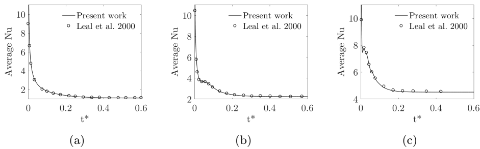
Figure 2.10: Comparison of average Nusselt number in the hot wall over time for (a) Ra = 10^3 , (b) Ra = 10^4 and (c) Ra = 10^5 .
