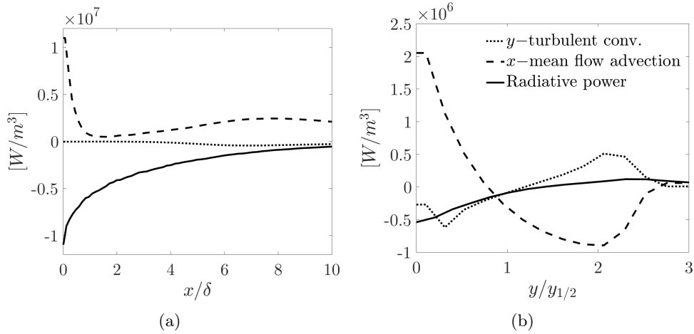
Figure 4.8: Enthalpy balance main components for the strongly heated jet at Re = 250 . (a) Downstream evolution and (b) cross-sections profile at x = 10\delta .
