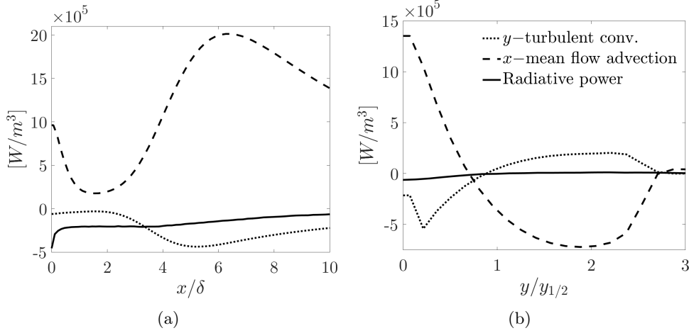
Figure 4.6: Enthalpy balance main components for the slightly heated jet at Re = 1500 . (a) Downstream evolution (b) and cross-section profile at x = 10\delta .
