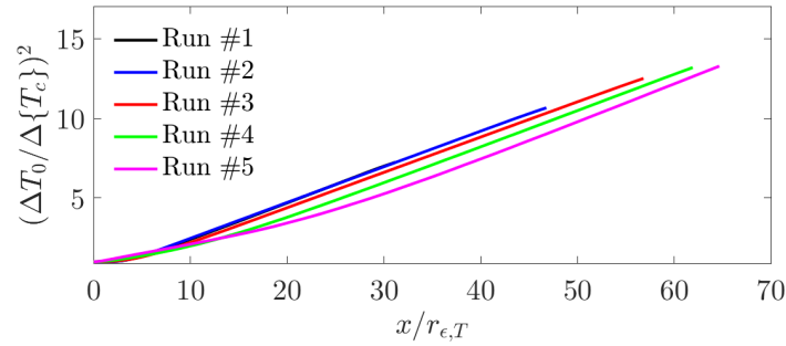
Figure 9.21: Downstream evolution of the temperature decay along the jet centerline using the adimensionalization of the equivalent heat jet opening based on the convective heat flux conservation for five different heated jets.
