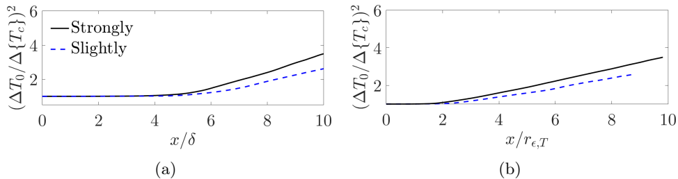
Figure 8.6: Downstream temperature decay along the jet centerline for the strongly and slightly heated jets using (a) classical scaling (b) scaling based on convective heat flux conservation.
