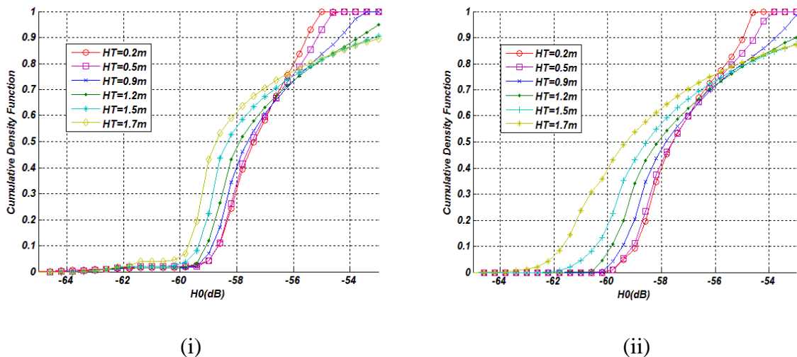
Figure 3.19. CDF(H_0) for scenario (b) as a function of H_T ; m=2 ; (i): \alpha=45^\circ ; (ii): \alpha=60^\circ
