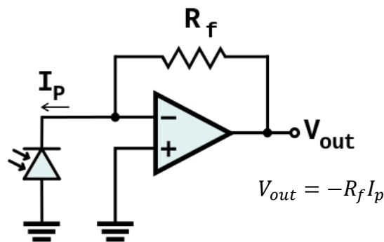
Figure 2.16. Basic scheme of TIA
