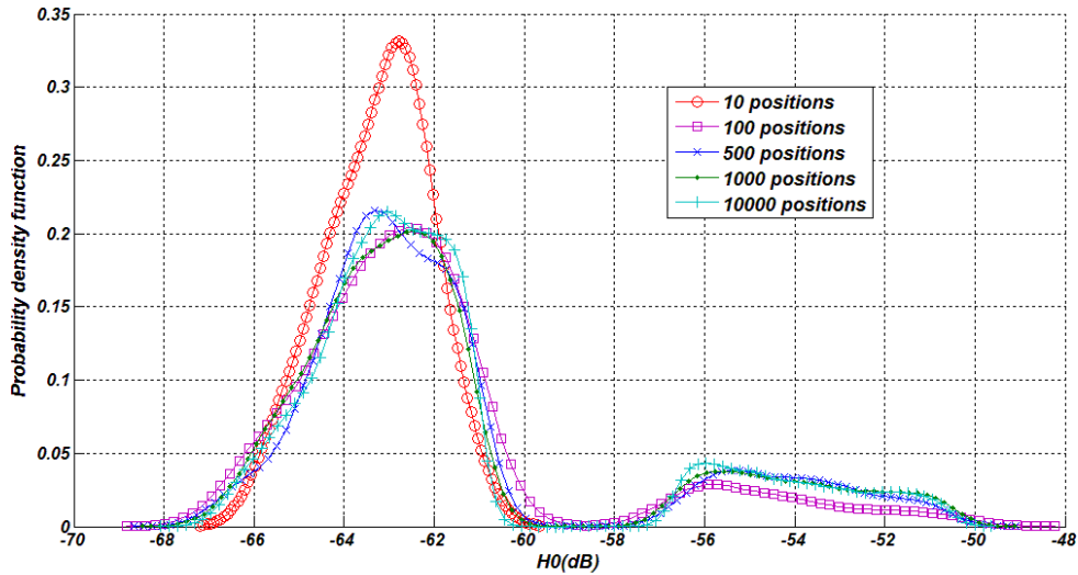
Figure 3.9. PDF(H_0) as a function of number of transmitter's position
