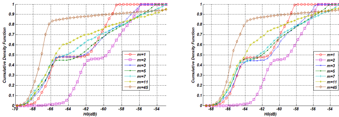
(a) \rho=0.1
