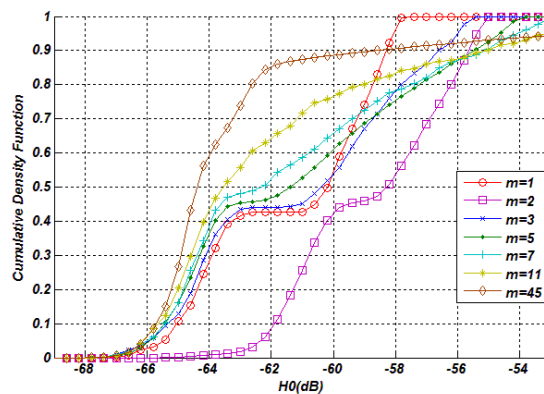
(c) \rho=0.9
