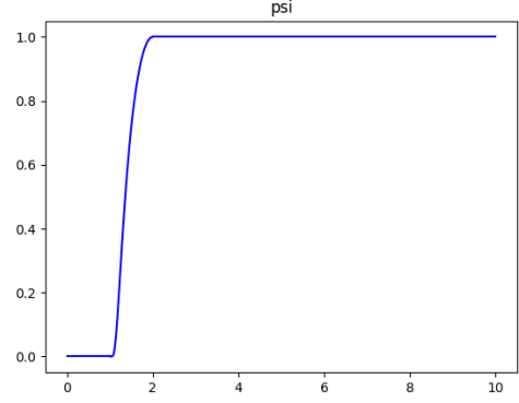
FIGURE F.2 – \psi
