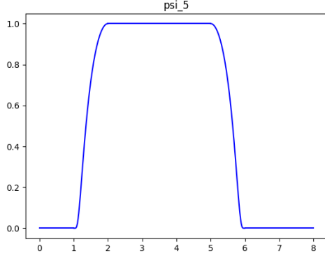
FIGURE F.1 – \psi_n for n = 5
