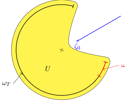
FIGURE G.1 – In yellow, an example of the domain U . The black circle arc is \omega_T (once we identify \mathbb{T} with the complex unit circle). The null-controllability of the parabolic-hyperbolic system implies that we can estimate the L^2(D(0, 1)) norm of complex polynomials by their L^\infty(U) norm. But if T is not too large, \omega_T is not the whole unit circle, and we can choose U such that D(0, 1) \not\subset U . Then, we can find a sequence of polynomials that converges to \zeta \mapsto (\zeta - \zeta_0)^{-1} away from the blue line.
