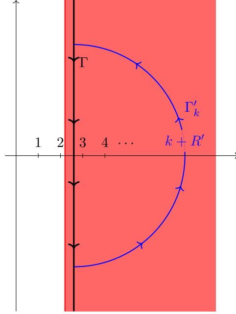
FIGURE G.2 – Path for the Residue theorem.
