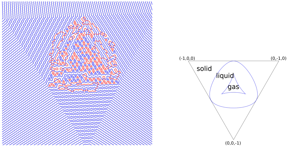
Figure 44: Left: a random taut loop configuration when |z| is large. Right: the algebraic limit shape, represented in the plane x + y + z = -1 , with the three expected phases of the model.
