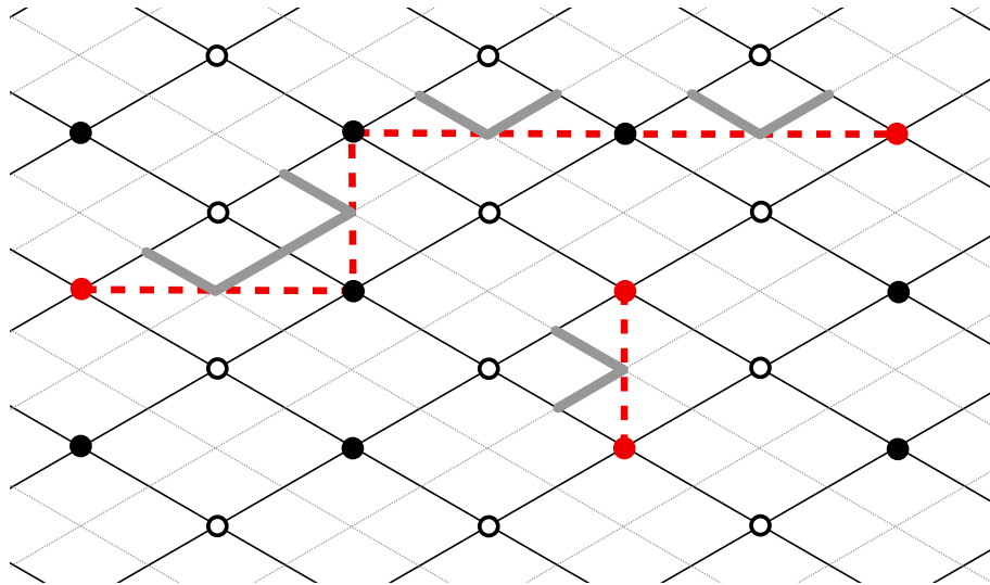
Figure II.6: A piece of a quadrangulation, a subset B_1 \subset \mathcal{B} with paths \gamma_{B_1} joining them pairwise (dashed), and a partial configuration (bold grey)
