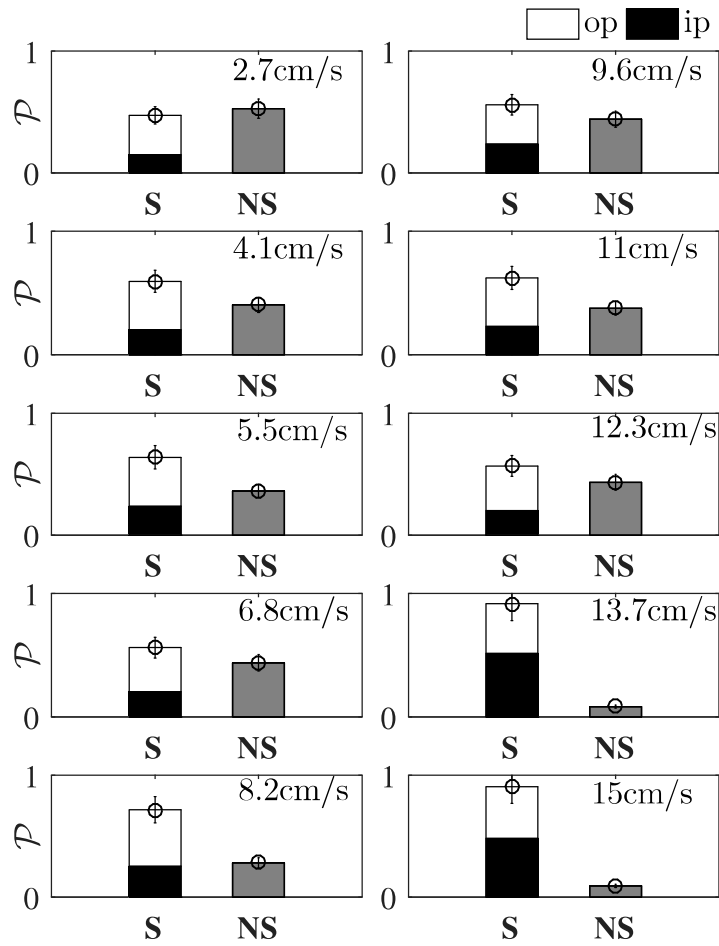
FIGURE A.2: Probability histograms of synchronization of fish pair 2 at different flow velocities: The mean body length of pair2 is 28 mm. The ratio of body length of two fish( L1/L2 ) is 1.10, where L1 is body length of top fish and L2 is body length of bottom.
