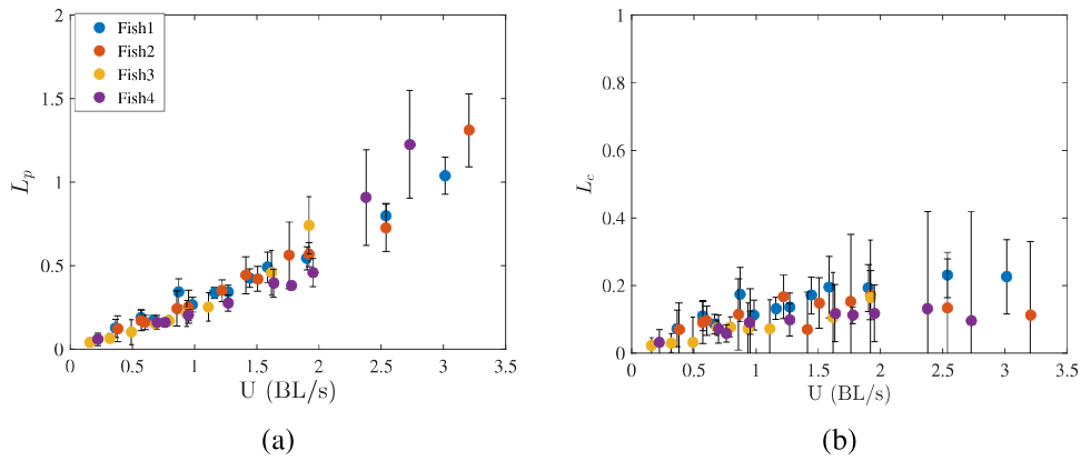
FIGURE 3.4: (a) Length scale L_p during burst period (b) Length scale L_c during coast period as a function of swimming velocity, U .
