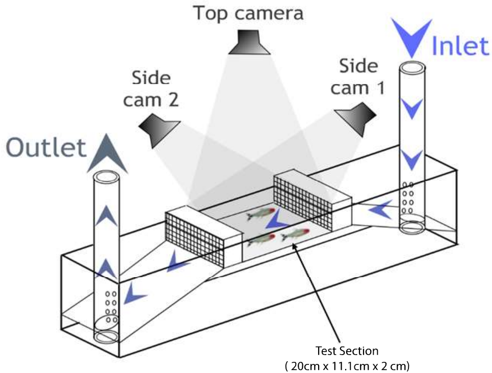
FIGURE 2.1: Schematic diagram of the swimming channel. An external pump drives the flow, which is directed toward the test section after a convergent ramp and through a honeycomb section to minimise swirling motions. The test section is covered from the top by using acrylic plate. The two side cameras and one top camera is installed to track the fish.
