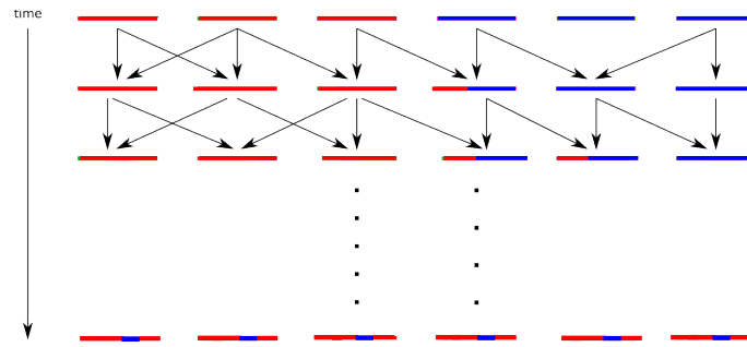
Figure II.1 – The Wright-Fisher model with recombination with two ancestral populations.
