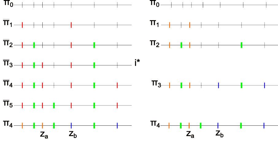
Figure I.5 – Example of two paths that go from \pi_0 to \pi_4 , for n = 7 . Loci in the same block are of the same color and the black loci corresponds to loci that are in singleton blocks. The path on the right corresponds p \in G(\pi_0 \rightarrow \pi_4, 4 + 2) and the path on the left is \tilde{p} \in G(\pi_0 \rightarrow \pi_4, 4) constructed from \pi with the method presented above.
