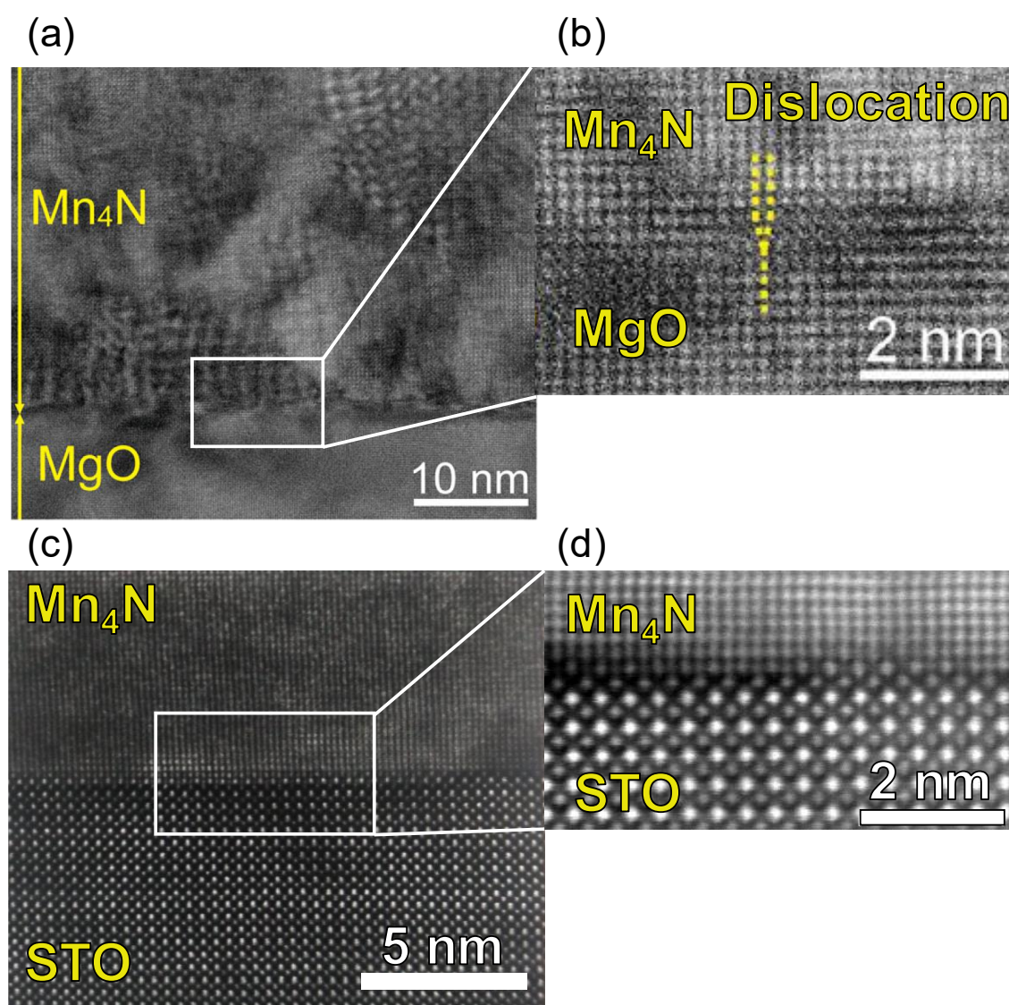
Figures A1: Cross-sectional TEM images of Mn 4 N thin films grown on (a), (b) MgO 114 and (c), (d) STO substrates. (b) and (d) are magnified views near the Mn 4 N/substrate interfaces. Yellow dashed lines in (b) denote a misfit dislocation.
