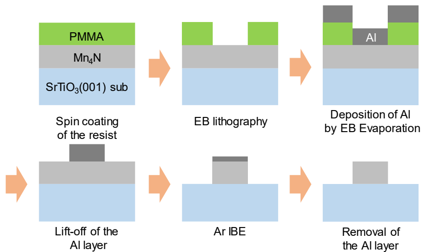
Figure 4-1: Fabrication process of Mn_4N into microstrips.
