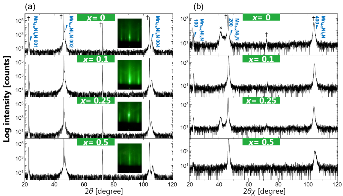
Figures 6-2: (a) Out-of-plane and (b) in-plane XRD spectra of Mn 4-x Ni x N thin films grown on STO. The scattering vector of in-plane XRD is along STO [100]. The marks of † and × denote the diffraction peaks from the substrate and from the oxidized phase (MnO), respectively. The in-plane diffraction peaks from Mn 4-x Ni x N are invisible, due to the overlapping with those of STO, which possess a close lattice constant. The insets are RHEED patterns, with the azimuth of electron beam along the STO [100] direction.
