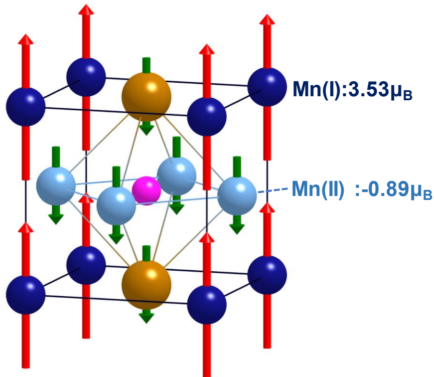
Figure 2-8: Crystalline structure and ferrimagnetic structure of \text{Mn}_4\text{N} .
