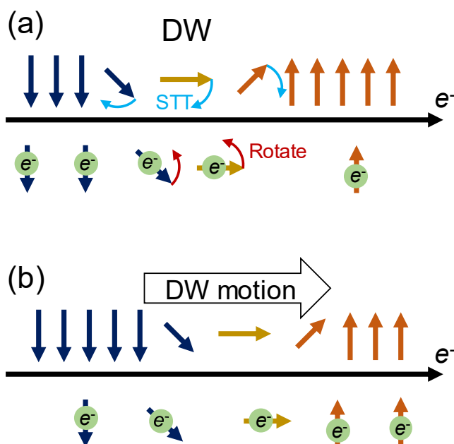
Figures 2-3: Schematic illustrations of CIDWM. Arrows denote magnetic moments. Electrons flows from left side to right side. (a) When electrons go through the DW, the spins rotate to be aligned along the localized magnetic moments. As a reaction, a STT acts on the localized moments. (b) As the STT acts on localized moments, the DW moves in the same direction as the electrons flow.
