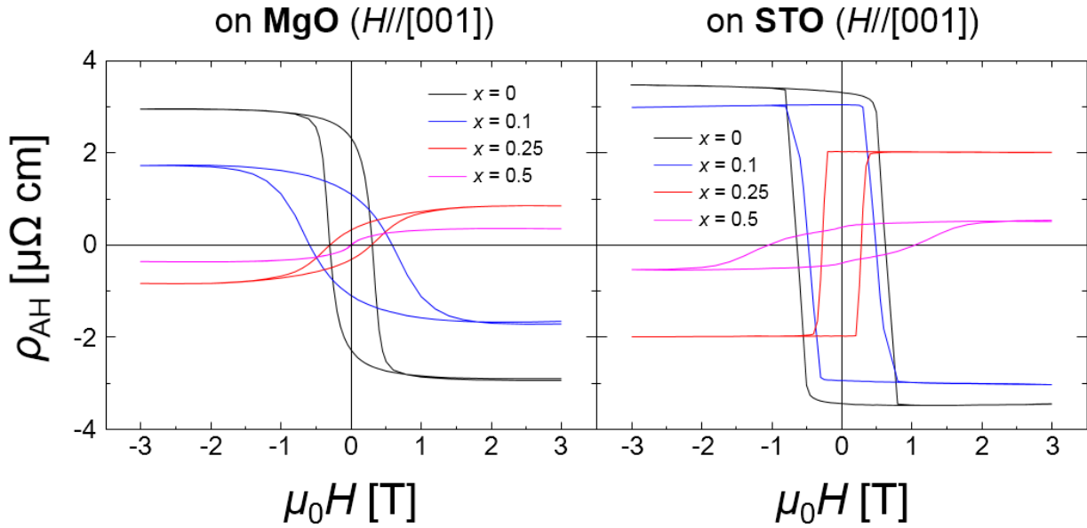
Figures 6-5: AHE hysteresis loops for out-of-plane fields of Mn 4-x Ni x N films deposited on (a) MgO and (b) STO substrates.
