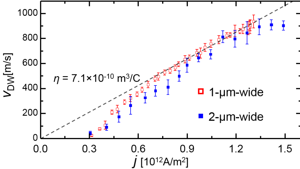
Figure 5-6: Current density dependence of DW velocity measured at room temperature. Both the 1 and 2- \mu m-wide strips possess similar behavior. The DW mobility has been derived from the linear fitting in the high j regime.
