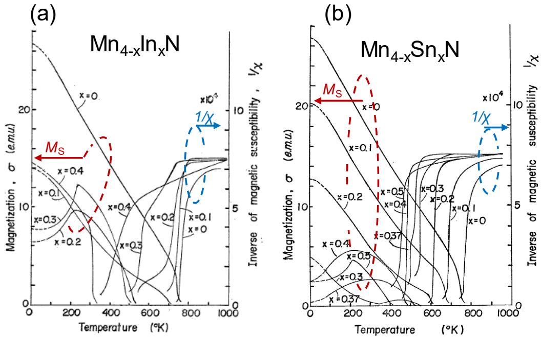
Figures 6-11: Temperature dependence of the magnetization ( T < T_N ) and of the susceptibility ( T > T_N ) in (a) Mn_{4-x}In_xN and (b) Mn_{4-x}Sn_xN powders 185 . The left (right) curves correspond to spontaneous magnetization M_S (inverted susceptibility 1/\chi ). Above compensation, M - T curves are bended in (a) x = 0.2, 0.3 and (b) x = 0.4, 0.5 .
