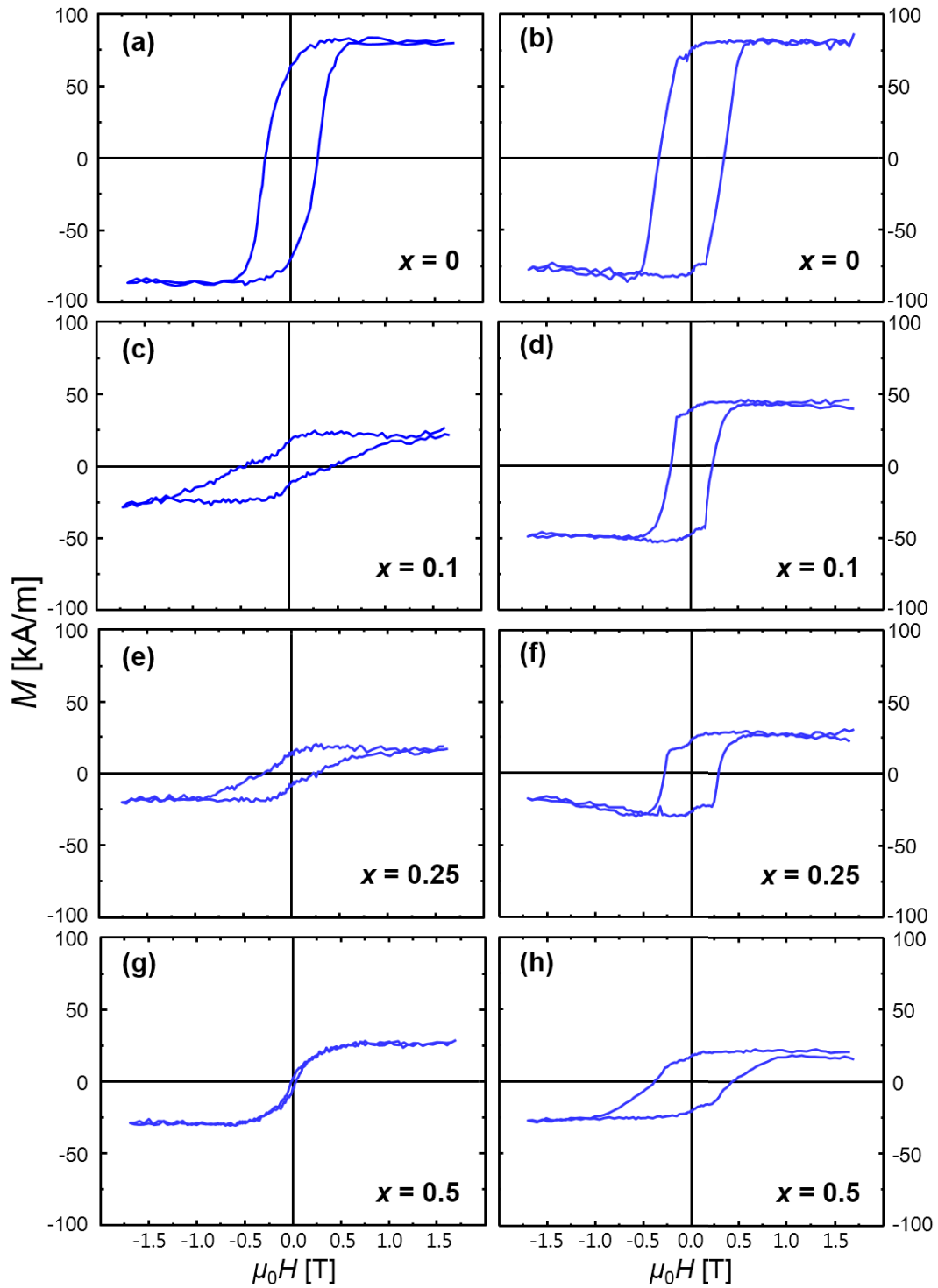
Figures 6-3: Out-of-plane M - H loops of Mn_{4-x}Ni_xN films grown on (a), (c), (e), (g) MgO and (b), (d), (f), (h) STO substrates.
