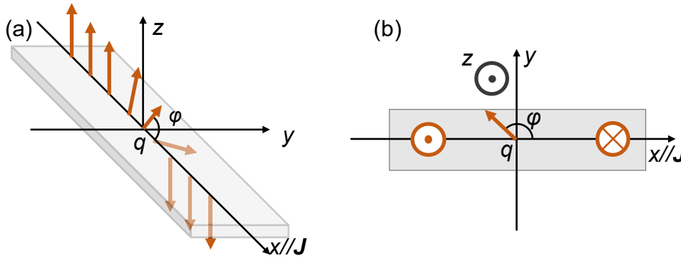
Figures 2-4: 1D model in magnetic strip. (a) Distribution of the magnetization in the vicinity of the DW. The orange arrows represent local magnetic moments. (b) Top view of (a). q and \varphi are the position of DW and the azimuth of magnetic moment in DW.
