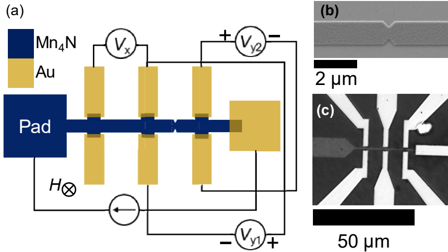
Figures 4-2: (a) Measurement geometry and Hall bar pattern consisting of a nucleation pad, 3 Hall crosses with Au electrodes and 1 notch to pin DW between 2 crosses. (b) SEM image of Al mask around the notch of 1- \mu\text{m} -wide strip after lift-off process. (c) Optical microscope image of the Hall bar.
