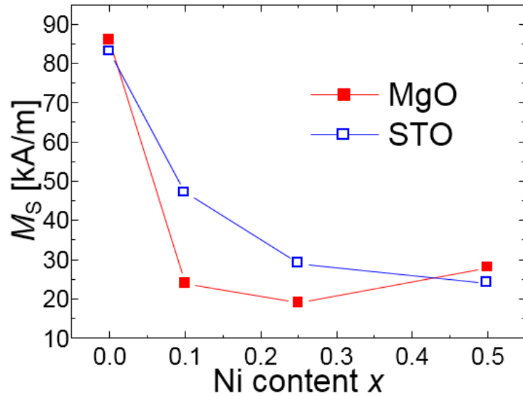
Figure 6-4: Dependence of the spontaneous magnetization with the Ni composition, for thin films deposited on MgO and STO.
