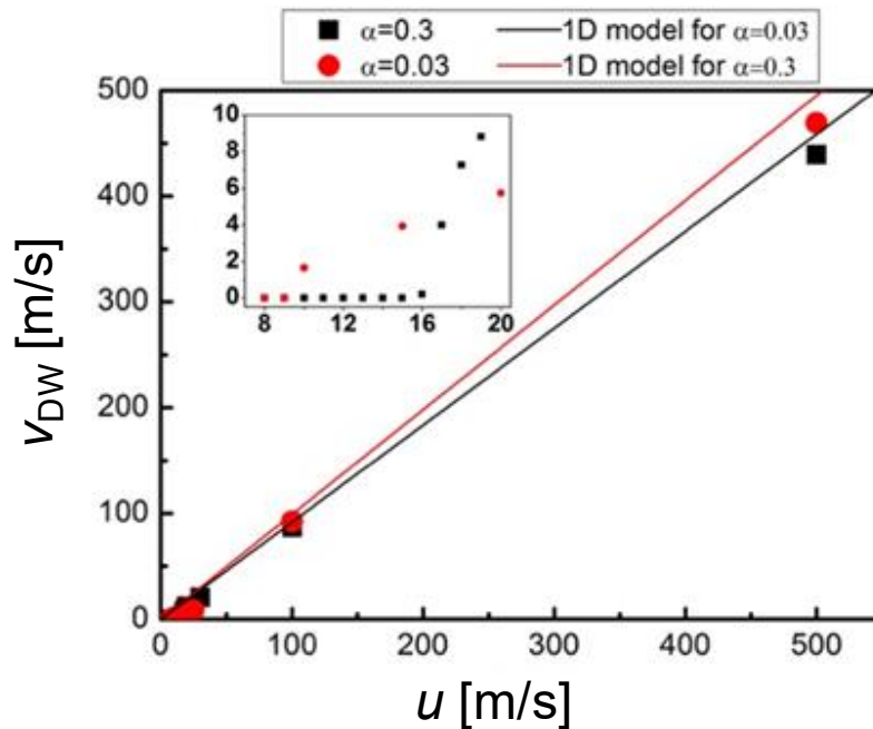
Figure 5-10: Results of micromagnetic simulations showing the DW velocity vs. spin-drift-velocity for two different values of \alpha : \alpha=0.03 (red circles), \alpha=0.3 (black squares). The solid lines represent the 1D model velocity. The inset presents the zoomed area around the critical current.
