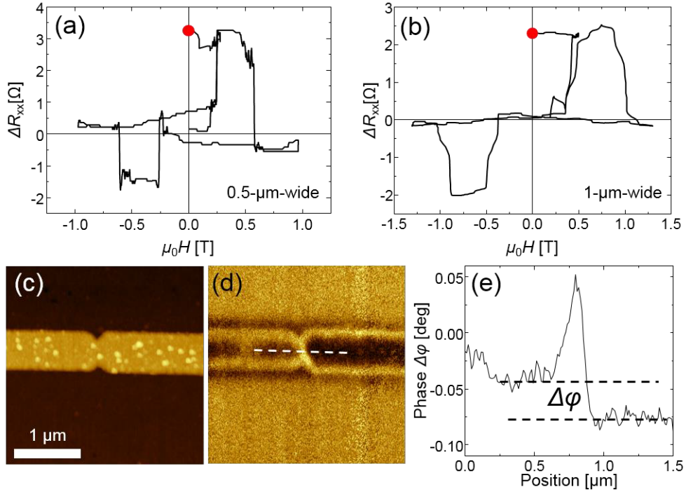
Figures 4-6: (a), (b) 4-probe resistance between the center and right Hall crosses as a function of the magnetic field, for (a) a 0.5- \mu\text{m} and (b) a 1- \mu\text{m} -wide device. The red dots indicate the end of the minor loop. (c) AFM and (d) MFM images of a 0.5- \mu\text{m} -wide strip after partial reversal. The phase difference \Delta\phi between the two sides of the constriction, shown in (e) suggest that a DW is indeed pinned at the notch.
