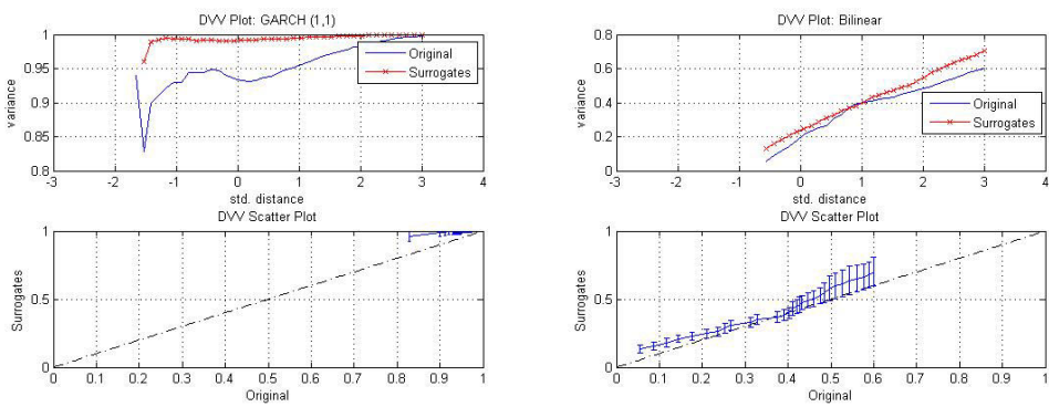
(a) DVV analysis on GARCH(1,1) signal
