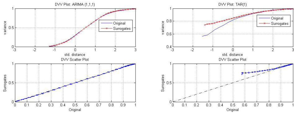
(a) DVV analysis on ARIMA(1,1,1) signal
