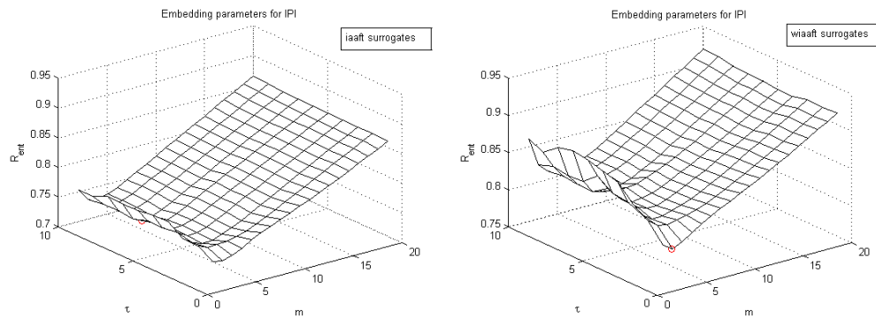
(a) Differential-Entropy based method with iAAFT surrogates. The optimal embedding values are m = 4 and \tau = 7 with entropy ratio , R_{ent}(m, \tau) = 0.7271 . (b) Differential-Entropy based method with wiAAFT surrogates. The optimal embedding values are m = 3 and \tau = 1 with entropy ratio , R_{ent}(m, \tau) = 0.7923 .
