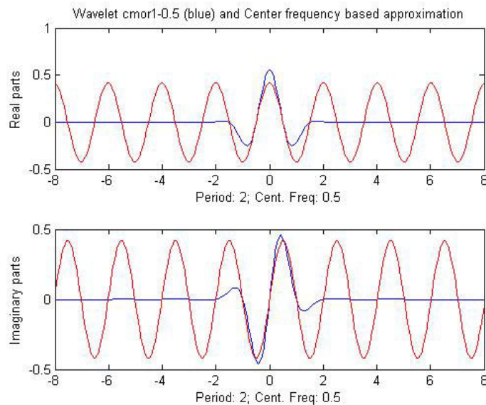
FIGURE 2.1: Complex Morlet wavelet with f_b = 1 and f_c = 0.5
