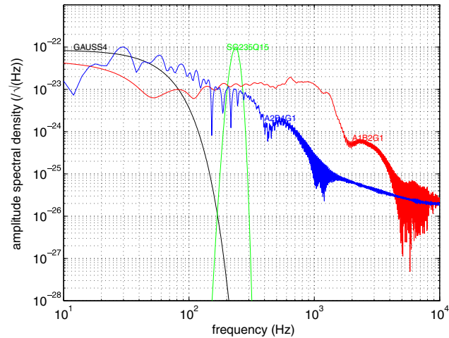
Figure 3. Spectrum of the waveform families of burst sources used in this study to estimate the performance of the different pipelines. DFM A1B2G1 and DFM A2B4G1: gravitational wave emitted during core collapse simulated by Dimmelmeier, Font and Mueller [4]. SG235Q15: sine-Gaussian signal. GAUSS4: Gaussian peak. All waveforms have been normalized such that h_{\text{ISS}} = 3.59 \times 10^{-22} \sqrt{\text{Hz}} . This value corresponds to a SN source located at 10 kpc emitting a A1B2G1 waveform.
