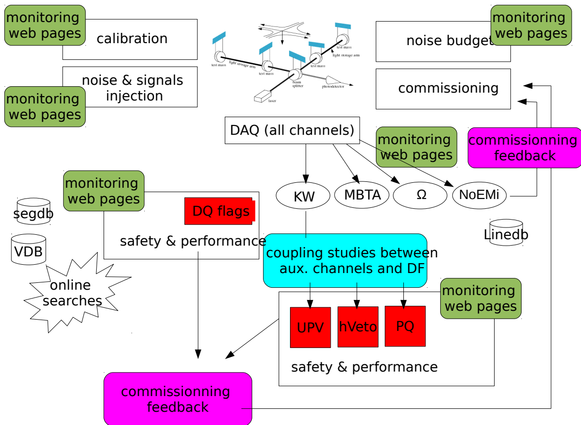
Figure 4.21: Virgo detector characterization elements. Each of them correspond to an activity or a piece of software that processes Virgo raw data. Most of the activities generate automatically web pages that are useful for commissioning and shifters.
