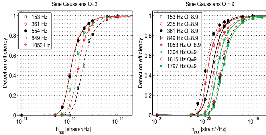
Figure 10. Detection efficiency of the search analysis as a function of the signal strength h_{rSS} at earth for Sine Gaussian waveforms with different central frequencies f_0 and for two different values of the Q_0 factor: left Q_0 = 3 , right Q_0 \sim 9 . The efficiencies were computed for sources at random sky locations. The error bars take into account only the statistical error on the detection efficiency.
