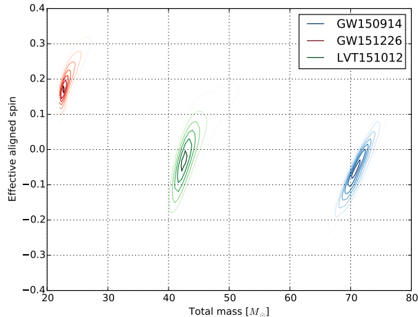
Figure 2.15: The effective spin of the inspiralling components of the three events GW150914, GW151226 and LVT151012 against their total mass [267].
