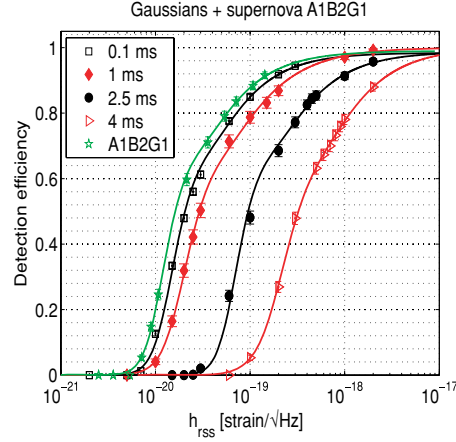
Figure 9. Detection efficiency of the search analysis as a function of the signal strength h_{r,SS} at earth for the Gaussian waveforms (with \tau specified in the legend) and one core collapse simulated waveform (A1B2G1). The efficiencies were computed for sources at random sky locations. The error bars take into account only the statistical error on the detection efficiency.
