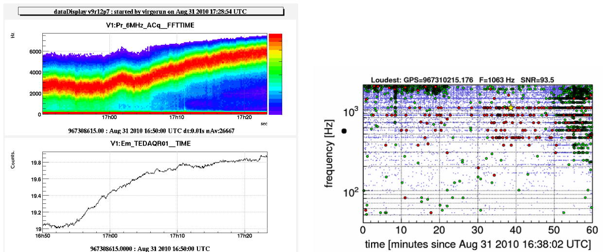
Figure 4.20: Left: Spectrogram of 30 minutes of data showing an excess of noise between 2 and 6 kHz that drifts over time following the data acquisition room temperature increase. The excess of loud glitches (SNR > 10 glitches in red) at high frequency (between 1 and 4 kHz) is visible on the right plot. The correlation between the glitch excess at high frequency and the temperature in the DAQ room has been observed but has never been understood.
