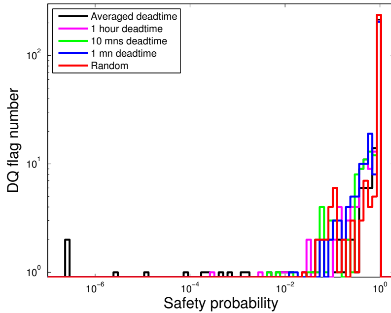
Figure 4.26: Comparison of the different safety probability estimations for all a priori safe vetoes defined during VSR2, VSR3 and VSR4 runs.
