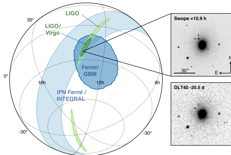
Figure 5.5: Skymap of GW170817 (green) and GRB170817A (blue). The LIGO only (light green) skymap 90% area is reduced from 190 deg 2 to 31 deg 2 when Virgo data are used. The inset shows the location of the apparent host galaxy NGC4993 seen by the Swope telescope 10.9 hours after GW170817 and an image of the same sky region taken by DLT40 20.5 days before.
