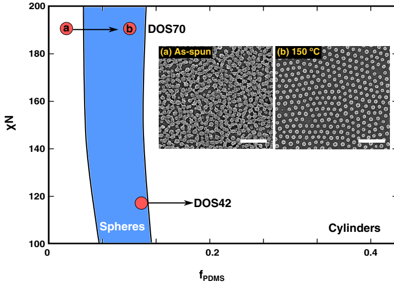
Figure 2.5.: Main image: BCP phase diagram in the high-segregation regime ( \chi N > 100 ). Morphology transition of the plasticized solution PS- b -PDMS 70 kg/-mol with DOS: Top-view SEM images of their (a) as-spun thin film and (b) after thermal annealing during 30 s at 150 °C. Scale bar corresponds to 200 nm.
