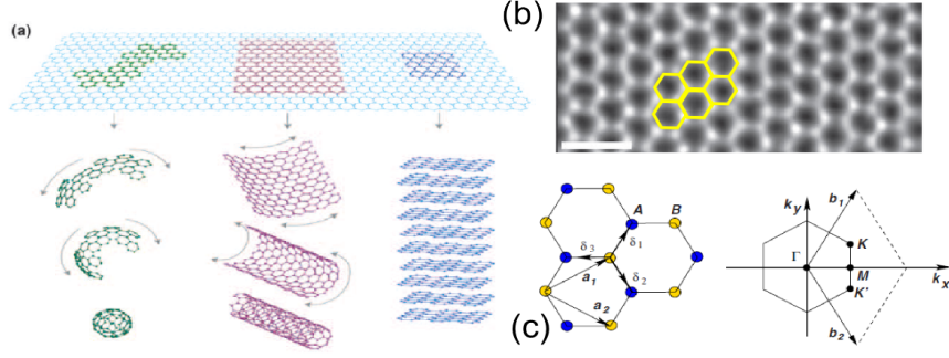
Figure 3.1.: (a) Schematic drawing of the relationship between graphene and other carbon materials. G is a 2D building material for carbon materials of all other dimensions. It can be wrapped up into 0D buckyballs, rolled into 1D nanotubes or stacked into 3D graphite [3]. (b) Lattice structure of G under TEM showing its hexagonal lattice [4]. (c) Lattice structure of G, made out of two interpenetrating triangular lattices ( \mathbf{a}_1 and \mathbf{a}_2 are the lattice unit vectors, and \sigma_i, i = 1, 2, 3 are the nearest-neighbor vectors), at the right the corresponding Brillouin zone. The Dirac cones are located at the \mathbf{K} and \mathbf{K}' points.
