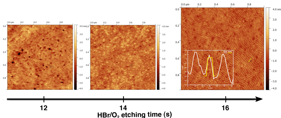
Figure 5.6.: Oxidation evolution in time of the PDMS features for (a) 12 s, (b) 14 s and (c) 16 s of HBr/O 2 plasma etching. The mask was stripped with the optimal conditions found in fig. 5.5, i.e., 10 s with HF 0.5 % v. Inset in image (c): AFM height profile of the yellow line.
